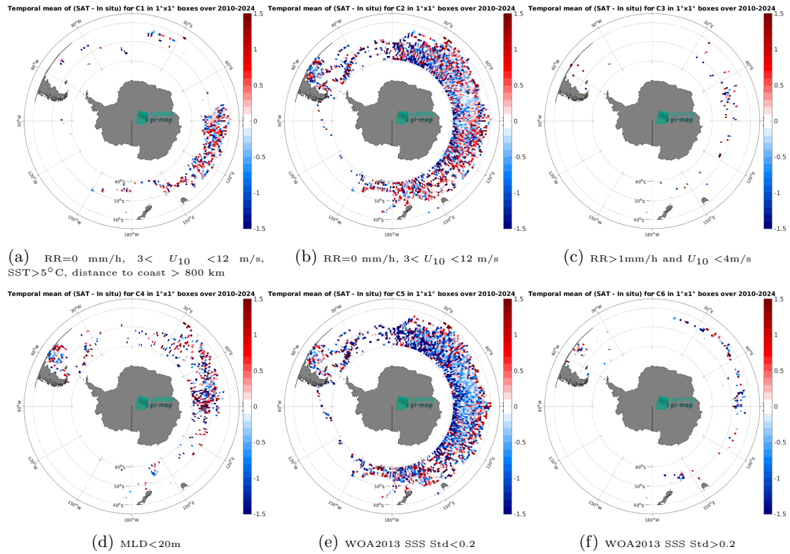
Figure 14: Temporal mean gridded over spatial boxes of size 1^\circ \times 1^\circ of \Delta SSS (SMOS SSS L2Q v331 - No FLAG (CMEMS-CATDS-CPDC) - Marine mammals) for 6 different subdatasets corresponding to:RR=0 mm/h, 3 < U_{10} < 12 m/s, SST>5°C, distance to coast > 800 km (a), RR=0 mm/h, 3 < U_{10} < 12 m/s (b), RR>1mm/h and U_{10} < 4 m/s (c),MLD<20m (d),WOA2013 SSS Std<0.2 (e),WOA2013 SSS Std>0.2 (f).
