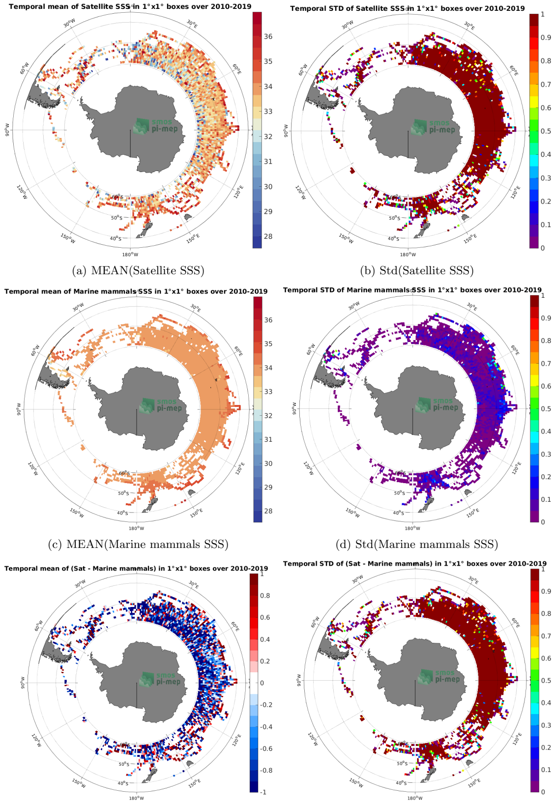
Figure 6: Temporal mean (left) and Std (right) of SSS from SMOS SSS L2Q v331 - No FLAG (CMEMS-CATDS-CPDC) (top), Marine mammals (middle), and of \Delta SSS (Satellite - Marine mammals). Only match-up pairs are used to generate these maps.
