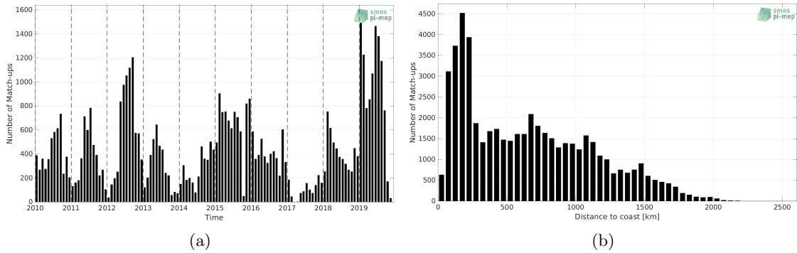
Figure 1: Number of match-ups between Marine mammals and SMOS SSS L2Q v331 - No FLAG (CMEMS-CATDS-CPDC) SSS as a function of time (a) and as function of the distance to coast (b) over the Roaring Forties and Furious Fifties Pi-MEP region and for the full satellite product period.
