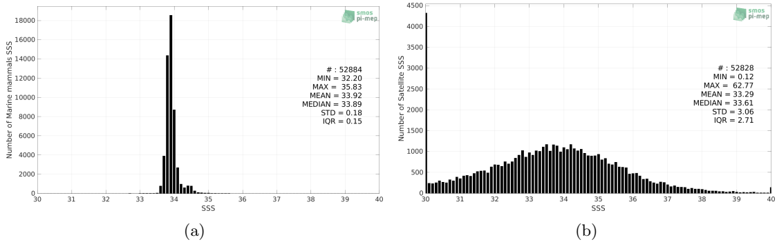
Figure 2: Histograms of SSS from Marine mammals (a) and SMOS SSS L2Q v331 - No FLAG (CMEMS-CATDS-CPDC) (b) considering all match-up pairs per bins of 0.1 over the Roaring Forties and Furious Fifties Pi-MEP region and for the full satellite product period.
