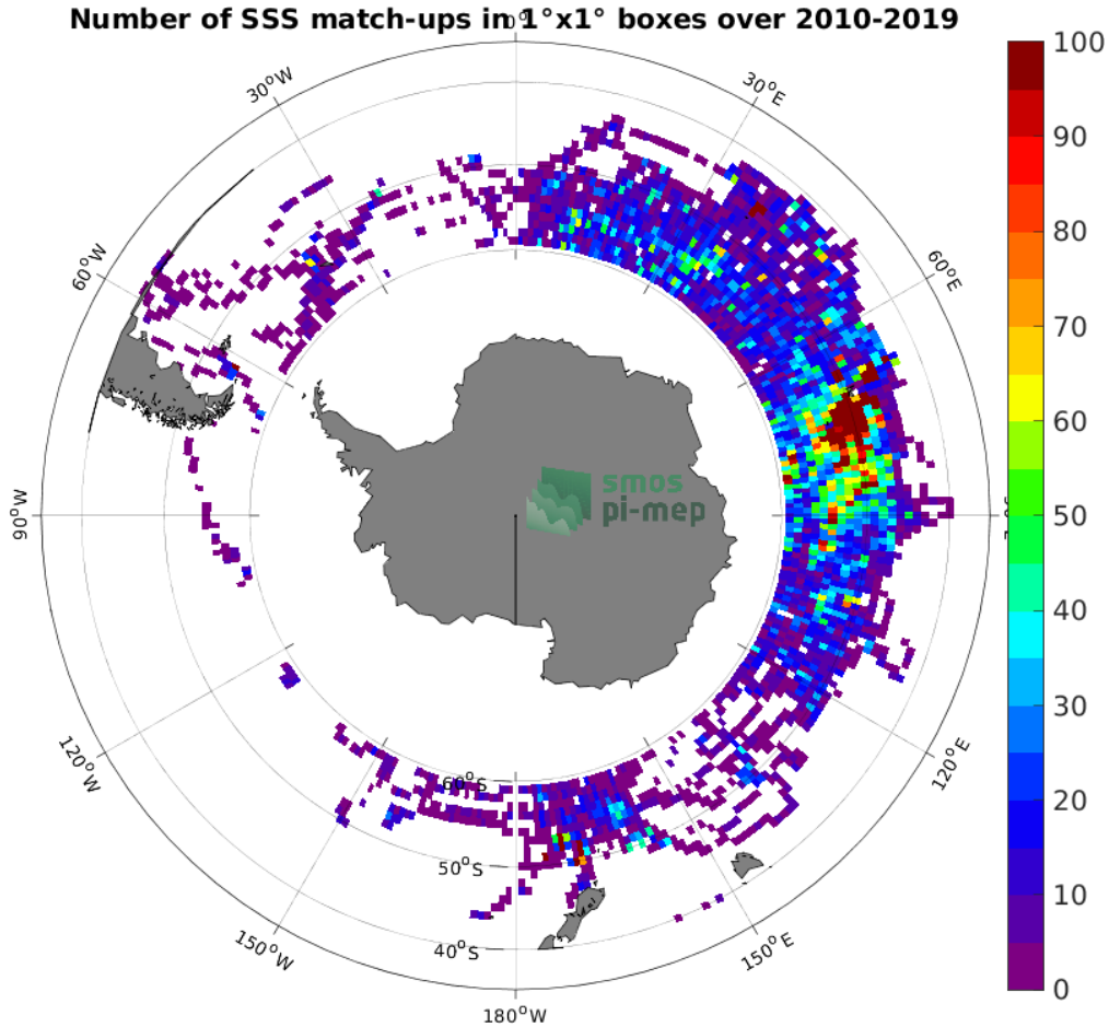
Figure 4: Number of SSS match-ups between Marine mammals SSS and the SMOS SSS L2Q v331 - No FLAG (CMEMS-CATDS-CPDC) SSS product for the Roaring Forties and Furious Fifties Pi-MEP region over 1^\circ \times 1^\circ boxes and for the full satellite product period.
