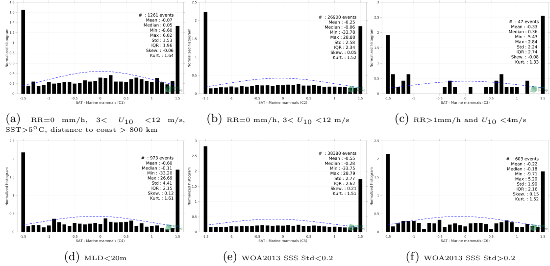
Figure 13: Normalized histogram of \Delta SSS (SMOS SSS L2Q v331 - No FLAG (CMEMS-CATDS-CPDC) - Marine mammals) for 6 different subdatasets corresponding to: RR=0 mm/h, 3 < U_{10} < 12 m/s, SST>5°C, distance to coast > 800 km (a), RR=0 mm/h, 3 < U_{10} < 12 m/s (b), RR>1mm/h and U_{10} < 4 m/s (c), MLD<20m (d), WOA2013 SSS Std<0.2 (e), WOA2013 SSS Std>0.2 (f).
