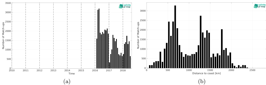
Figure 2: Number of match-ups between Surface drifters and SMOS SSS L2Q v331 - No FLAG (CMEMS-CATDS-CPDC) SSS as a function of time (a) and as function of the distance to coast (b) over the Roaring Forties and Furious Fifties Pi-MEP region and for the full satellite product period.
