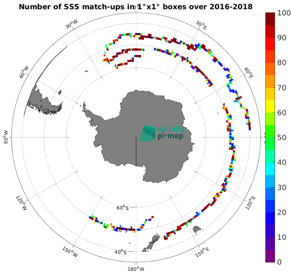
Figure 4: Number of SSS match-ups between Surface drifters SSS and the SMOS SSS L2Q v331 - No FLAG (CMEMS-CATDS-CPDC) SSS product for the Roaring Forties and Furious Fifties Pi-MEP region over 1^\circ \times 1^\circ boxes and for the full satellite product period.
