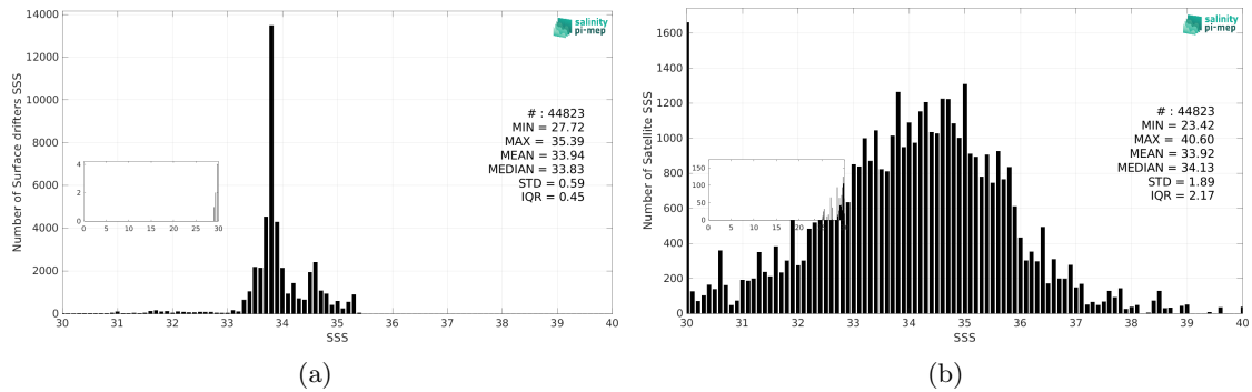
Figure 3: Histograms of SSS from Surface drifters (a) and SMOS SSS L2Q v331 - No FLAG (CMEMS-CATDS-CPDC) (b) considering all match-up pairs per bins of 0.1 over the Roaring Forties and Furious Fifties Pi-MEP region and for the full satellite product period.
