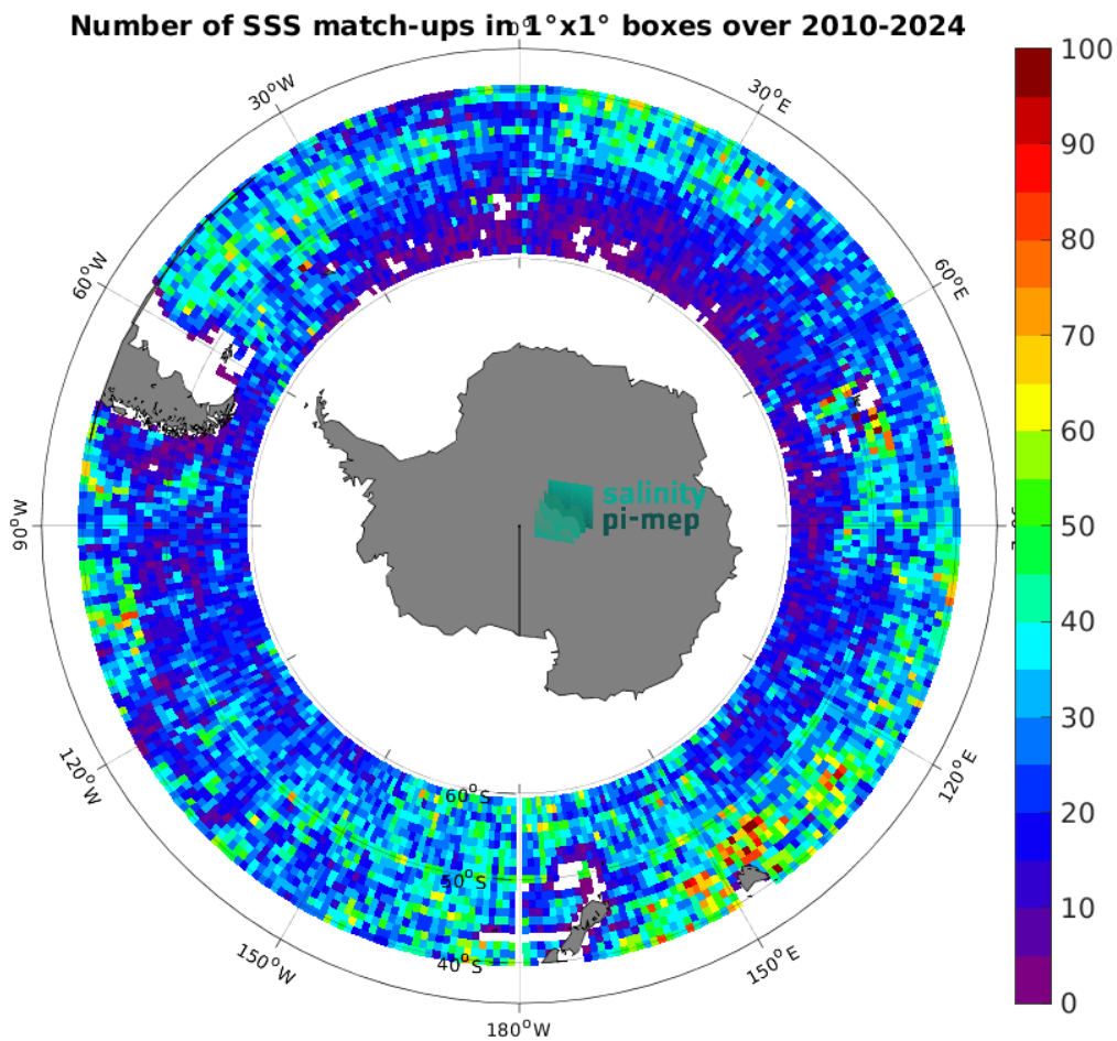
Figure 5: Number of SSS match-ups between Argo SSS and the SMOS SSS L2Q v331 - No FLAG (CMEMS-CATDS-CPDC) SSS product for the Roaring Forties and Furious Fifties Pi-MEP region over 1^\circ \times 1^\circ boxes and for the full satellite product period.
