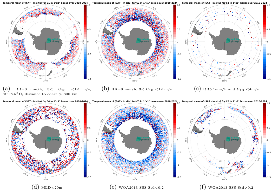
Figure 14: Temporal mean gridded over spatial boxes of size 1^\circ \times 1^\circ of \Delta SSS (SMOS SSS L2Q v331 - No FLAG (CMEMS-CATDS-CPDC) - Argo) for 6 different subdatasets corresponding to:RR=0 mm/h, 3 < U_{10} < 12 m/s, SST>5°C, distance to coast > 800 km (a), RR=0 mm/h, 3 < U_{10} < 12 m/s (b), RR>1mm/h and U_{10} < 4 m/s (c),MLD<20m (d),WOA2013 SSS Std<0.2 (e),WOA2013 SSS Std>0.2 (f).
