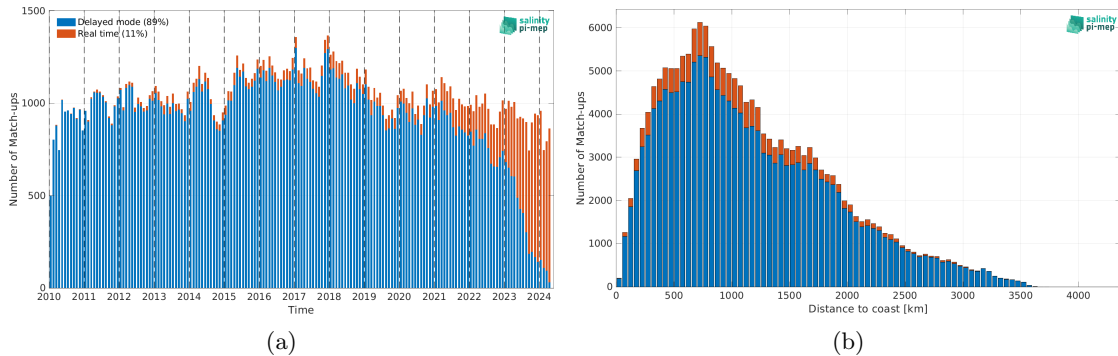
Figure 2: Number of match-ups between Argo and SMOS SSS L2Q v331 - No FLAG (CMEMS-CATDS-CPDC) SSS as a function of time (a) and as function of the distance to coast (b) over the Roaring Forties and Furious Fifties Pi-MEP region and for the full satellite product period.
