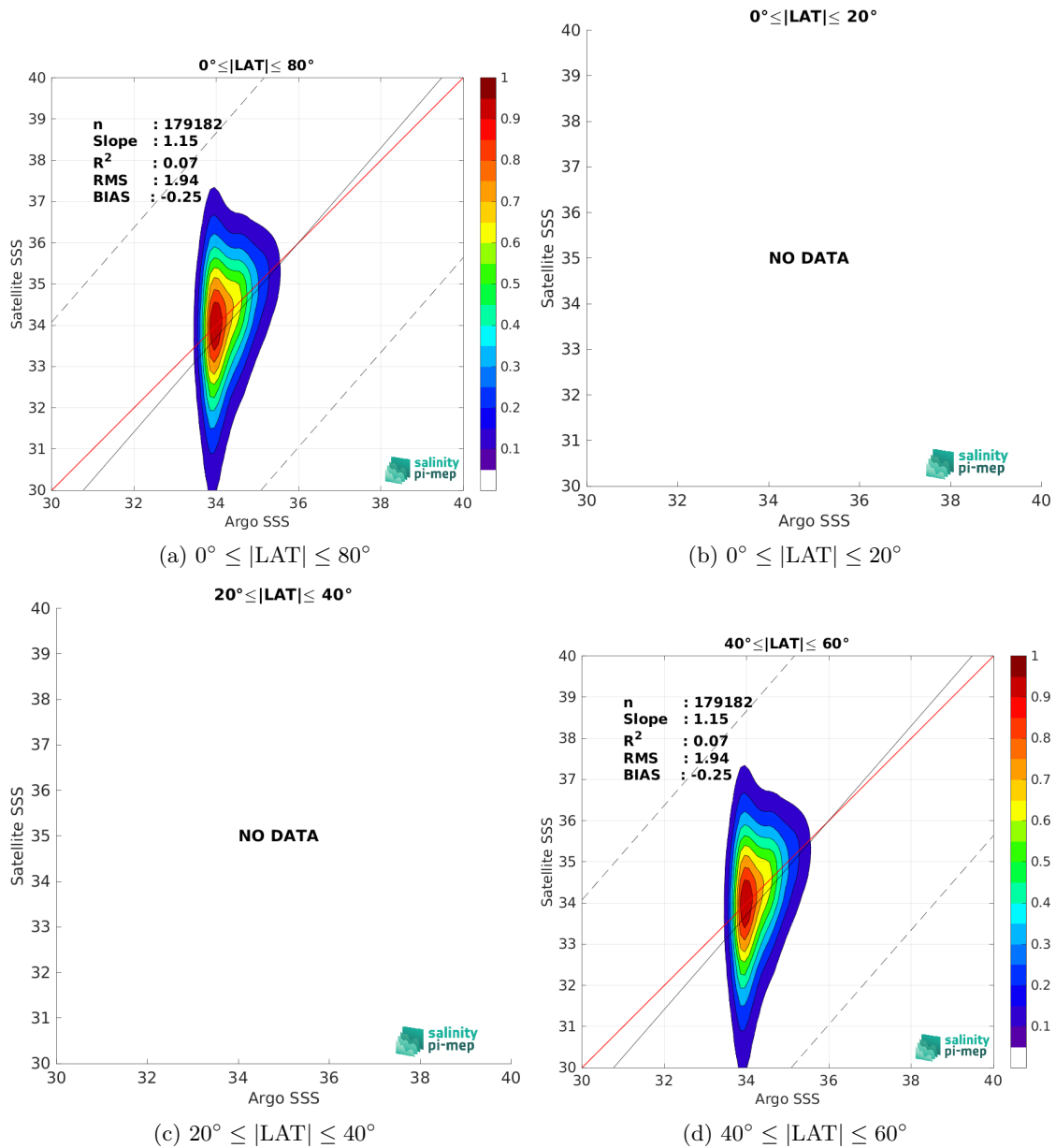
Figure 10: Contour maps of the concentration of SMOS SSS L2Q v331 - No FLAG (CMEMS-CATDS-CPDC) SSS (y-axis) versus Argo SSS (x-axis) at match-up pairs for different latitude bands. For each plot, the red line shows x=y . The black thin and dashed lines indicate a linear fit through the data cloud and the \pm 95\% confidence levels, respectively. The number match-up pairs n , the slope and R^2 coefficient of the linear fit, the root mean square (RMS) and the mean bias between satellite and in situ data are indicated for each latitude band in each plots.
