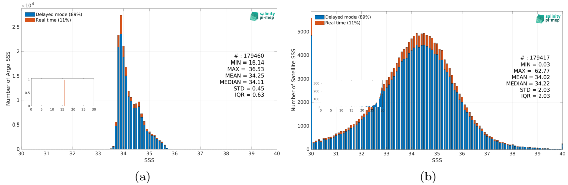
Figure 3: Histograms of SSS from Argo (a) and SMOS SSS L2Q v331 - No FLAG (CMEMS-CATDS-CPDC) (b) considering all match-up pairs per bins of 0.1 over the Roaring Forties and Furious Fifties Pi-MEP region and for the full satellite product period.
