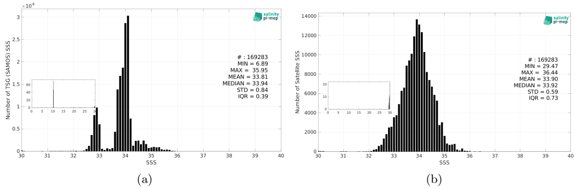
Figure 2: Histograms of SSS from TSG (SAMOS) (a) and SMOS SSS L3 v9 - 9 Days (CATDS-CEC-LOCEAN) (b) considering all match-up pairs per bins of 0.1 over the Roaring Forties and Furious Fifties Pi-MEP region and for the full satellite product period.
