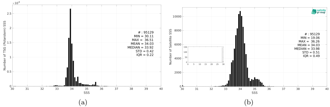
Figure 2: Histograms of SSS from TSG (Polarstern) (a) and SMOS SSS L3 v9 - 9 Days (CATDS-CEC-LOCEAN) (b) considering all match-up pairs per bins of 0.1 over the Roaring Forties and Furious Fifties Pi-MEP region and for the full satellite product period.
