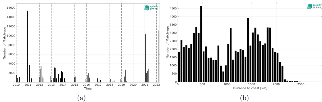
Figure 1: Number of match-ups between TSG (Polarstern) and SMOS SSS L3 v9 - 9 Days (CATDS-CEC-LOCEAN) SSS as a function of time (a) and as function of the distance to coast (b) over the Roaring Forties and Furious Fifties Pi-MEP region and for the full satellite product period.
