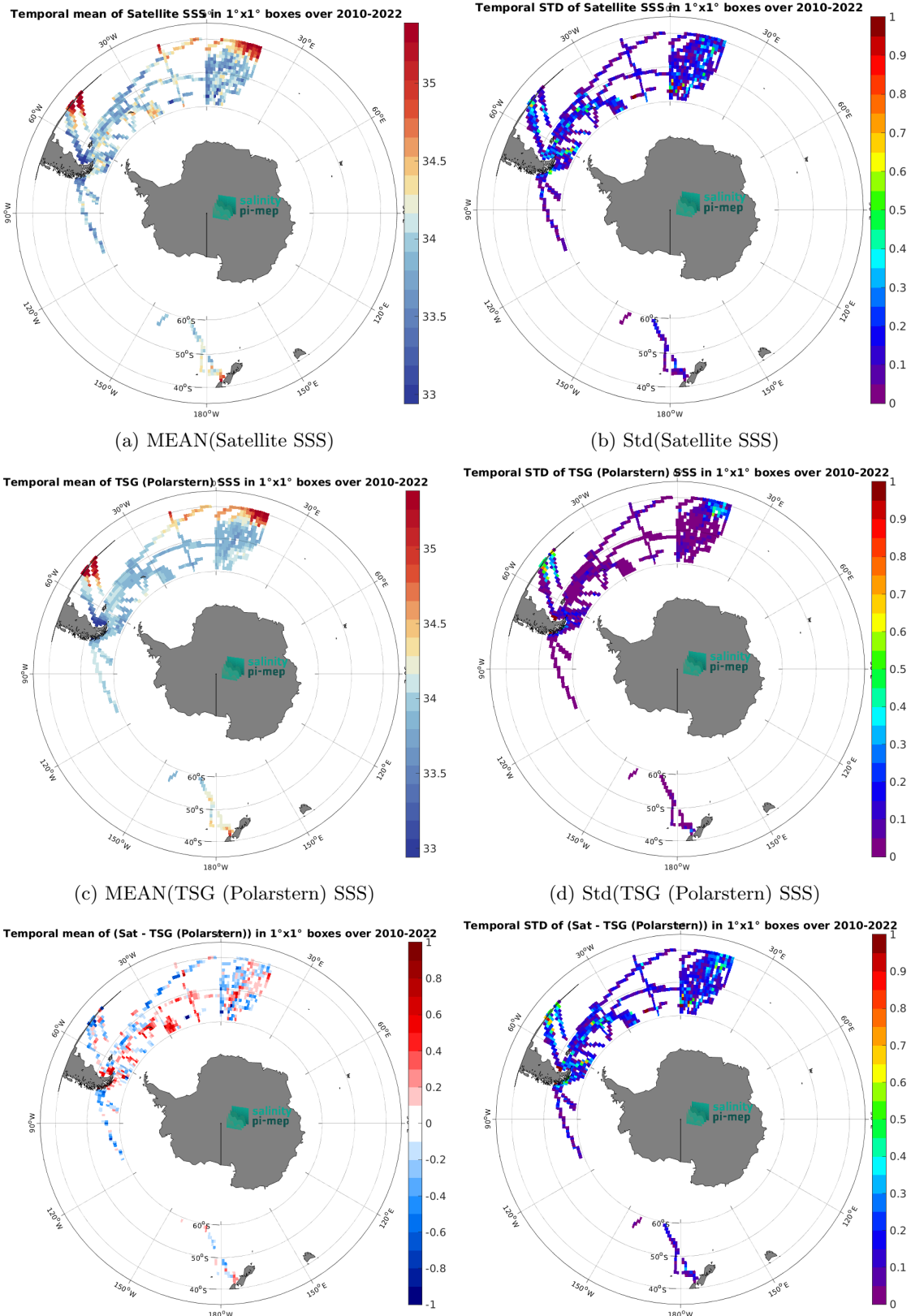
Figure 6: Temporal mean (left) and Std (right) of SSS from SMOS SSS L3 v9 - 9 Days (CATDS-CEC-LOCEAN) (top), TSG (Polarstern) (middle), and of \Delta SSS (Satellite - TSG (Polarstern)). Only match-up pairs are used to generate these maps.
