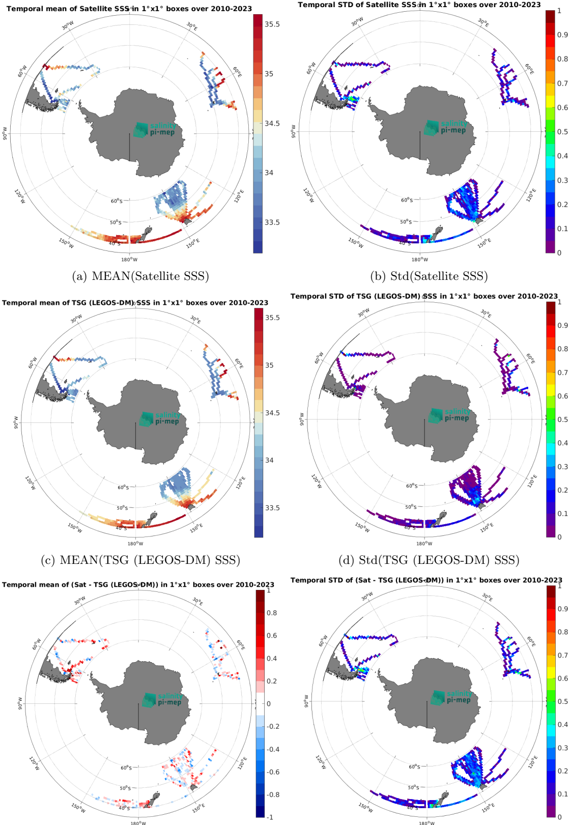
Figure 6: Temporal mean (left) and Std (right) of SSS from SMOS SSS L3 v9 - 9 Days (CATDS-CEC-LOCEAN) (top), TSG (LEGOS-DM) (middle), and of \Delta SSS (Satellite - TSG (LEGOS-DM)). Only match-up pairs are used to generate these maps.
