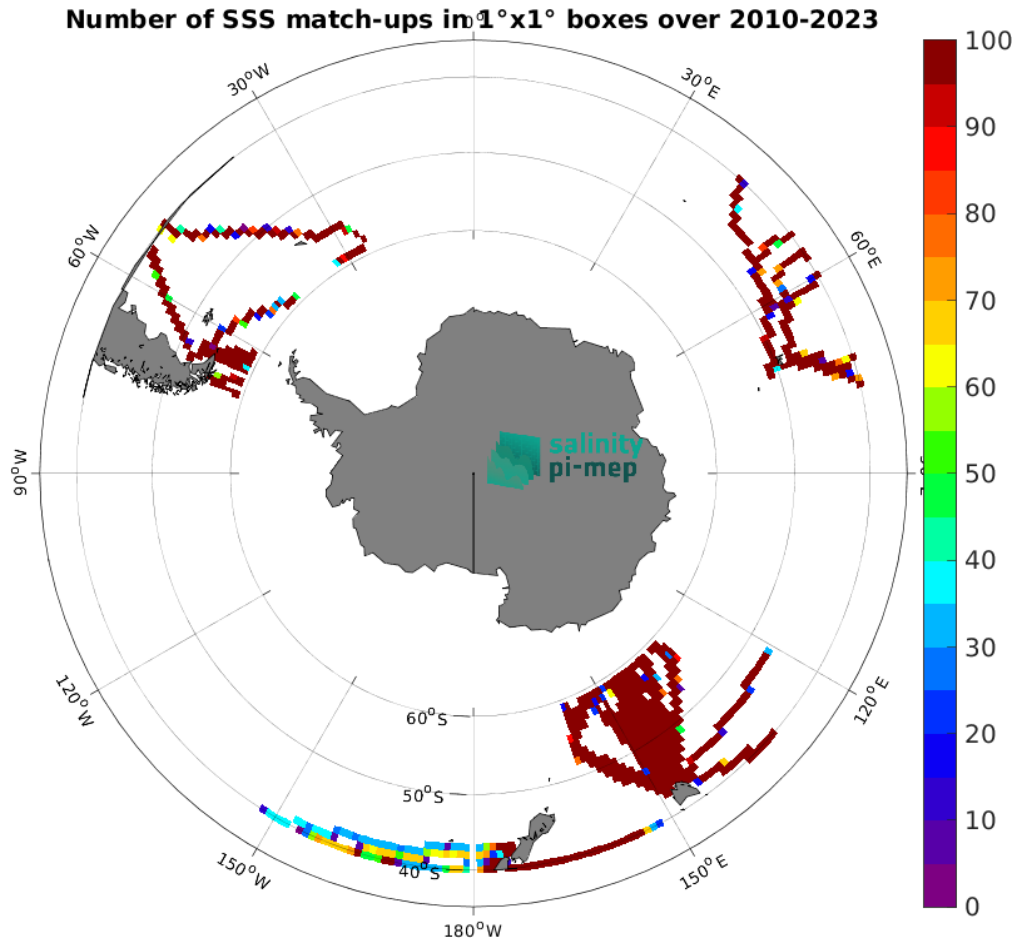
Figure 4: Number of SSS match-ups between TSG (LEGOS-DM) SSS and the SMOS SSS L3 v9 - 9 Days (CATDS-CEC-LOCEAN) SSS product for the Roaring Forties and Furious Fifties Pi-MEP region over 1^\circ \times 1^\circ boxes and for the full satellite product period.
