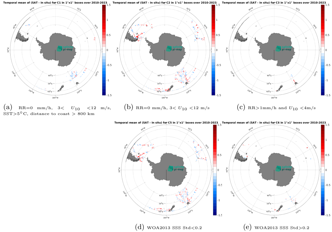
Figure 12: Temporal mean gridded over spatial boxes of size 1^{\circ}\times 1^{\circ} of \Delta\text{SSS} (SMOS SSS L3 v9 - 9 Days (CATDS-CEC-LOCEAN) - TSG (LEGOS-DM)) for 5 different subdatasets corresponding to:RR=0 mm/h, 3 < U_{10} < 12 m/s, SST >5^{\circ}\text{C} , distance to coast > 800 km (a), RR=0 mm/h, 3 < U_{10} < 12 m/s (b), RR >1 mm/h and U_{10} < 4 m/s (c), WOA2013 SSS Std <0.2 (d), WOA2013 SSS Std >0.2 (e).
