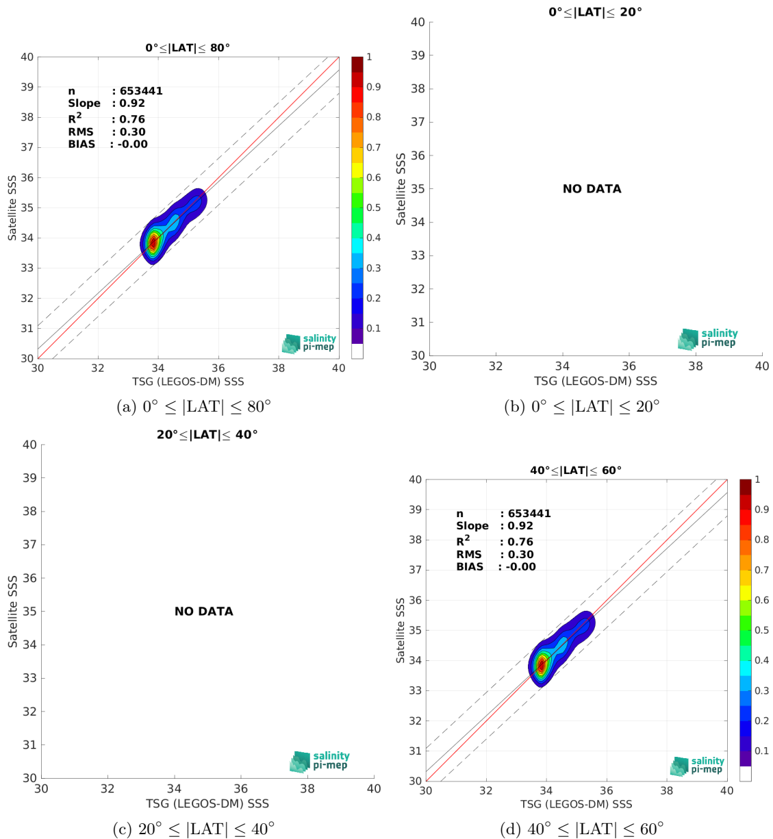
Figure 9: Contour maps of the concentration of SMOS SSS L3 v9 - 9 Days (CATDS-CEC-LOCEAN) SSS (y-axis) versus TSG (LEGOS-DM) SSS (x-axis) at match-up pairs for different latitude bands. For each plot, the red line shows x=y . The black thin and dashed lines indicate a linear fit through the data cloud and the \pm 95\% confidence levels, respectively. The number match-up pairs n , the slope and R^2 coefficient of the linear fit, the root mean square (RMS) and the mean bias between satellite and in situ data are indicated for each latitude band in each plots.
