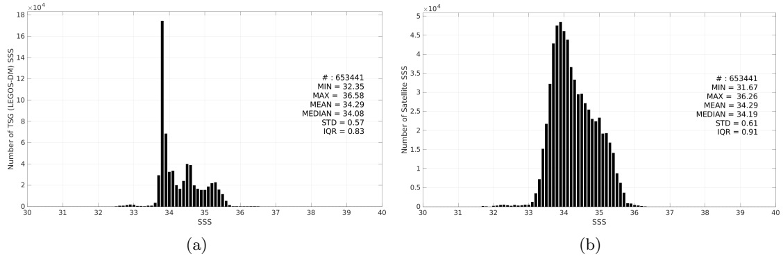
Figure 2: Histograms of SSS from TSG (LEGOS-DM) (a) and SMOS SSS L3 v9 - 9 Days (CATDS-CEC-LOCEAN) (b) considering all match-up pairs per bins of 0.1 over the Roaring Forties and Furious Fifties Pi-MEP region and for the full satellite product period.
