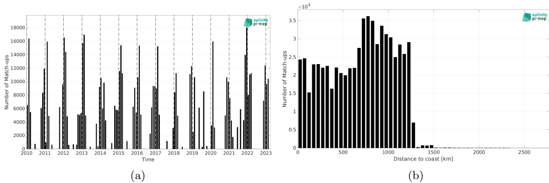
Figure 1: Number of match-ups between TSG (LEGOS-DM) and SMOS SSS L3 v9 - 9 Days (CATDS-CEC-LOCEAN) SSS as a function of time (a) and as function of the distance to coast (b) over the Roaring Forties and Furious Fifties Pi-MEP region and for the full satellite product period.
