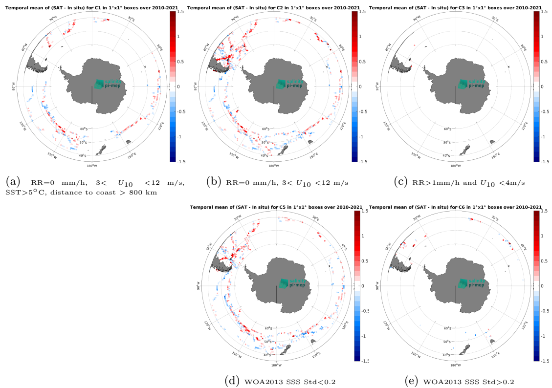
Figure 14: Temporal mean gridded over spatial boxes of size 1^\circ \times 1^\circ of \Delta\text{SSS} (SMOS SSS L3 v9 - 9 Days (CATDS-CEC-LOCEAN) - TSG (GOSUD-Sailing-ship)) for 5 different subdatasets corresponding to:RR=0 mm/h, 3 < U_{10} < 12 m/s, SST>5°C, distance to coast > 800 km (a), RR=0 mm/h, 3 < U_{10} < 12 m/s (b), RR>1mm/h and U_{10} < 4 m/s (c), WOA2013 SSS Std<0.2 (d), WOA2013 SSS Std>0.2 (e).
