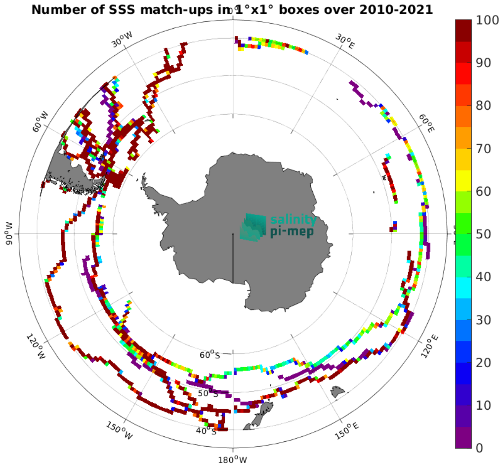
Figure 5: Number of SSS match-ups between TSG (GOSUD-Sailing-ship) SSS and the SMOS SSS L3 v9 - 9 Days (CATDS-CEC-LOCEAN) SSS product for the Roaring Forties and Furious Fifties Pi-MEP region over 1^\circ \times 1^\circ boxes and for the full satellite product period.
