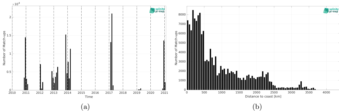
Figure 2: Number of match-ups between TSG (GOSUD-Sailing-ship) and SMOS SSS L3 v9 - 9 Days (CATDS-CEC-LOCEAN) SSS as a function of time (a) and as function of the distance to coast (b) over the Roaring Forties and Furious Fifties Pi-MEP region and for the full satellite product period.
