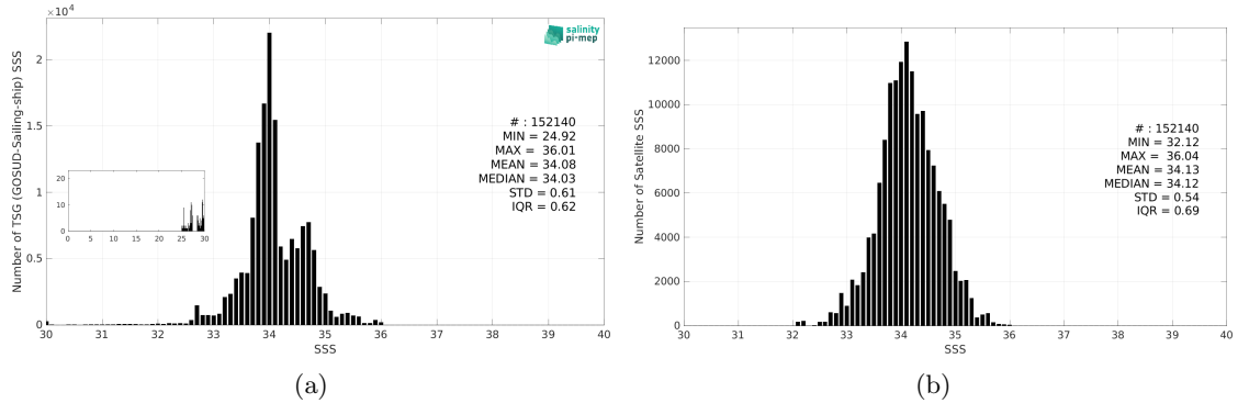
Figure 3: Histograms of SSS from TSG (GOSUD-Sailing-ship) (a) and SMOS SSS L3 v9 - 9 Days (CATDS-CEC-LOCEAN) (b) considering all match-up pairs per bins of 0.1 over the Roaring Forties and Furious Fifties Pi-MEP region and for the full satellite product period.
