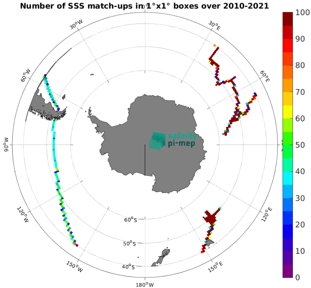
Figure 4: Number of SSS match-ups between TSG (GOSUD-Research-vessel) SSS and the SMOS SSS L3 v9 - 9 Days (CATDS-CEC-LOCEAN) SSS product for the Roaring Forties and Furious Fifties Pi-MEP region over 1^\circ \times 1^\circ boxes and for the full satellite product period.
