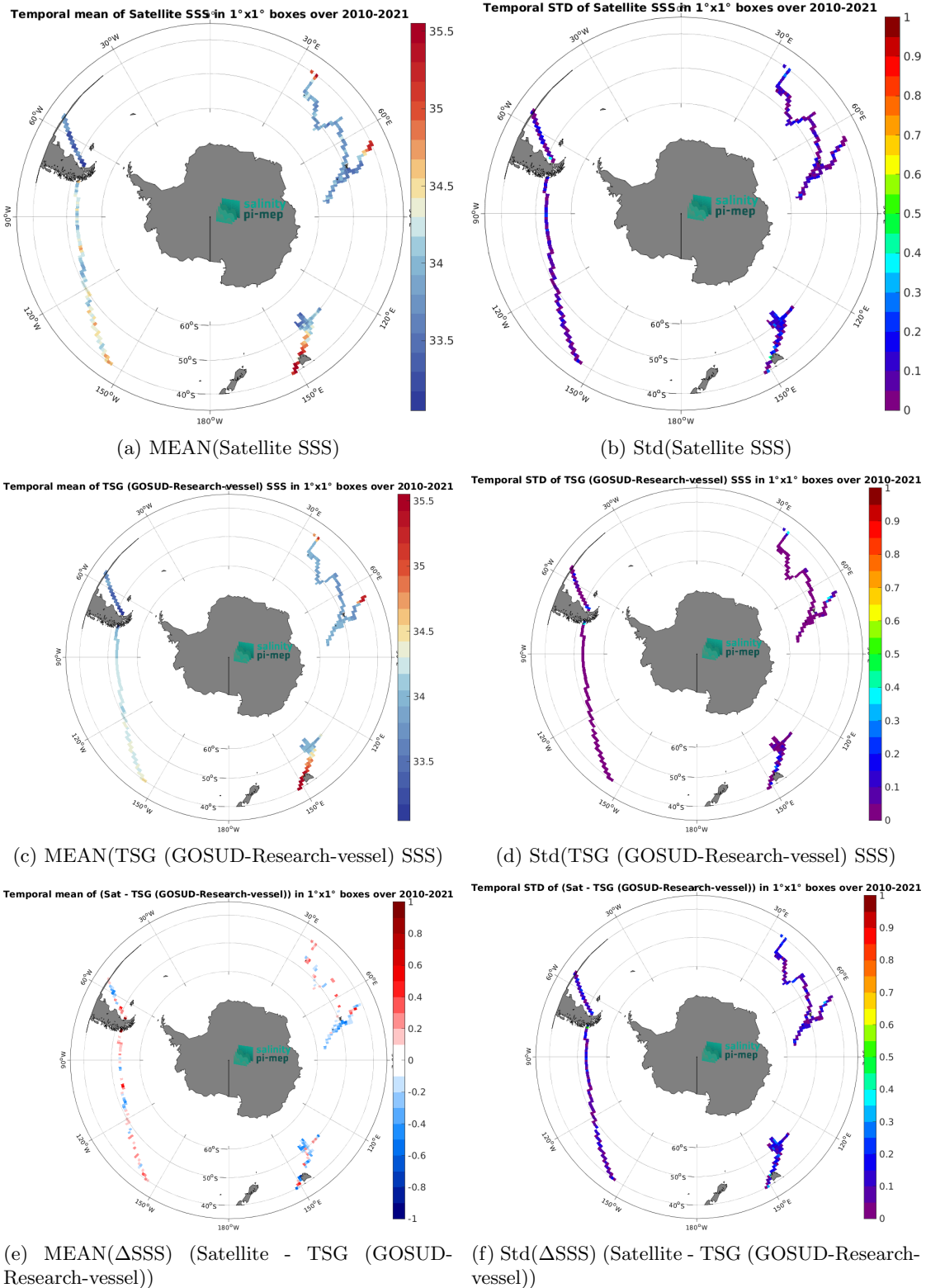
Figure 6: Temporal mean (left) and Std (right) of SSS from SMOS SSS L3 v9 - 9 Days (CATDS-CEC-LOCEAN) (top), TSG (GOSUD-Research-vessel) (middle), and of \Delta SSS (Satellite - TSG (GOSUD-Research-vessel)). Only match-up pairs are used to generate these maps.
