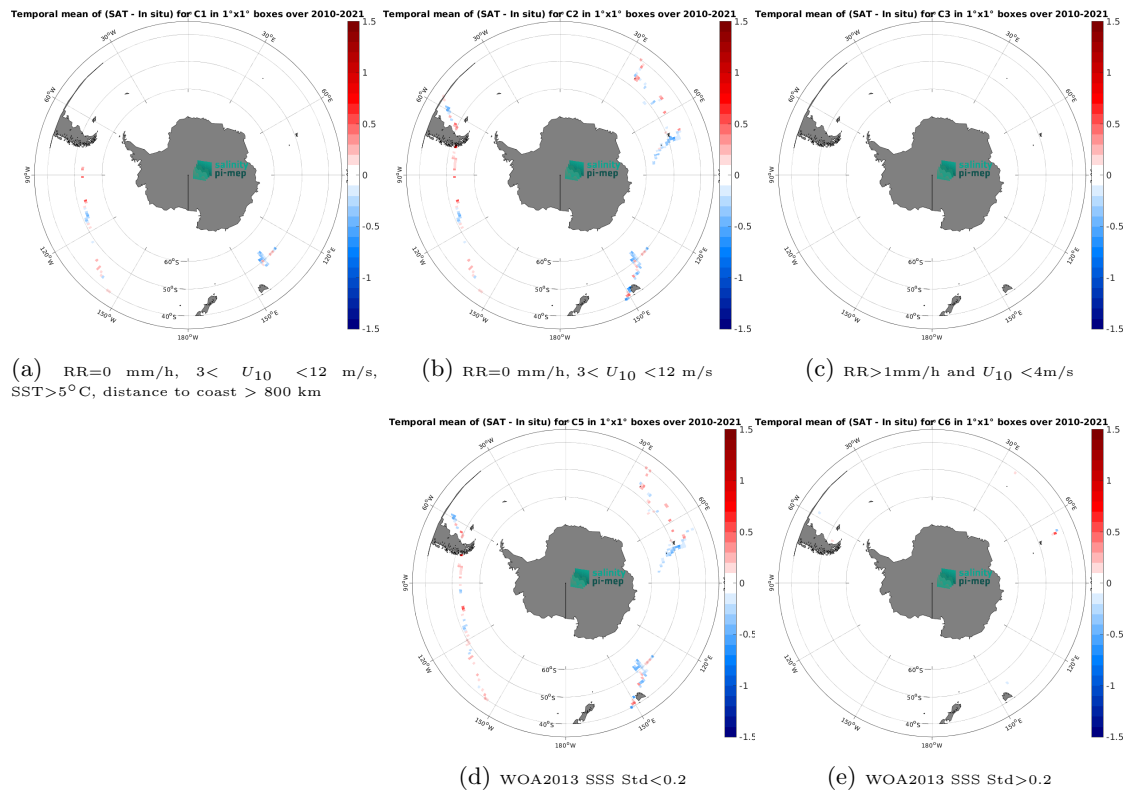
Figure 12: Temporal mean gridded over spatial boxes of size 1^\circ \times 1^\circ of \Delta SSS (SMOS SSS L3 v9 - 9 Days (CATDS-CEC-LOCEAN) - TSG (GOSUD-Research-vessel)) for 5 different subdatasets corresponding to:RR=0 mm/h, 3 < U_{10} < 12 m/s, SST>5°C, distance to coast > 800 km (a), RR=0 mm/h, 3 < U_{10} < 12 m/s (b), RR>1mm/h and U_{10} < 4 m/s (c), WOA2013 SSS Std<0.2 (d), WOA2013 SSS Std>0.2 (e).
