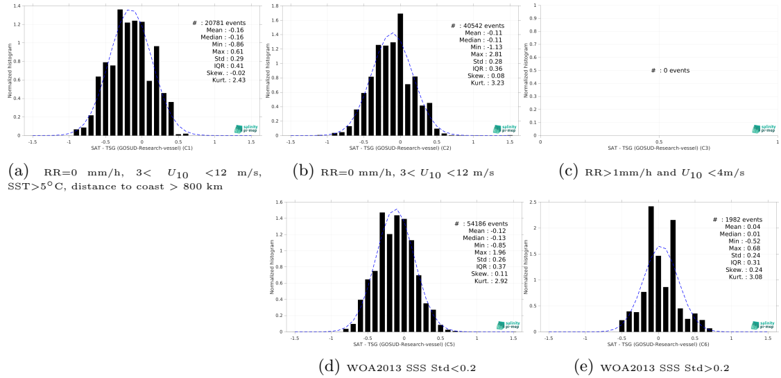
Figure 13: Normalized histogram of \Delta SSS (SMOS SSS L3 v9 - 9 Days (CATDS-CEC-LOCEAN) - TSG (GOSUD-Research-vessel)) for 5 different subdatasets corresponding to: RR=0 mm/h, 3 < U_{10} < 12 m/s, SST > 5°C, distance to coast > 800 km (a), RR=0 mm/h, 3 < U_{10} < 12 m/s (b), RR > 1mm/h and U_{10} < 4 m/s (c), WOA2013 SSS Std < 0.2 (d), WOA2013 SSS Std > 0.2 (e).
