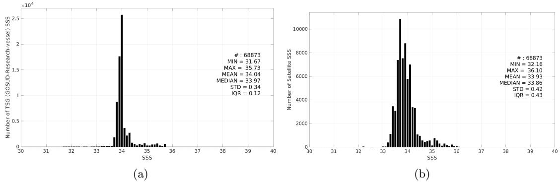
Figure 2: Histograms of SSS from TSG (GOSUD-Research-vessel) (a) and SMOS SSS L3 v9 - 9 Days (CATDS-CEC-LOCEAN) (b) considering all match-up pairs per bins of 0.1 over the Roaring Forties and Furious Fifties Pi-MEP region and for the full satellite product period.
