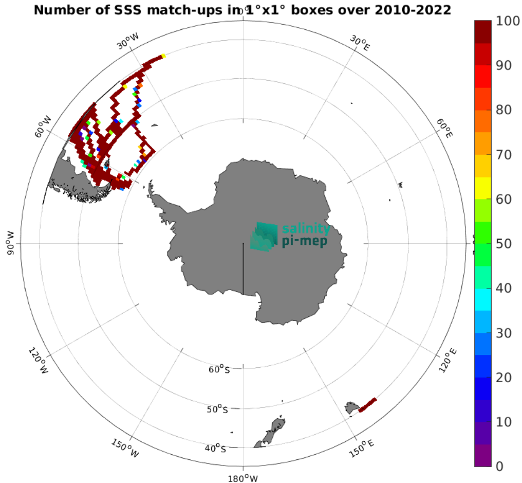
Figure 4: Number of SSS match-ups between TSG (CSIC-UTM) SSS and the SMOS SSS L3 v9 - 9 Days (CATDS-CEC-LOCEAN) SSS product for the Roaring Forties and Furious Fifties Pi-MEP region over 1^\circ \times 1^\circ boxes and for the full satellite product period.
