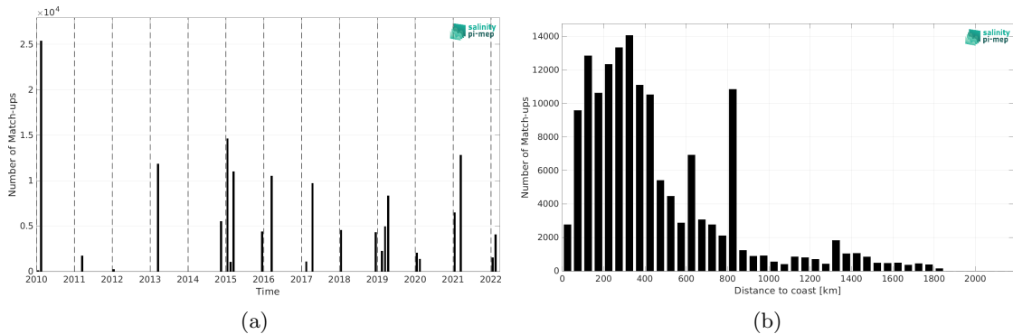
Figure 1: Number of match-ups between TSG (CSIC-UTM) and SMOS SSS L3 v9 - 9 Days (CATDS-CEC-LOCEAN) SSS as a function of time (a) and as function of the distance to coast (b) over the Roaring Forties and Furious Fifties Pi-MEP region and for the full satellite product period.
