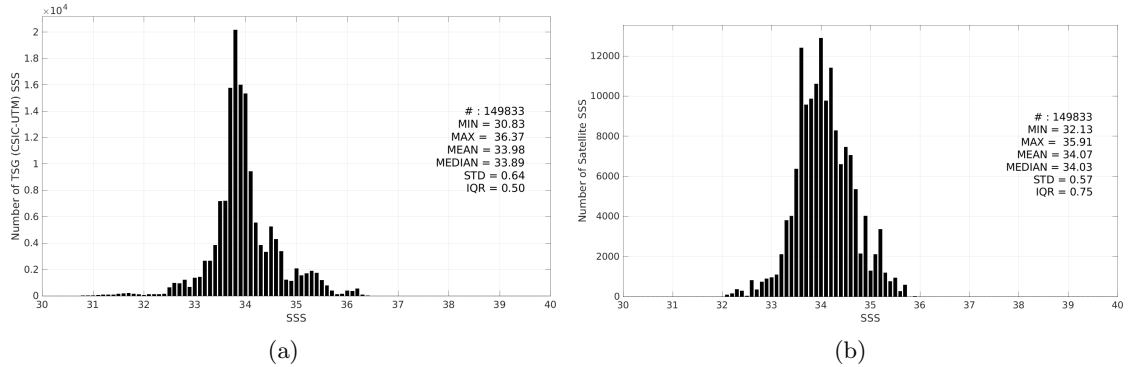
Figure 2: Histograms of SSS from TSG (CSIC-UTM) (a) and SMOS SSS L3 v9 - 9 Days (CATDS-CEC-LOCEAN) (b) considering all match-up pairs per bins of 0.1 over the Roaring Forties and Furious Fifties Pi-MEP region and for the full satellite product period.
