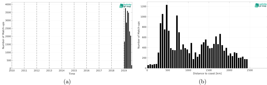
Figure 2: Number of match-ups between Saildrone and SMOS SSS L3 v9 - 9 Days (CATDS-CEC-LOCEAN) SSS as a function of time (a) and as function of the distance to coast (b) over the Roaring Forties and Furious Fifties Pi-MEP region and for the full satellite product period.
