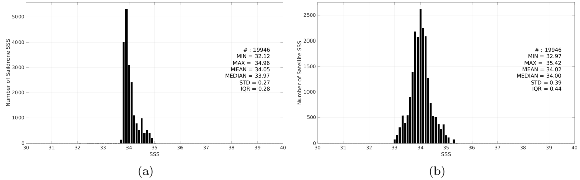
Figure 3: Histograms of SSS from Saildrone (a) and SMOS SSS L3 v9 - 9 Days (CATDS-CEC-LOCEAN) (b) considering all match-up pairs per bins of 0.1 over the Roaring Forties and Furious Fifties Pi-MEP region and for the full satellite product period.
