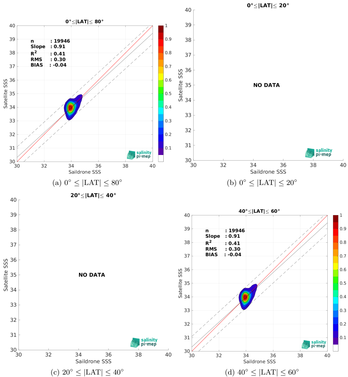
Figure 10: Contour maps of the concentration of SMOS SSS L3 v9 - 9 Days (CATDS-CEC-LOCEAN) SSS (y-axis) versus Saildrone SSS (x-axis) at match-up pairs for different latitude bands. For each plot, the red line shows x=y . The black thin and dashed lines indicate a linear fit through the data cloud and the \pm 95\% confidence levels, respectively. The number match-up pairs n , the slope and R^2 coefficient of the linear fit, the root mean square (RMS) and the mean bias between satellite and in situ data are indicated for each latitude band in each plots.
