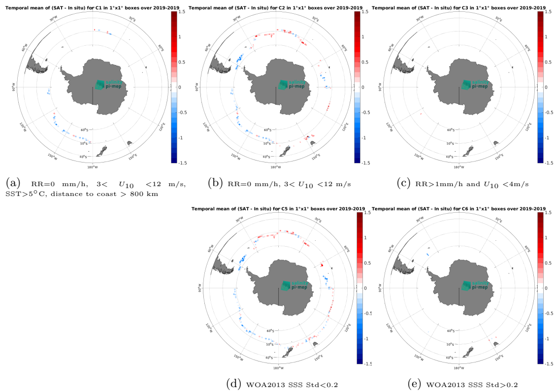
Figure 14: Temporal mean gridded over spatial boxes of size 1^\circ \times 1^\circ of \Delta\text{SSS} (SMOS SSS L3 v9 - 9 Days (CATDS-CEC-LOCEAN) - Saildrone) for 5 different subdatasets corresponding to:RR=0 mm/h, 3 < U_{10} < 12 m/s, SST >5^\circ\text{C} , distance to coast > 800 km (a), RR=0 mm/h, 3 < U_{10} < 12 m/s (b), RR >1 mm/h and U_{10} < 4 m/s (c), WOA2013 SSS Std <0.2 (d), WOA2013 SSS Std >0.2 (e).
