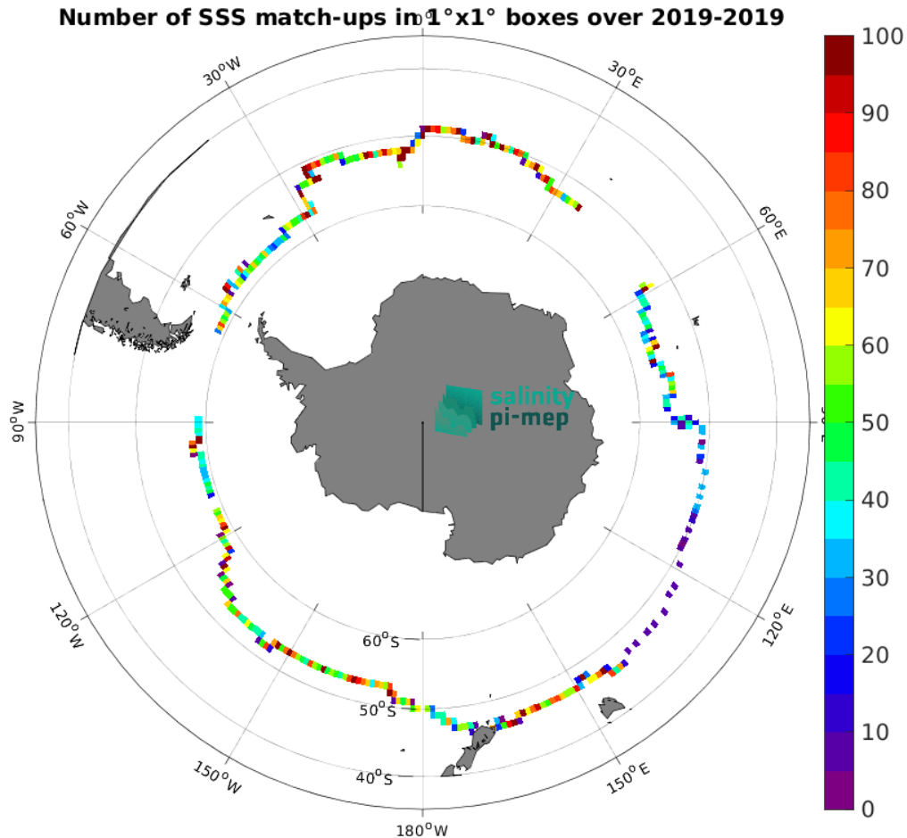
Figure 4: Number of SSS match-ups between Saildrone SSS and the SMOS SSS L3 v9 - 9 Days (CATDS-CEC-LOCEAN) SSS product for the Roaring Forties and Furious Fifties Pi-MEP region over 1^\circ \times 1^\circ boxes and for the full satellite product period.
