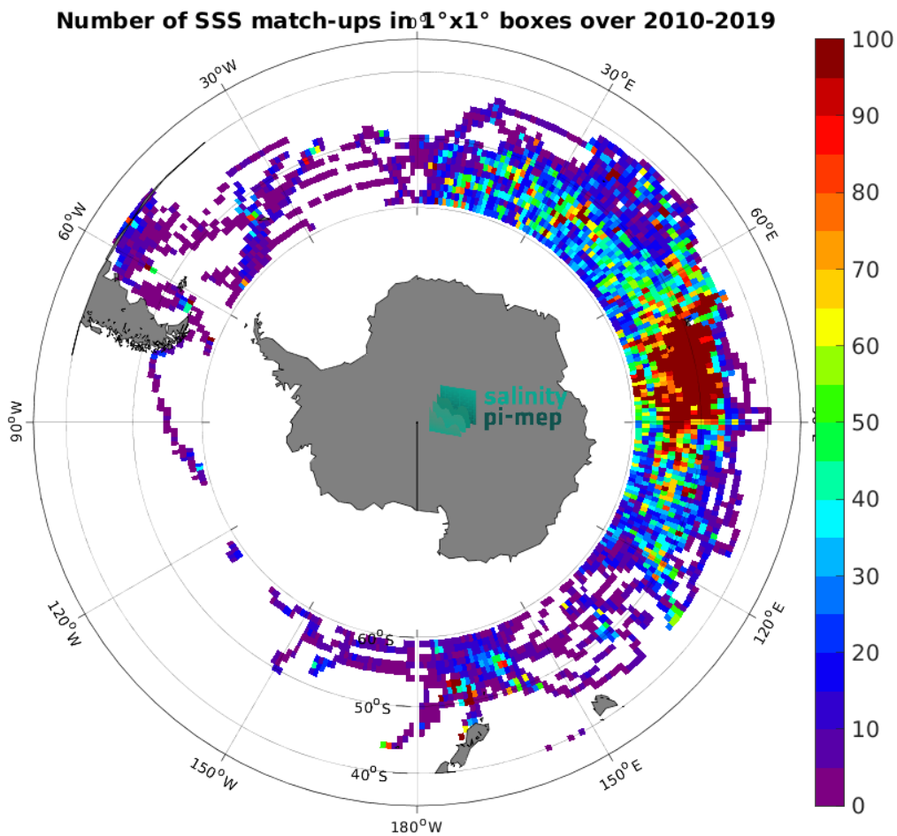
Figure 4: Number of SSS match-ups between Marine mammals SSS and the SMOS SSS L3 v9 - 9 Days (CATDS-CEC-LOCEAN) SSS product for the Roaring Forties and Furious Fifties Pi-MEP region over 1^\circ \times 1^\circ boxes and for the full satellite product period.
