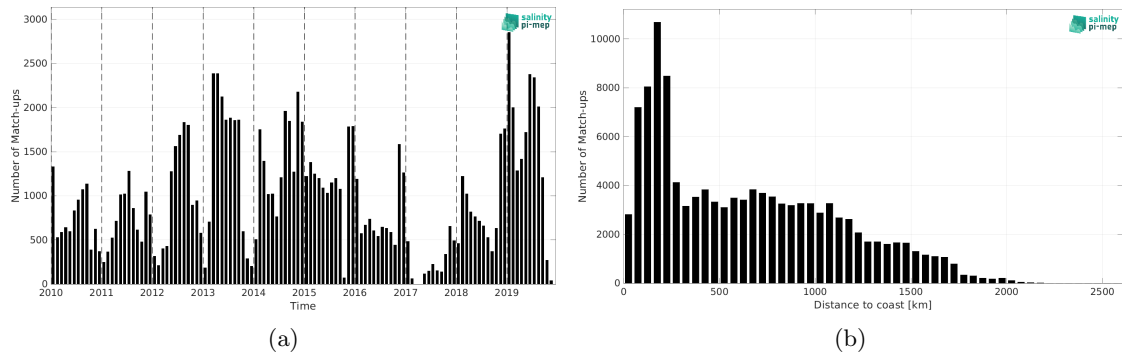
Figure 1: Number of match-ups between Marine mammals and SMOS SSS L3 v9 - 9 Days (CATDS-CEC-LOCEAN) SSS as a function of time (a) and as function of the distance to coast (b) over the Roaring Forties and Furious Fifties Pi-MEP region and for the full satellite product period.
