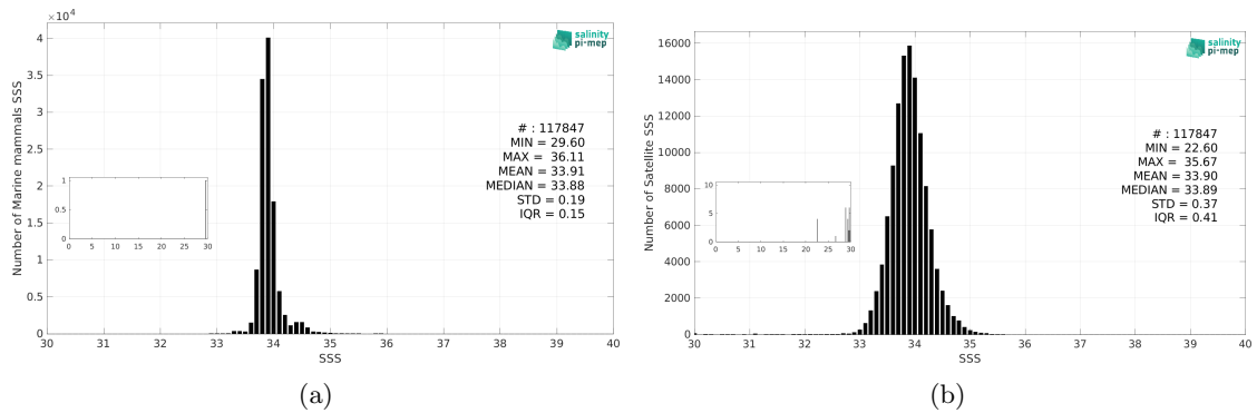
Figure 2: Histograms of SSS from Marine mammals (a) and SMOS SSS L3 v9 - 9 Days (CATDS-CEC-LOCEAN) (b) considering all match-up pairs per bins of 0.1 over the Roaring Forties and Furious Fifties Pi-MEP region and for the full satellite product period.
