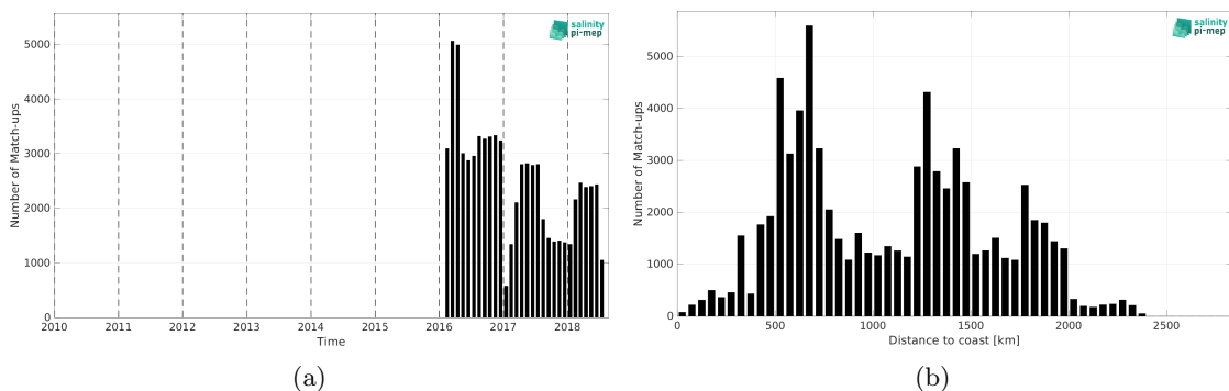
Figure 1: Number of match-ups between Surface drifters and SMOS SSS L3 v9 - 9 Days (CATDS-CEC-LOCEAN) SSS as a function of time (a) and as function of the distance to coast (b) over the Roaring Forties and Furious Fifties Pi-MEP region and for the full satellite product period.
