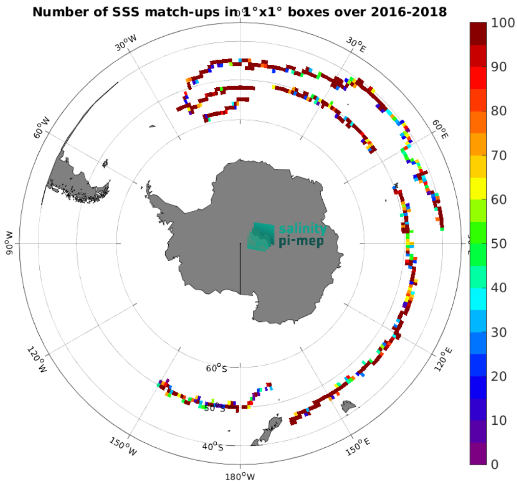
Figure 3: Number of SSS match-ups between Surface drifters SSS and the SMOS SSS L3 v9 - 9 Days (CATDS-CEC-LOCEAN) SSS product for the Roaring Forties and Furious Fifties Pi-MEP region over 1^\circ \times 1^\circ boxes and for the full satellite product period.
