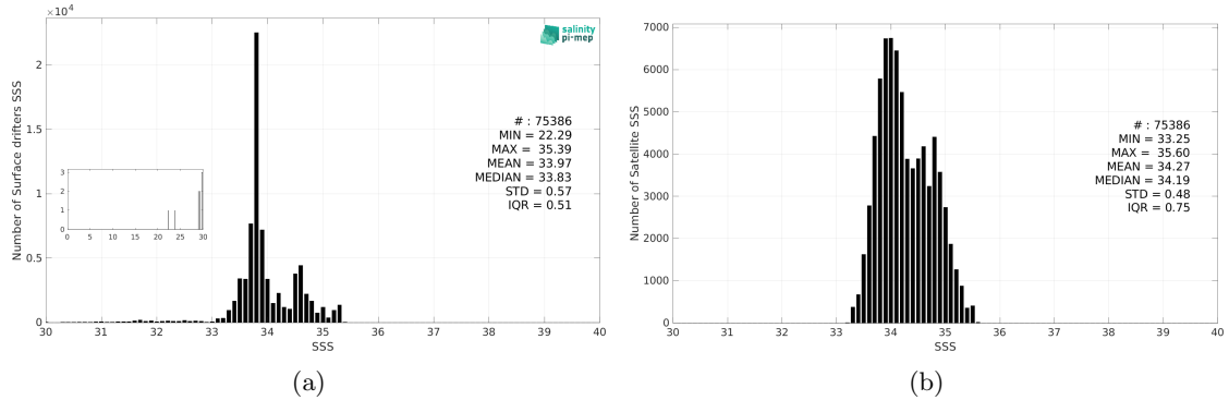
Figure 2: Histograms of SSS from Surface drifters (a) and SMOS SSS L3 v9 - 9 Days (CATDS-CEC-LOCEAN) (b) considering all match-up pairs per bins of 0.1 over the Roaring Forties and Furious Fifties Pi-MEP region and for the full satellite product period.
