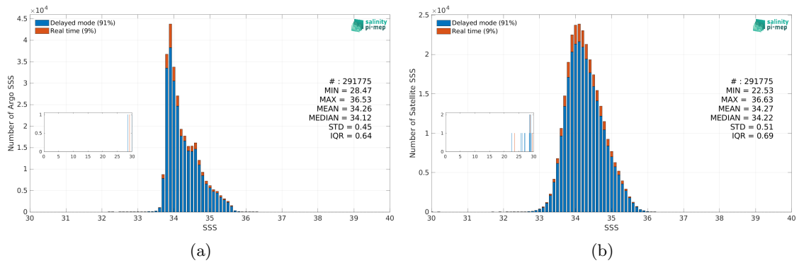
Figure 3: Histograms of SSS from Argo (a) and SMOS SSS L3 v9 - 9 Days (CATDS-CEC-LOCEAN) (b) considering all match-up pairs per bins of 0.1 over the Roaring Forties and Furious Fifties Pi-MEP region and for the full satellite product period.
