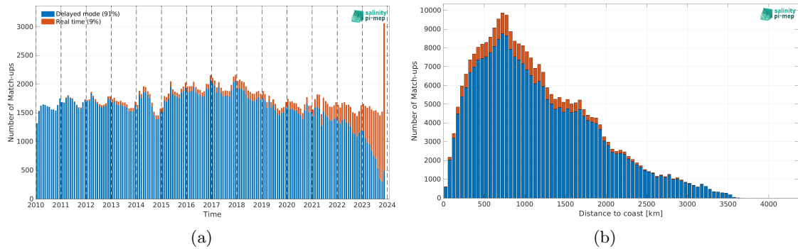
Figure 2: Number of match-ups between Argo and SMOS SSS L3 v9 - 9 Days (CATDS-CEC-LOCEAN) SSS as a function of time (a) and as function of the distance to coast (b) over the Roaring Forties and Furious Fifties Pi-MEP region and for the full satellite product period.
