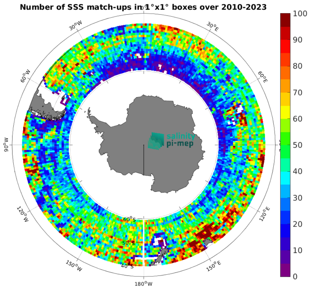
Figure 5: Number of SSS match-ups between Argo SSS and the SMOS SSS L3 v9 - 9 Days (CATDS-CEC-LOCEAN) SSS product for the Roaring Forties and Furious Fifties Pi-MEP region over 1^{\circ} \times 1^{\circ} boxes and for the full satellite product period.
