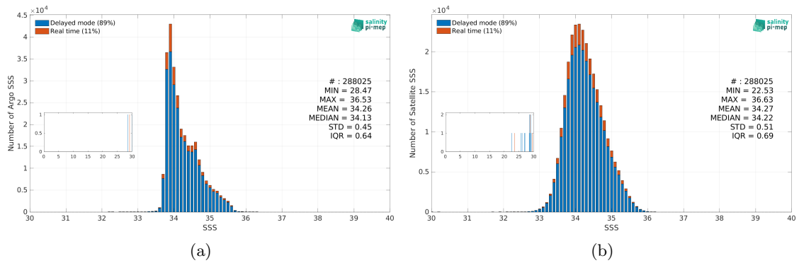
Figure 2: Histograms of SSS from Argo (a) and SMOS SSS L3 v9 - 9 Days (CATDS-CEC-LOCEAN) (b) considering all match-up pairs per bins of 0.1 over the Roaring Forties and Furious Fifties Pi-MEP region and for the full satellite product period.
