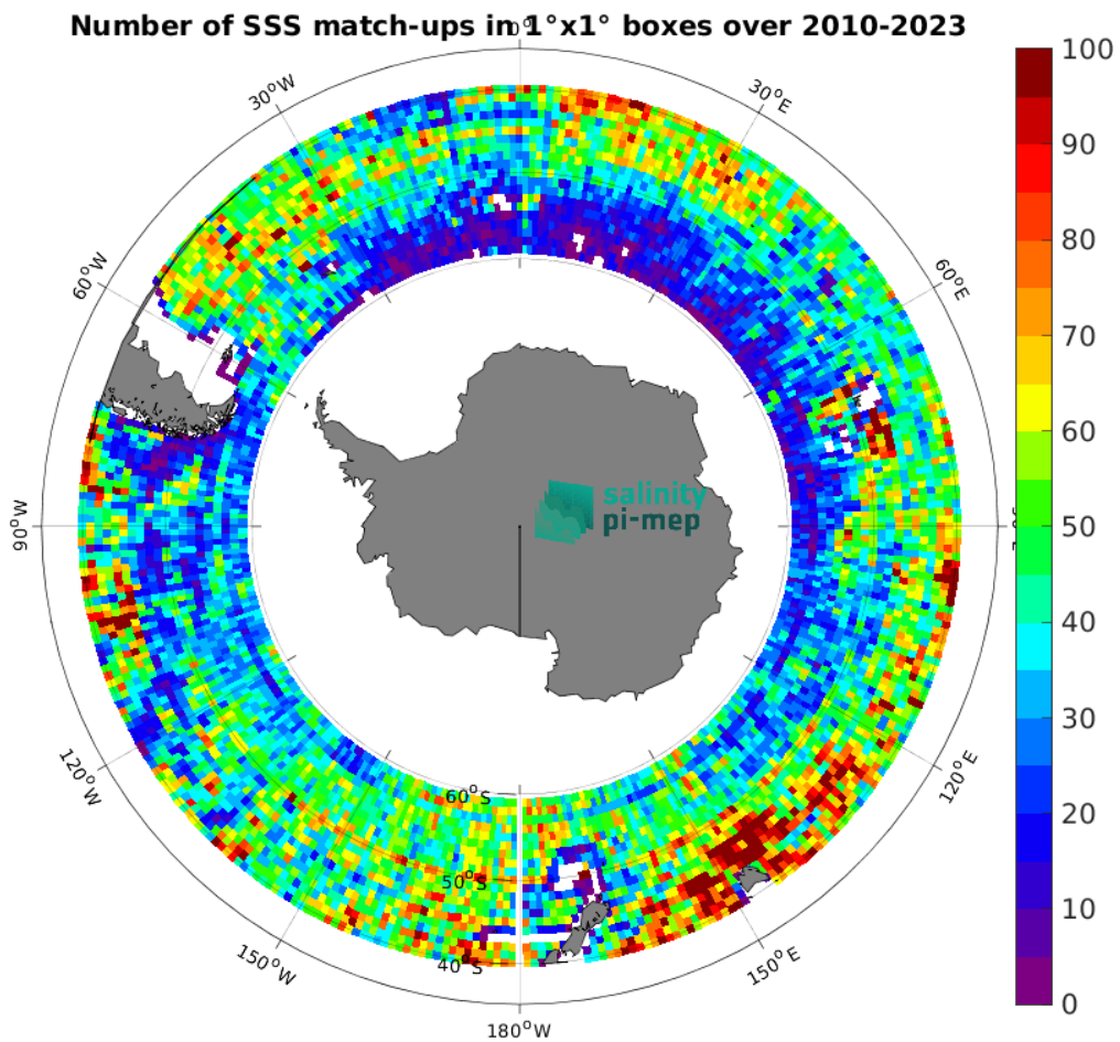
Figure 4: Number of SSS match-ups between Argo SSS and the SMOS SSS L3 v9 - 9 Days (CATDS-CEC-LOCEAN) SSS product for the Roaring Forties and Furious Fifties Pi-MEP region over 1^\circ \times 1^\circ boxes and for the full satellite product period.
