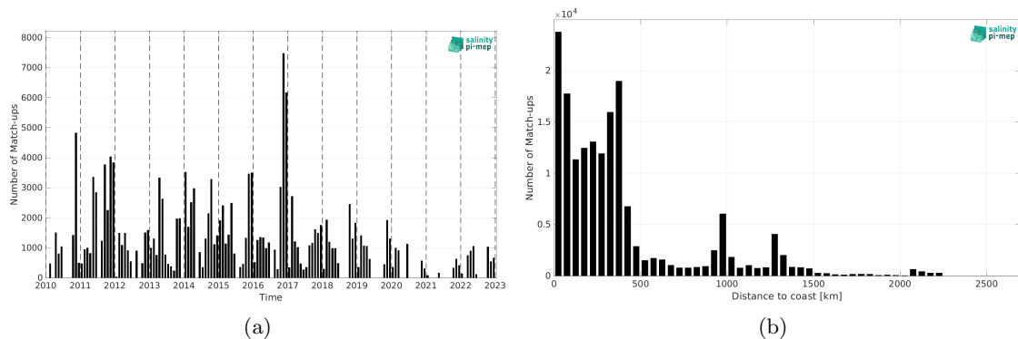
Figure 2: Number of match-ups between TSG (SAMOS) and SMOS SSS L3 v9 - 18 Days (CATDS-CEC-LOCEAN) SSS as a function of time (a) and as function of the distance to coast (b) over the Roaring Forties and Furious Fifties Pi-MEP region and for the full satellite product period.
