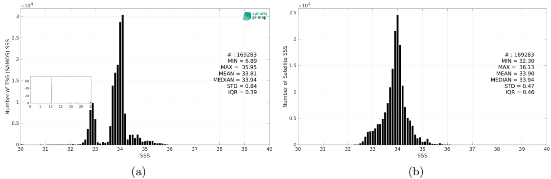
Figure 3: Histograms of SSS from TSG (SAMOS) (a) and SMOS SSS L3 v9 - 18 Days (CATDS-CEC-LOCEAN) (b) considering all match-up pairs per bins of 0.1 over the Roaring Forties and Furious Fifties Pi-MEP region and for the full satellite product period.
