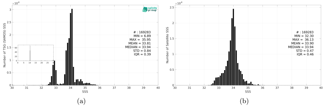
Figure 2: Histograms of SSS from TSG (SAMOS) (a) and SMOS SSS L3 v9 - 18 Days (CATDS-CEC-LOCEAN) (b) considering all match-up pairs per bins of 0.1 over the Roaring Forties and Furious Fifties Pi-MEP region and for the full satellite product period.
