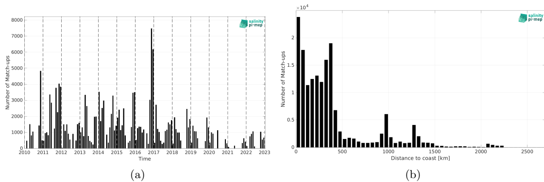
Figure 1: Number of match-ups between TSG (SAMOS) and SMOS SSS L3 v9 - 18 Days (CATDS-CEC-LOCEAN) SSS as a function of time (a) and as function of the distance to coast (b) over the Roaring Forties and Furious Fifties Pi-MEP region and for the full satellite product period.
