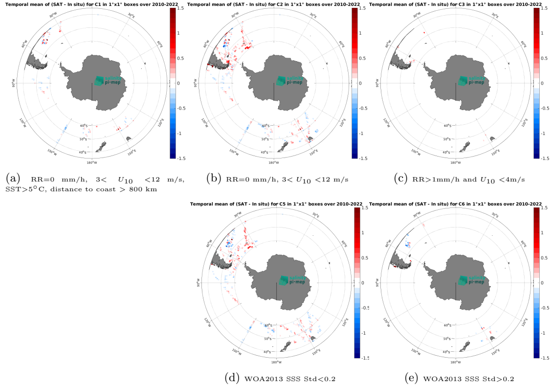
Figure 12: Temporal mean gridded over spatial boxes of size 1^{\circ}\times 1^{\circ} of \Delta\text{SSS} (SMOS SSS L3 v9 - 18 Days (CATDS-CEC-LOCEAN) - TSG (SAMOS)) for 5 different subdatasets corresponding to: \text{RR}=0 mm/h, 3 < U_{10} < 12 m/s, \text{SST}>5^{\circ}\text{C} , distance to coast > 800 km (a), \text{RR}=0 mm/h, 3 < U_{10} < 12 m/s (b), \text{RR}>1 mm/h and U_{10} < 4 m/s (c), WOA2013 SSS Std <0.2 (d), WOA2013 SSS Std >0.2 (e).
