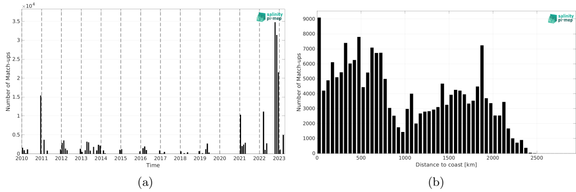
Figure 2: Number of match-ups between TSG (Polarstern) and SMOS SSS L3 v9 - 18 Days (CATDS-CEC-LOCEAN) SSS as a function of time (a) and as function of the distance to coast (b) over the Roaring Forties and Furious Fifties Pi-MEP region and for the full satellite product period.
