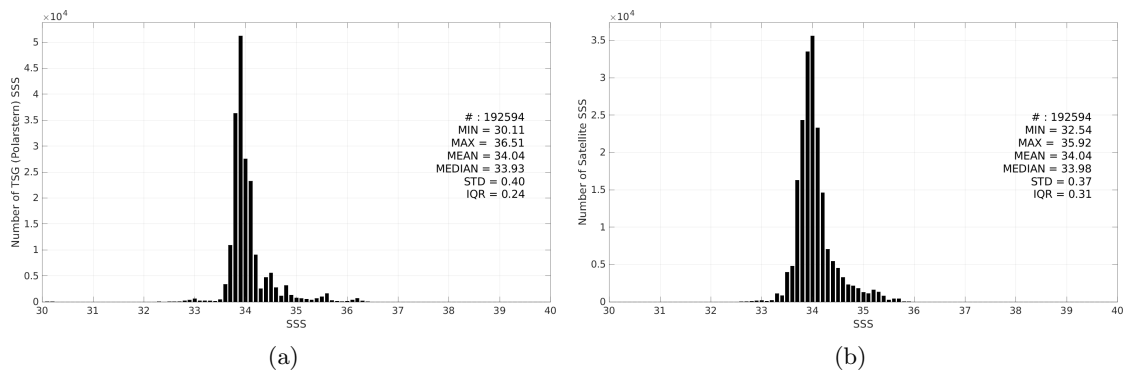
Figure 3: Histograms of SSS from TSG (Polarstern) (a) and SMOS SSS L3 v9 - 18 Days (CATDS-CEC-LOCEAN) (b) considering all match-up pairs per bins of 0.1 over the Roaring Forties and Furious Fifties Pi-MEP region and for the full satellite product period.
