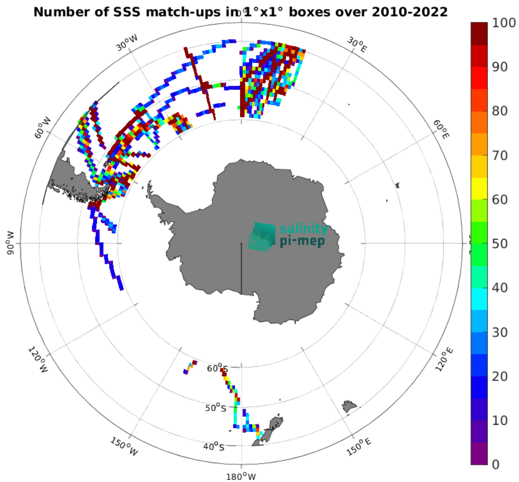
Figure 4: Number of SSS match-ups between TSG (Polarstern) SSS and the SMOS SSS L3 v9 - 18 Days (CATDS-CEC-LOCEAN) SSS product for the Roaring Forties and Furious Fifties Pi-MEP region over 1^\circ \times 1^\circ boxes and for the full satellite product period.
