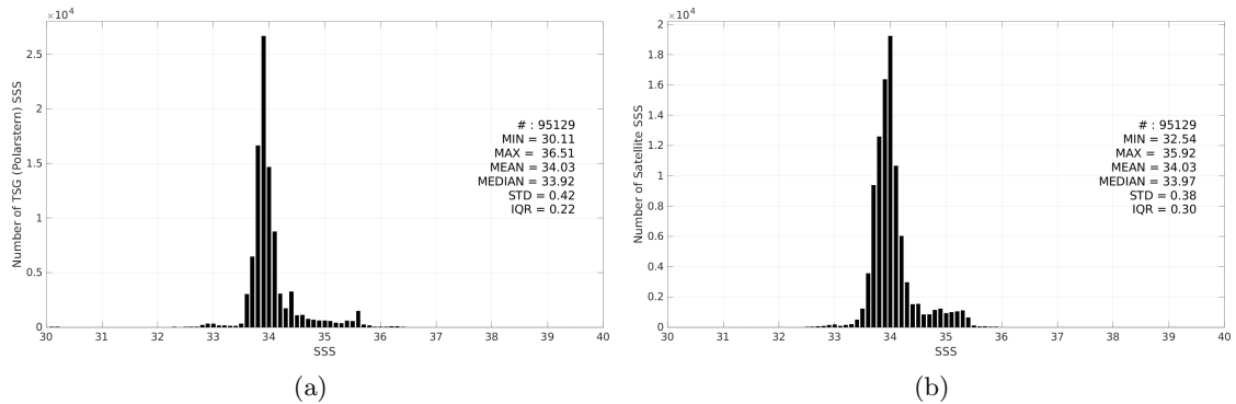
Figure 2: Histograms of SSS from TSG (Polarstern) (a) and SMOS SSS L3 v9 - 18 Days (CATDS-CEC-LOCEAN) (b) considering all match-up pairs per bins of 0.1 over the Roaring Forties and Furious Fifties Pi-MEP region and for the full satellite product period.
