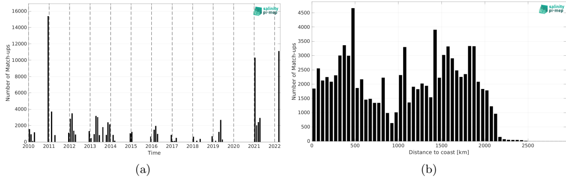
Figure 1: Number of match-ups between TSG (Polarstern) and SMOS SSS L3 v9 - 18 Days (CATDS-CEC-LOCEAN) SSS as a function of time (a) and as function of the distance to coast (b) over the Roaring Forties and Furious Fifties Pi-MEP region and for the full satellite product period.
