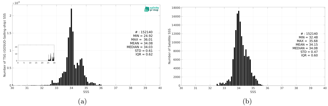
Figure 2: Histograms of SSS from TSG (GOSUD-Sailing-ship) (a) and SMOS SSS L3 v9 - 18 Days (CATDS-CEC-LOCEAN) (b) considering all match-up pairs per bins of 0.1 over the Roaring Forties and Furious Fifties Pi-MEP region and for the full satellite product period.
