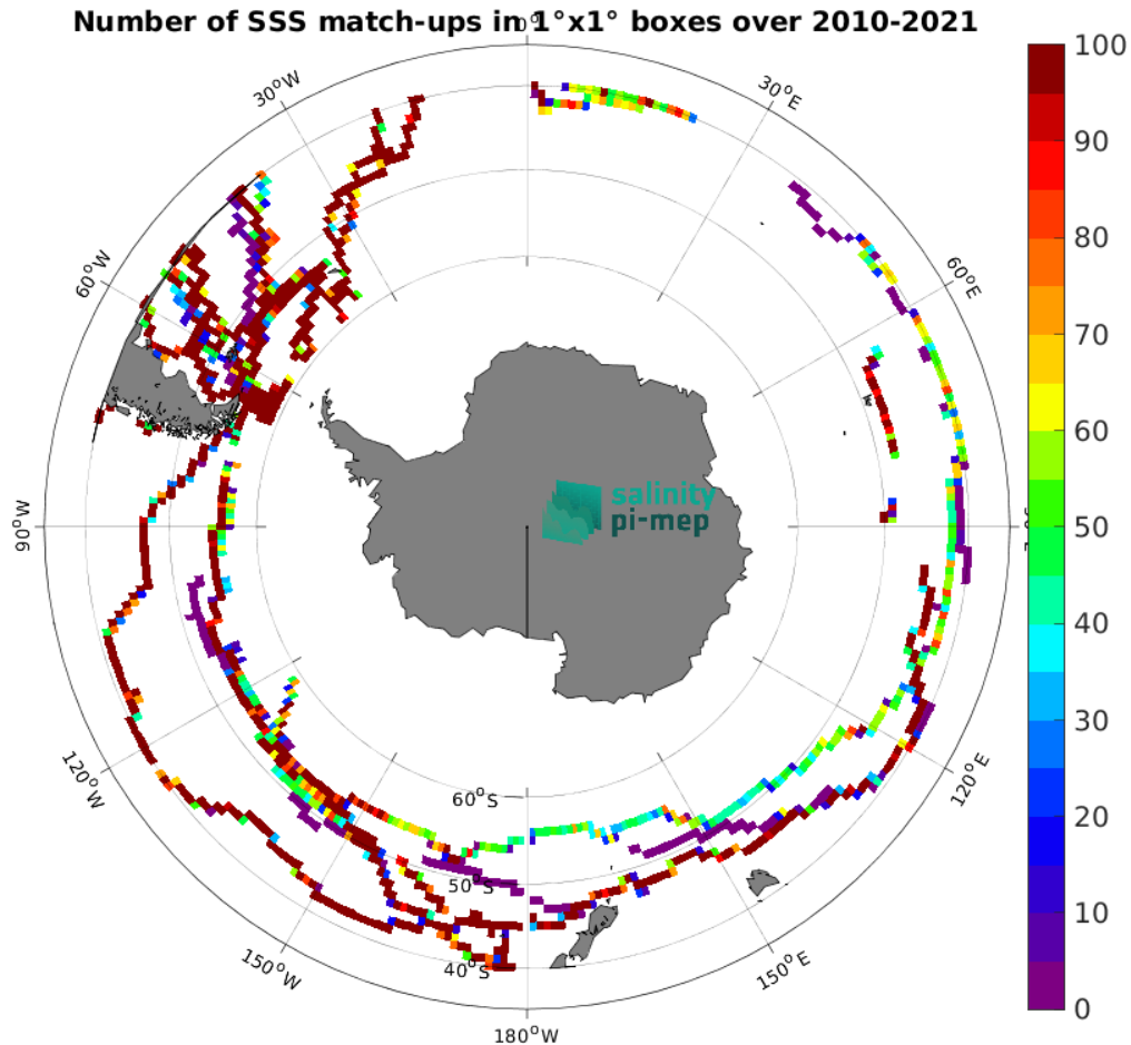
Figure 4: Number of SSS match-ups between TSG (GOSUD-Sailing-ship) SSS and the SMOS SSS L3 v9 - 18 Days (CATDS-CEC-LOCEAN) SSS product for the Roaring Forties and Furious Fifties Pi-MEP region over 1^\circ \times 1^\circ boxes and for the full satellite product period.
