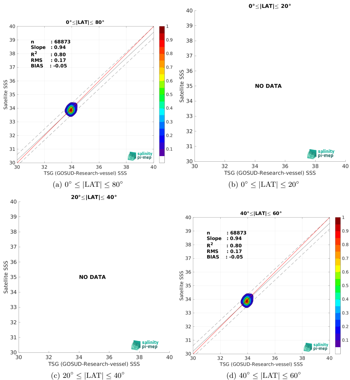
Figure 9: Contour maps of the concentration of SMOS SSS L3 v9 - 18 Days (CATDS-CEC-LOCEAN) SSS (y-axis) versus TSG (GOSUD-Research-vessel) SSS (x-axis) at match-up pairs for different latitude bands. For each plot, the red line shows x=y . The black thin and dashed lines indicate a linear fit through the data cloud and the \pm 95\% confidence levels, respectively. The number match-up pairs n , the slope and R^2 coefficient of the linear fit, the root mean square (RMS) and the mean bias between satellite and in situ data are indicated for each latitude band in each plots.
