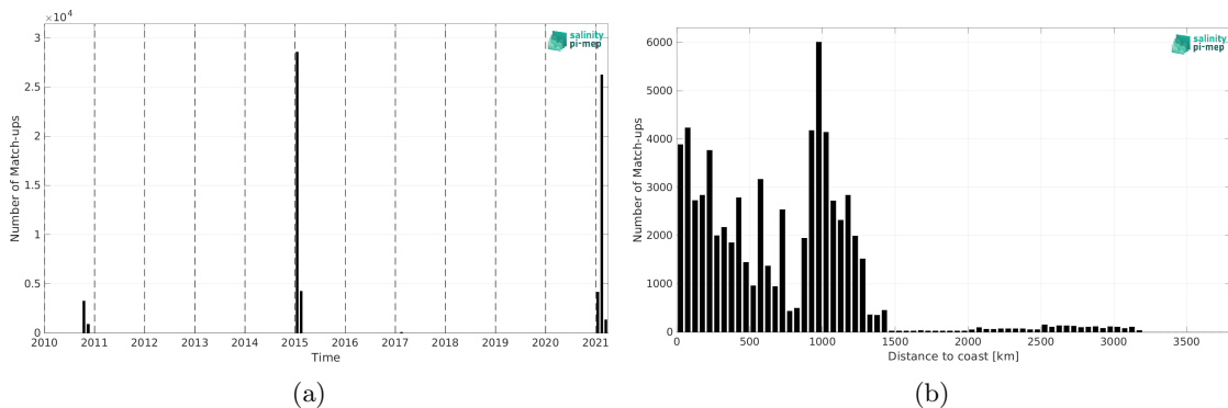
Figure 1: Number of match-ups between TSG (GOSUD-Research-vessel) and SMOS SSS L3 v9 - 18 Days (CATDS-CEC-LOCEAN) SSS as a function of time (a) and as function of the distance to coast (b) over the Roaring Forties and Furious Fifties Pi-MEP region and for the full satellite product period.
