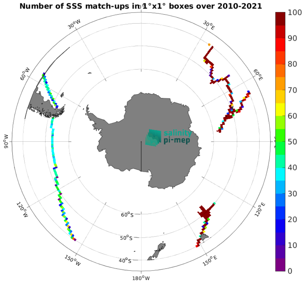
Figure 4: Number of SSS match-ups between TSG (GOSUD-Research-vessel) SSS and the SMOS SSS L3 v9 - 18 Days (CATDS-CEC-LOCEAN) SSS product for the Roaring Forties and Furious Fifties Pi-MEP region over 1^\circ \times 1^\circ boxes and for the full satellite product period.
