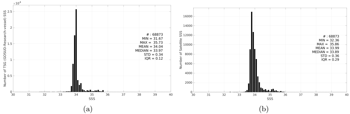
Figure 2: Histograms of SSS from TSG (GOSUD-Research-vessel) (a) and SMOS SSS L3 v9 - 18 Days (CATDS-CEC-LOCEAN) (b) considering all match-up pairs per bins of 0.1 over the Roaring Forties and Furious Fifties Pi-MEP region and for the full satellite product period.
