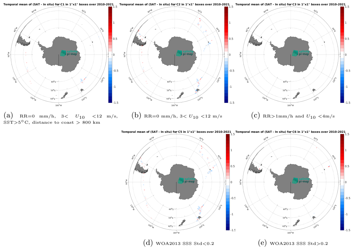
Figure 12: Temporal mean gridded over spatial boxes of size 1^\circ \times 1^\circ of \Delta\text{SSS} (SMOS SSS L3 v9 - 18 Days (CATDS-CEC-LOCEAN) - TSG (GOSUD-Research-vessel)) for 5 different subdatasets corresponding to: RR=0 mm/h, 3 < U_{10} < 12 m/s, SST > 5^\circ\text{C} , distance to coast > 800 km (a), RR=0 mm/h, 3 < U_{10} < 12 m/s (b), RR > 1 mm/h and U_{10} < 4 m/s (c), WOA2013 SSS Std < 0.2 (d), WOA2013 SSS Std > 0.2 (e).
