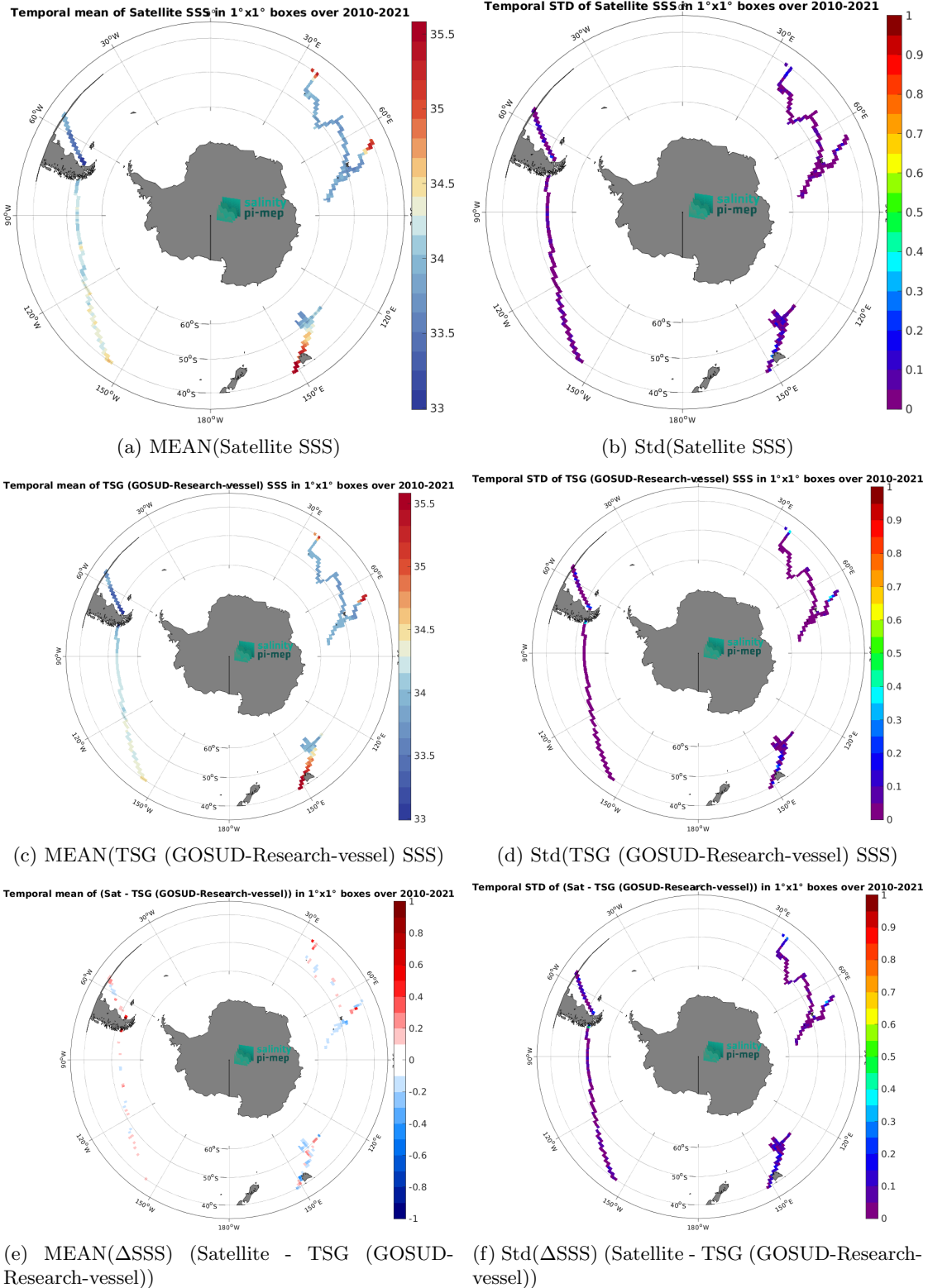
Figure 6: Temporal mean (left) and Std (right) of SSS from SMOS SSS L3 v9 - 18 Days (CATDS-CEC-LOCEAN) (top), TSG (GOSUD-Research-vessel) (middle), and of \Delta SSS (Satellite - TSG (GOSUD-Research-vessel)). Only match-up pairs are used to generate these maps.
