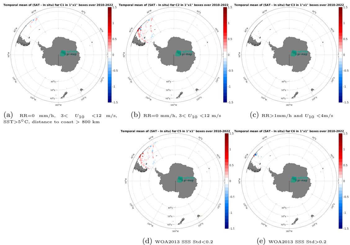
Figure 14: Temporal mean gridded over spatial boxes of size 1^\circ \times 1^\circ of \Delta SSS (SMOS SSS L3 v9 - 18 Days (CATDS-CEC-LOCEAN) - TSG (CSIC-UTM)) for 5 different subdatasets corresponding to:RR=0 mm/h, 3 < U_{10} < 12 m/s, SST >5^\circ C, distance to coast > 800 km (a), RR=0 mm/h, 3 < U_{10} < 12 m/s (b), RR >1 mm/h and U_{10} < 4 m/s (c), WOA2013 SSS Std <0.2 (d), WOA2013 SSS Std >0.2 (e).
