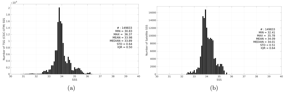
Figure 3: Histograms of SSS from TSG (CSIC-UTM) (a) and SMOS SSS L3 v9 - 18 Days (CATDS-CEC-LOCEAN) (b) considering all match-up pairs per bins of 0.1 over the Roaring Forties and Furious Fifties Pi-MEP region and for the full satellite product period.
