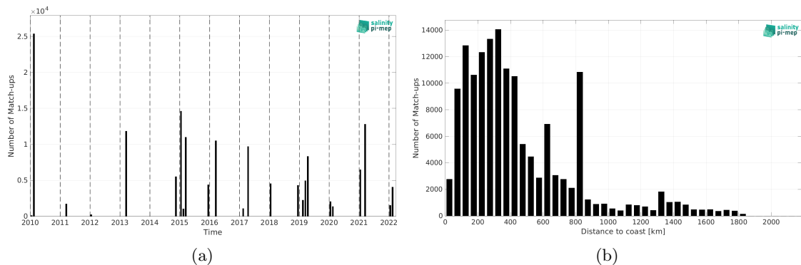
Figure 2: Number of match-ups between TSG (CSIC-UTM) and SMOS SSS L3 v9 - 18 Days (CATDS-CEC-LOCEAN) SSS as a function of time (a) and as function of the distance to coast (b) over the Roaring Forties and Furious Fifties Pi-MEP region and for the full satellite product period.
