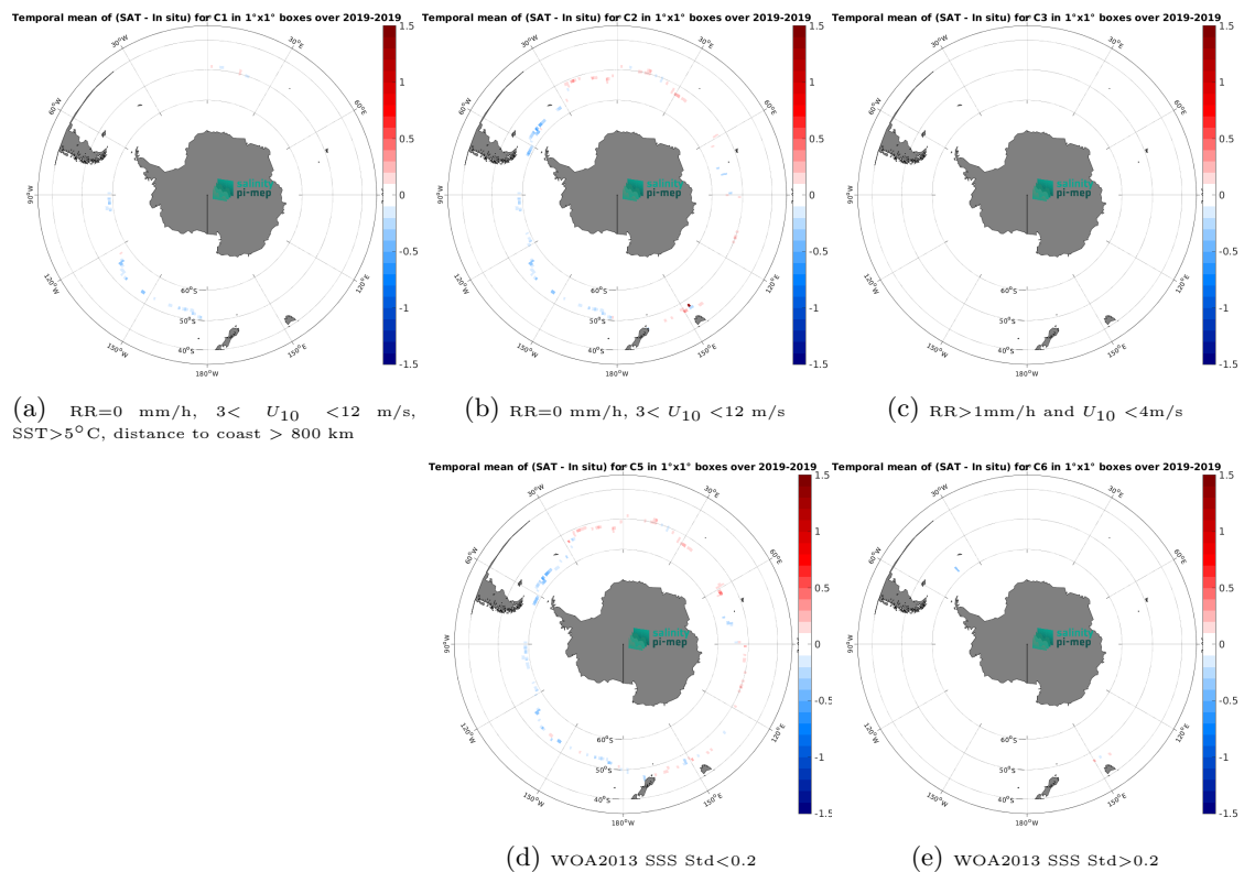
Figure 14: Temporal mean gridded over spatial boxes of size 1^\circ \times 1^\circ of \Delta SSS (SMOS SSS L3 v9 - 18 Days (CATDS-CEC-LOCEAN) - Sailability) for 5 different subdatasets corresponding to: RR=0 mm/h, 3 < U_{10} < 12 m/s, SST > 5°C, distance to coast > 800 km (a), RR=0 mm/h, 3 < U_{10} < 12 m/s (b), RR > 1mm/h and U_{10} < 4 m/s (c), WOA2013 SSS Std < 0.2 (d), WOA2013 SSS Std > 0.2 (e).
