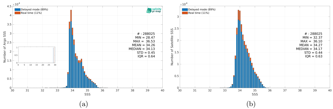
Figure 2: Histograms of SSS from Argo (a) and SMOS SSS L3 v9 - 18 Days (CATDS-CEC-LOCEAN) (b) considering all match-up pairs per bins of 0.1 over the Roaring Forties and Furious Fifties Pi-MEP region and for the full satellite product period.
