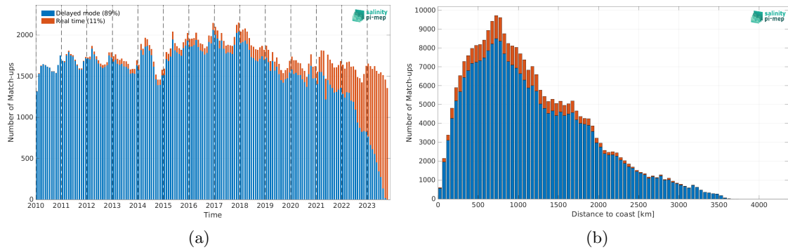
Figure 1: Number of match-ups between Argo and SMOS SSS L3 v9 - 18 Days (CATDS-CEC-LOCEAN) SSS as a function of time (a) and as function of the distance to coast (b) over the Roaring Forties and Furious Fifties Pi-MEP region and for the full satellite product period.
