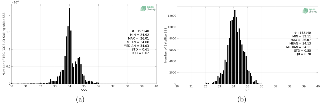
Figure 2: Histograms of SSS from TSG (GOSUD-Sailing-ship) (a) and SMOS SSS L3 v8 - 9 Days (CATDS-CECOS-LOCEAN) (b) considering all match-up pairs per bins of 0.1 over the Roaring Forties and Furious Fifties Pi-MEP region and for the full satellite product period.
