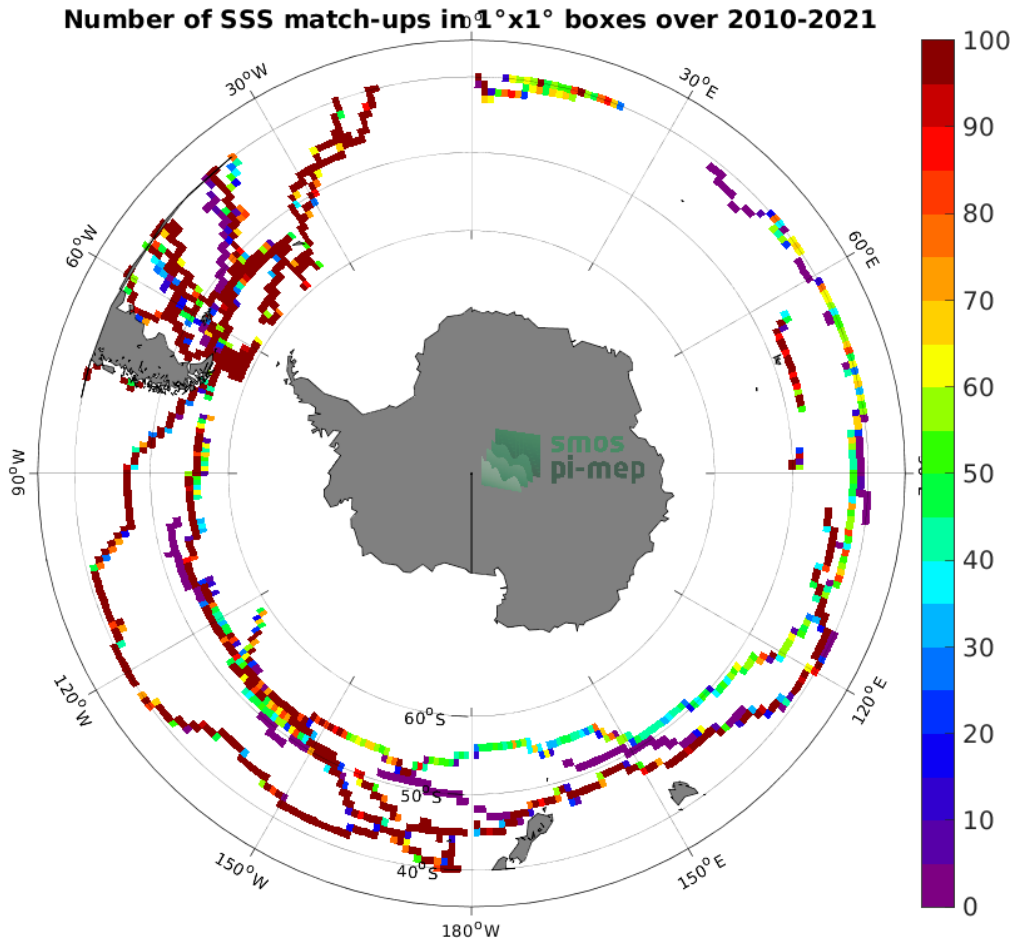
Figure 4: Number of SSS match-ups between TSG (GOSUD-Sailing-ship) SSS and the SMOS SSS L3 v8 - 9 Days (CATDS-CECOS-LOCEAN) SSS product for the Roaring Forties and Furious Fifties Pi-MEP region over 1^\circ \times 1^\circ boxes and for the full satellite product period.
