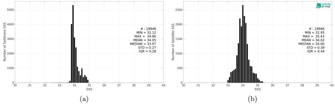
Figure 2: Histograms of SSS from Saildrone (a) and SMOS SSS L3 v8 - 9 Days (CATDS-CEC-LOCEAN) (b) considering all match-up pairs per bins of 0.1 over the Roaring Forties and Furious Fifties Pi-MEP region and for the full satellite product period.
