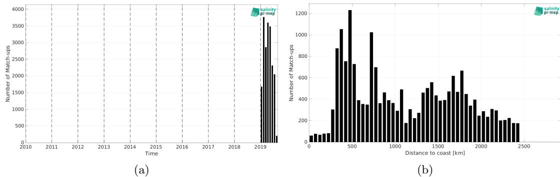
Figure 1: Number of match-ups between Saildrone and SMOS SSS L3 v8 - 9 Days (CATDS-CEC-LOCEAN) SSS as a function of time (a) and as function of the distance to coast (b) over the Roaring Forties and Furious Fifties Pi-MEP region and for the full satellite product period.
