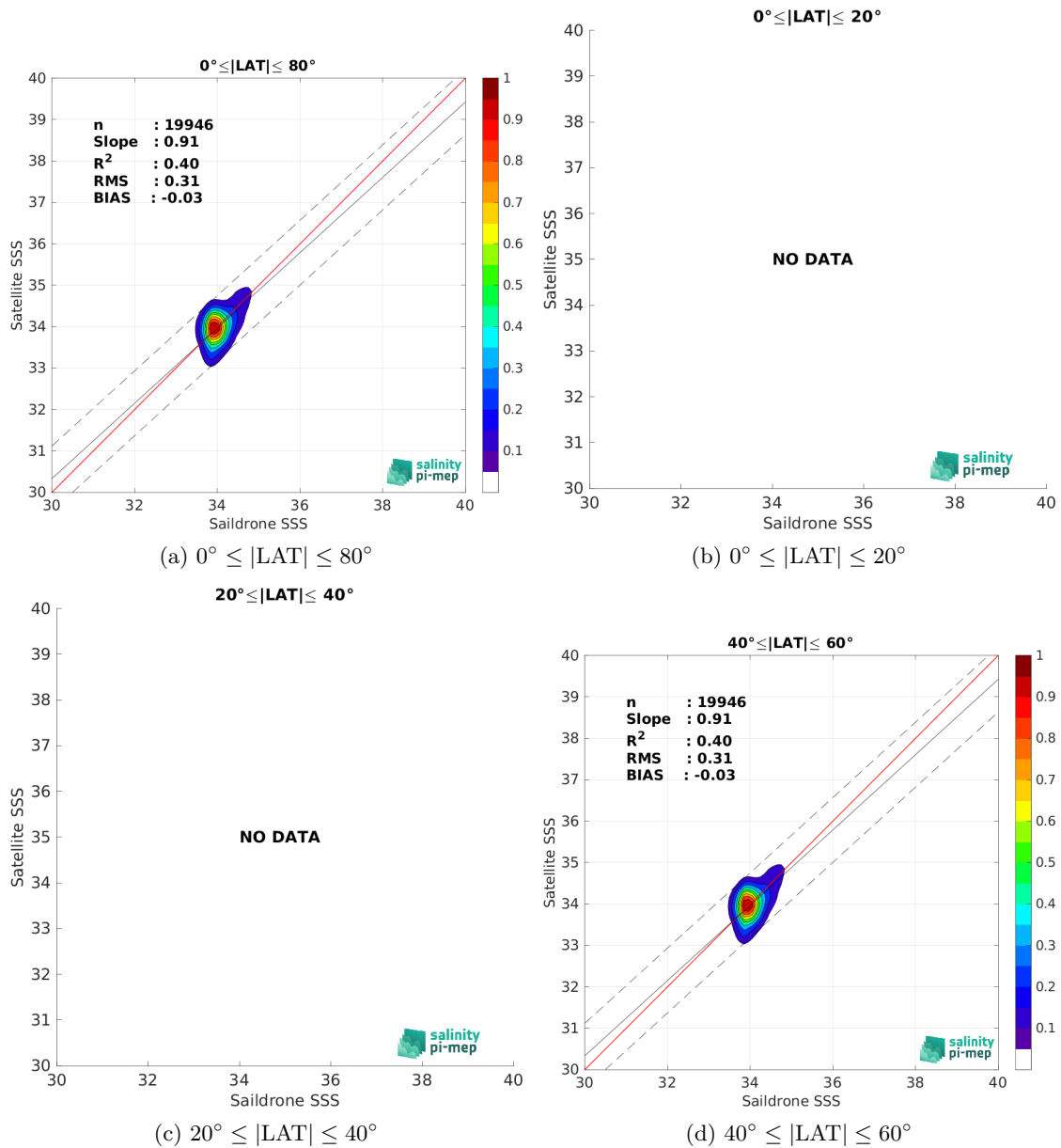
Figure 9: Contour maps of the concentration of SMOS SSS L3 v8 - 9 Days (CATDS-CEC-LOCEAN) SSS (y-axis) versus Sairdrone SSS (x-axis) at match-up pairs for different latitude bands. For each plot, the red line shows x=y . The black thin and dashed lines indicate a linear fit through the data cloud and the \pm 95\% confidence levels, respectively. The number match-up pairs n , the slope and R^2 coefficient of the linear fit, the root mean square (RMS) and the mean bias between satellite and in situ data are indicated for each latitude band in each plots.
