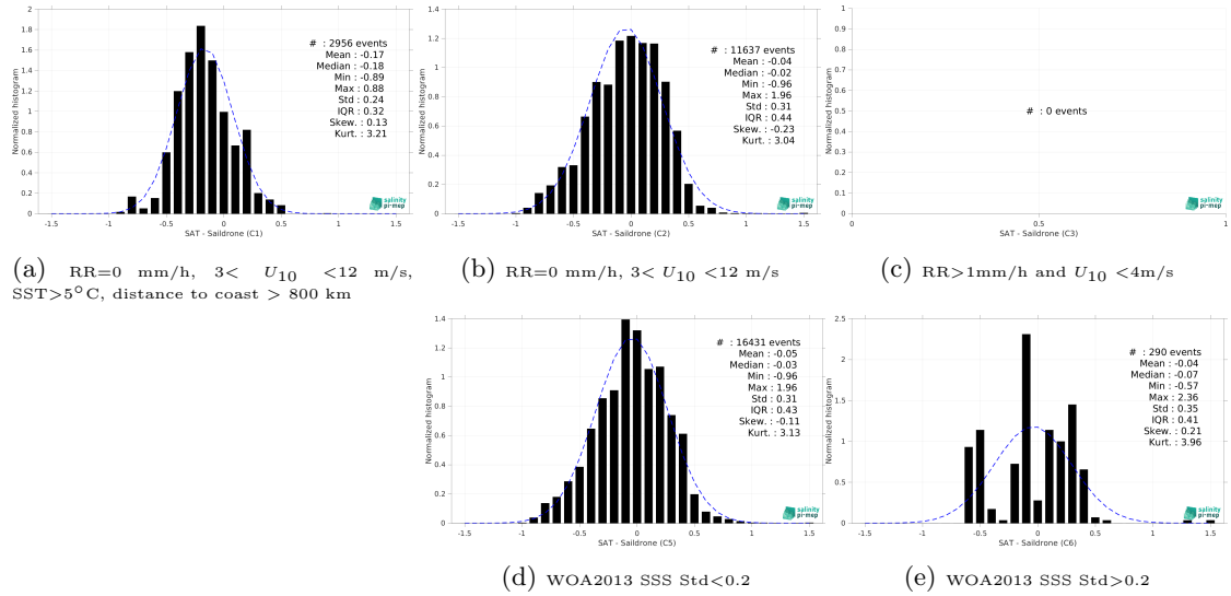
Figure 13: Normalized histogram of \Delta SSS (SMOS SSS L3 v8 - 9 Days (CATDS-CEC-LOCEAN) - Saildrone) for 5 different subdatasets corresponding to: RR=0 mm/h, 3 < U_{10} < 12 m/s, SST>5°C, distance to coast > 800 km (a), RR=0 mm/h, 3 < U_{10} < 12 m/s (b), RR>1mm/h and U_{10} < 4 m/s (c), WOA2013 SSS Std<0.2 (d), WOA2013 SSS Std>0.2 (e).
