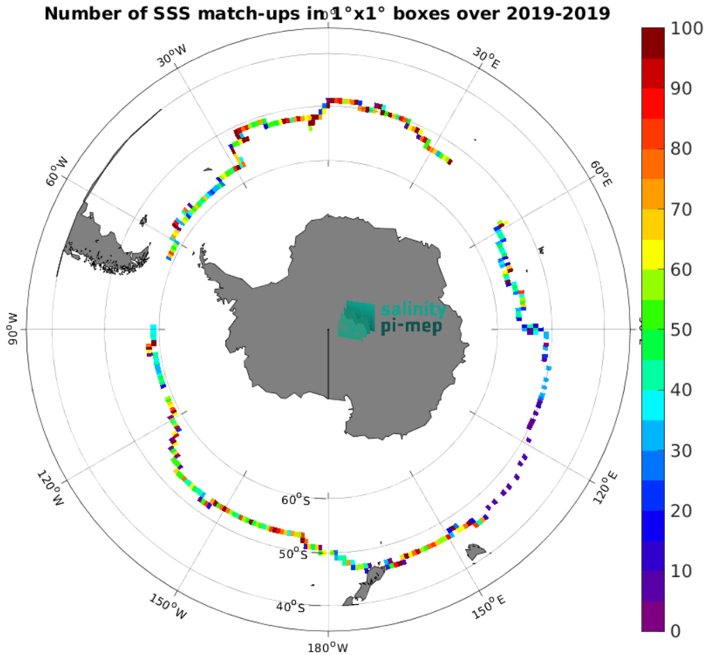
Figure 4: Number of SSS match-ups between Saildrone SSS and the SMOS SSS L3 v8 - 9 Days (CATDS-CEC-LOCEAN) SSS product for the Roaring Forties and Furious Fifties Pi-MEP region over 1^\circ \times 1^\circ boxes and for the full satellite product period.
