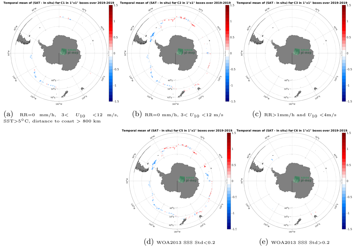
Figure 12: Temporal mean gridded over spatial boxes of size 1^{\circ}\times 1^{\circ} of \Delta\text{SSS} (SMOS SSS L3 v8 - 9 Days (CATDS-CECOS-LOCEAN) - Saildrone) for 5 different subdatasets corresponding to:RR=0 mm/h, 3 < U_{10} < 12 m/s, SST >5^{\circ}\text{C} , distance to coast > 800 km (a), RR=0 mm/h, 3 < U_{10} < 12 m/s (b), RR >1 mm/h and U_{10} < 4 m/s (c), WOA2013 SSS Std <0.2 (d), WOA2013 SSS Std >0.2 (e).
