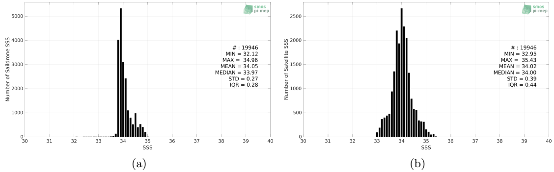
Figure 2: Histograms of SSS from Saildrone (a) and SMOS SSS L3 v8 - 9 Days (CATDS-CECOS-LOCEAN) (b) considering all match-up pairs per bins of 0.1 over the Roaring Forties and Furious Fifties Pi-MEP region and for the full satellite product period.
