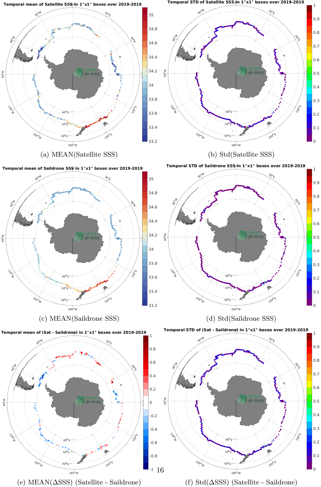
Figure 6: Temporal mean (left) and Std (right) of SSS from SMOS SSS L3 v8 - 9 Days (CATDS-CECOS-LOCEAN) (top), Saildrone (middle), and of \Delta SSS (Satellite - Saildrone). Only match-up pairs are used to generate these maps.
