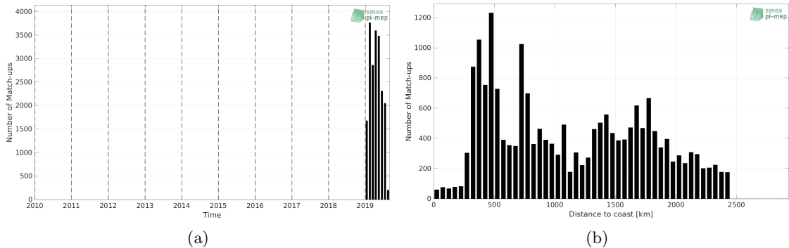
Figure 1: Number of match-ups between Saildrone and SMOS SSS L3 v8 - 9 Days (CATDS-CECOS-LOCEAN) SSS as a function of time (a) and as function of the distance to coast (b) over the Roaring Forties and Furious Fifties Pi-MEP region and for the full satellite product period.
