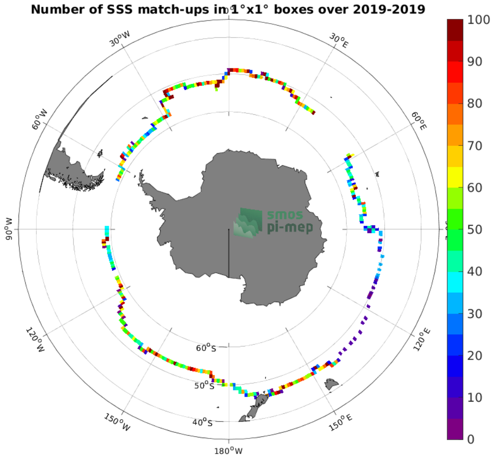
Figure 4: Number of SSS match-ups between Saildrone SSS and the SMOS SSS L3 v8 - 9 Days (CATDS-CECOS-LOCEAN) SSS product for the Roaring Forties and Furious Fifties Pi-MEP region over 1^\circ \times 1^\circ boxes and for the full satellite product period.
