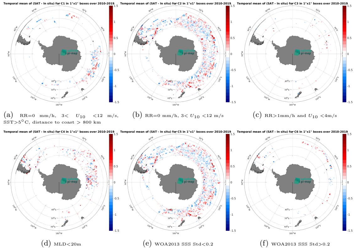
Figure 12: Temporal mean gridded over spatial boxes of size 1^{\circ}\times 1^{\circ} of \Delta\text{SSS} (SMOS SSS L3 v8 - 9 Days (CATDS-CEC-LOCEAN) - Marine mammals) for 6 different subdatasets corresponding to:RR=0 mm/h, 3 < U_{10} < 12 m/s, SST >5^{\circ}\text{C} , distance to coast > 800 km (a), RR=0 mm/h, 3 < U_{10} < 12 m/s (b), RR >1 mm/h and U_{10} < 4 m/s (c),MLD <20 m (d),WOA2013 SSS Std <0.2 (e),WOA2013 SSS Std >0.2 (f).
