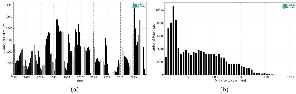
Figure 1: Number of match-ups between Marine mammals and SMOS SSS L3 v8 - 9 Days (CATDS-CEC-LOCEAN) SSS as a function of time (a) and as function of the distance to coast (b) over the Roaring Forties and Furious Fifties Pi-MEP region and for the full satellite product period.
