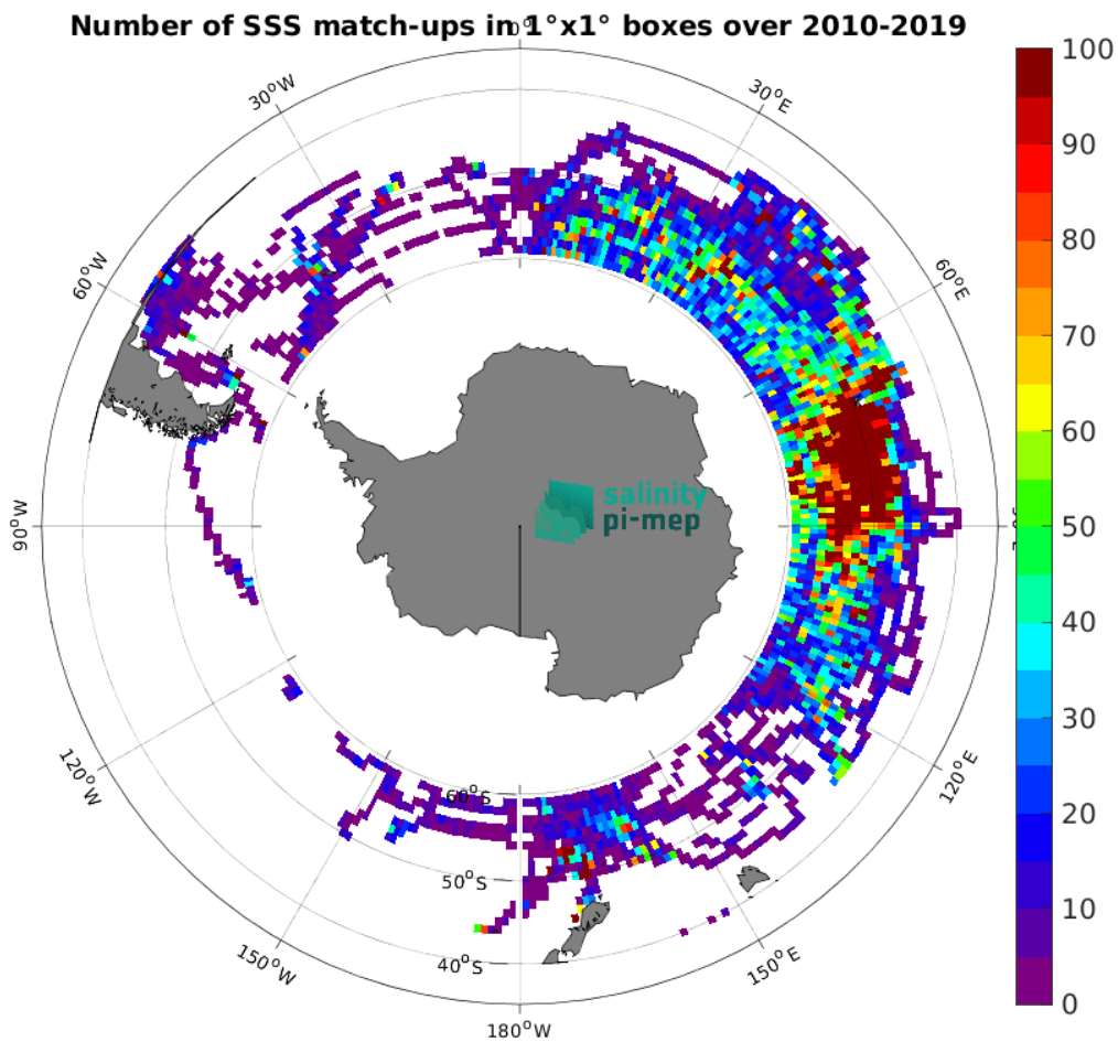
Figure 4: Number of SSS match-ups between Marine mammals SSS and the SMOS SSS L3 v8 - 9 Days (CATDS-CEC-LOCEAN) SSS product for the Roaring Forties and Furious Fifties Pi-MEP region over 1^\circ \times 1^\circ boxes and for the full satellite product period.
