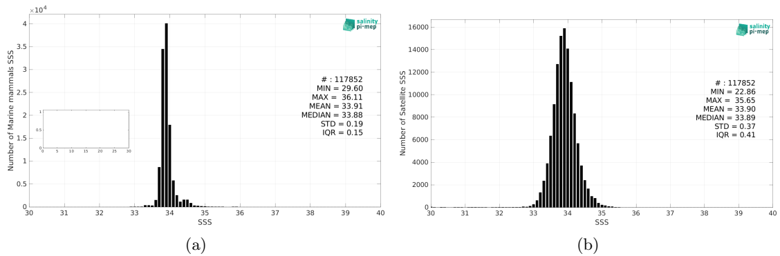
Figure 2: Histograms of SSS from Marine mammals (a) and SMOS SSS L3 v8 - 9 Days (CATDS-CEC-LOCEAN) (b) considering all match-up pairs per bins of 0.1 over the Roaring Forties and Furious Fifties Pi-MEP region and for the full satellite product period.
