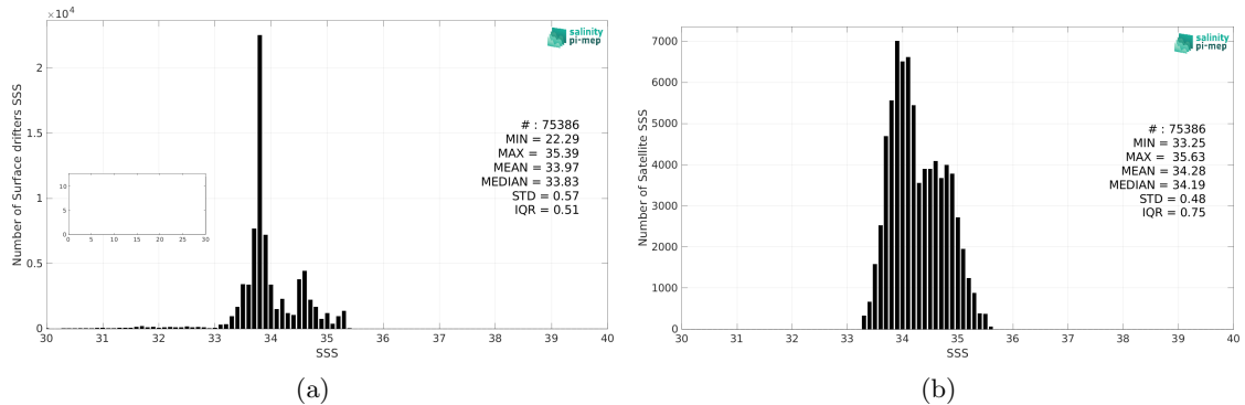
Figure 2: Histograms of SSS from Surface drifters (a) and SMOS SSS L3 v8 - 9 Days (CATDS-CEC-LOCEAN) (b) considering all match-up pairs per bins of 0.1 over the Roaring Forties and Furious Fifties Pi-MEP region and for the full satellite product period.
