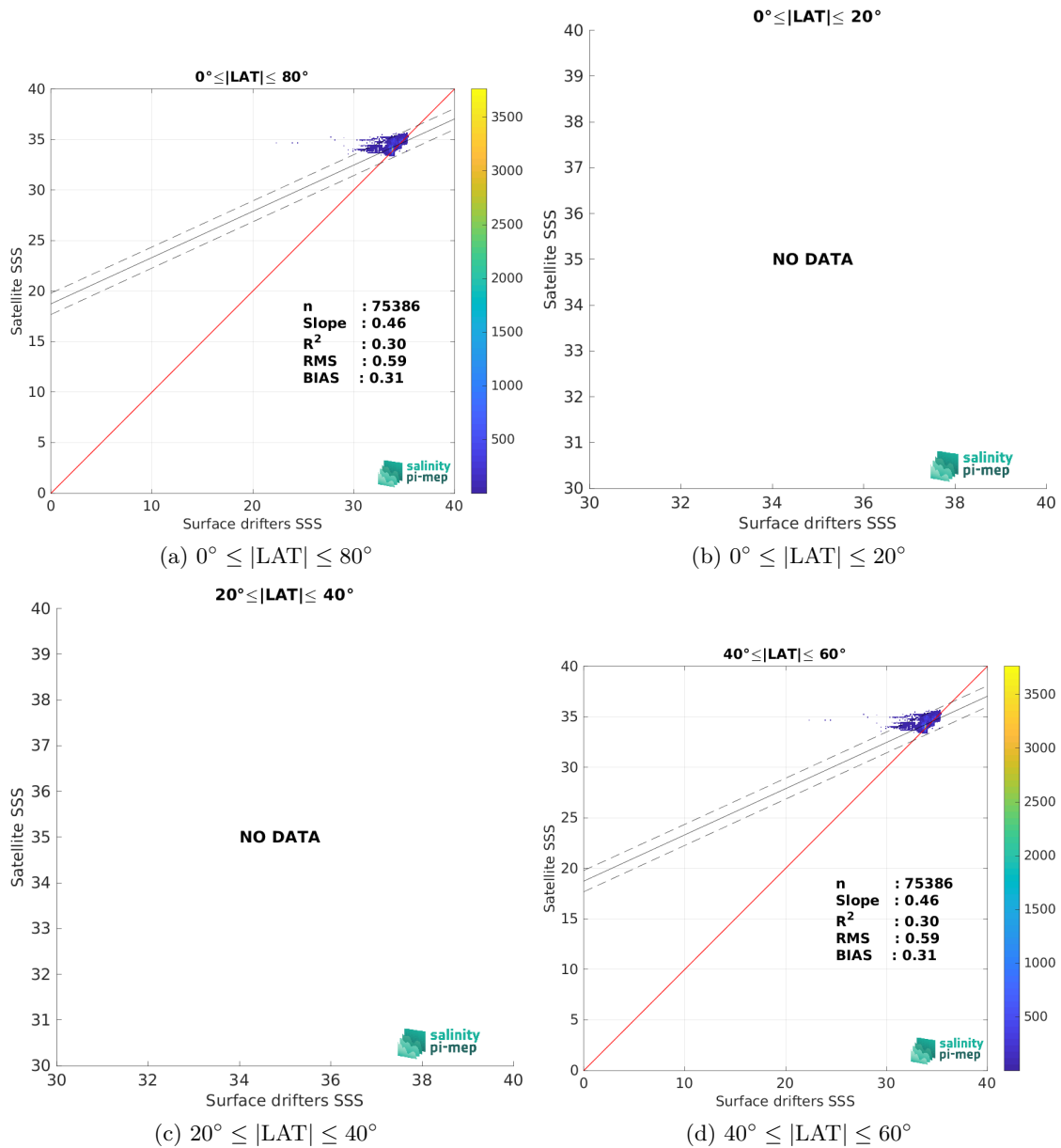
Figure 8: Contour maps of the concentration of SMOS SSS L3 v8 - 9 Days (CATDS-CEC-LOCEAN) SSS (y-axis) versus Surface drifters SSS (x-axis) at match-up pairs for different latitude bands. For each plot, the red line shows x=y . The black thin and dashed lines indicate a linear fit through the data cloud and the \pm 95\% confidence levels, respectively. The number match-up pairs n , the slope and R^2 coefficient of the linear fit, the root mean square (RMS) and the mean bias between satellite and in situ data are indicated for each latitude band in each plots.
