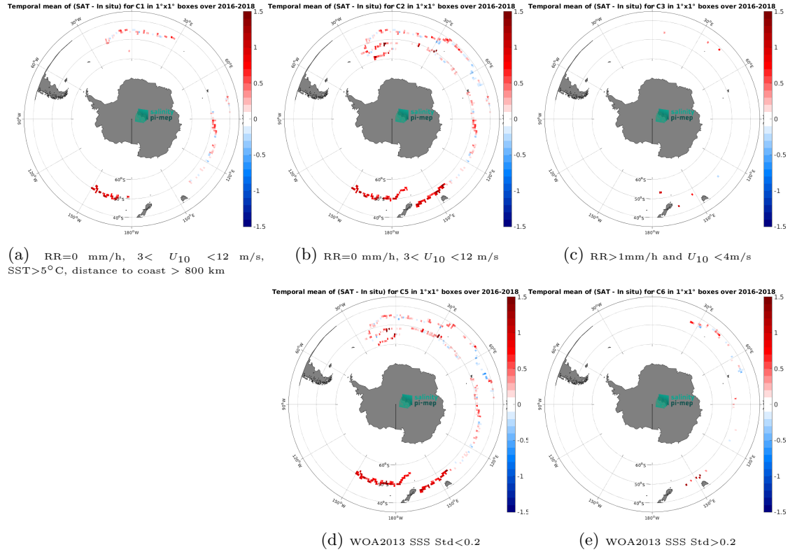
Figure 11: Temporal mean gridded over spatial boxes of size 1^{\circ}\times 1^{\circ} of \Delta\text{SSS} (SMOS SSS L3 v8 - 9 Days (CATDS-CEC-LOCEAN) - Surface drifters) for 5 different subdatasets corresponding to:RR=0 mm/h, 3 < U_{10} < 12 m/s, SST >5^{\circ}\text{C} , distance to coast > 800 km (a), RR=0 mm/h, 3 < U_{10} < 12 m/s (b), RR >1 mm/h and U_{10} < 4 m/s (c), WOA2013 SSS Std <0.2 (d), WOA2013 SSS Std >0.2 (e).
