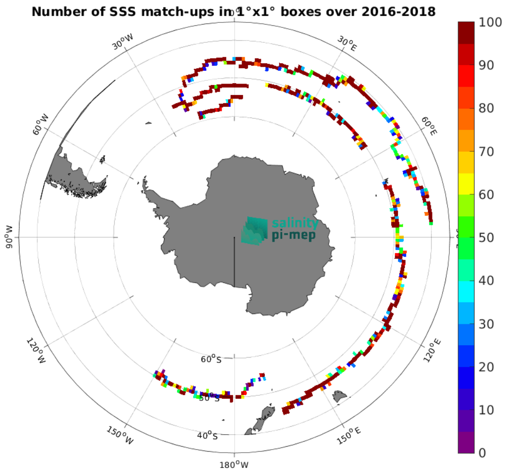
Figure 3: Number of SSS match-ups between Surface drifters SSS and the SMOS SSS L3 v8 - 9 Days (CATDS-CEC-LOCEAN) SSS product for the Roaring Forties and Furious Fifties Pi-MEP region over 1^\circ \times 1^\circ boxes and for the full satellite product period.
