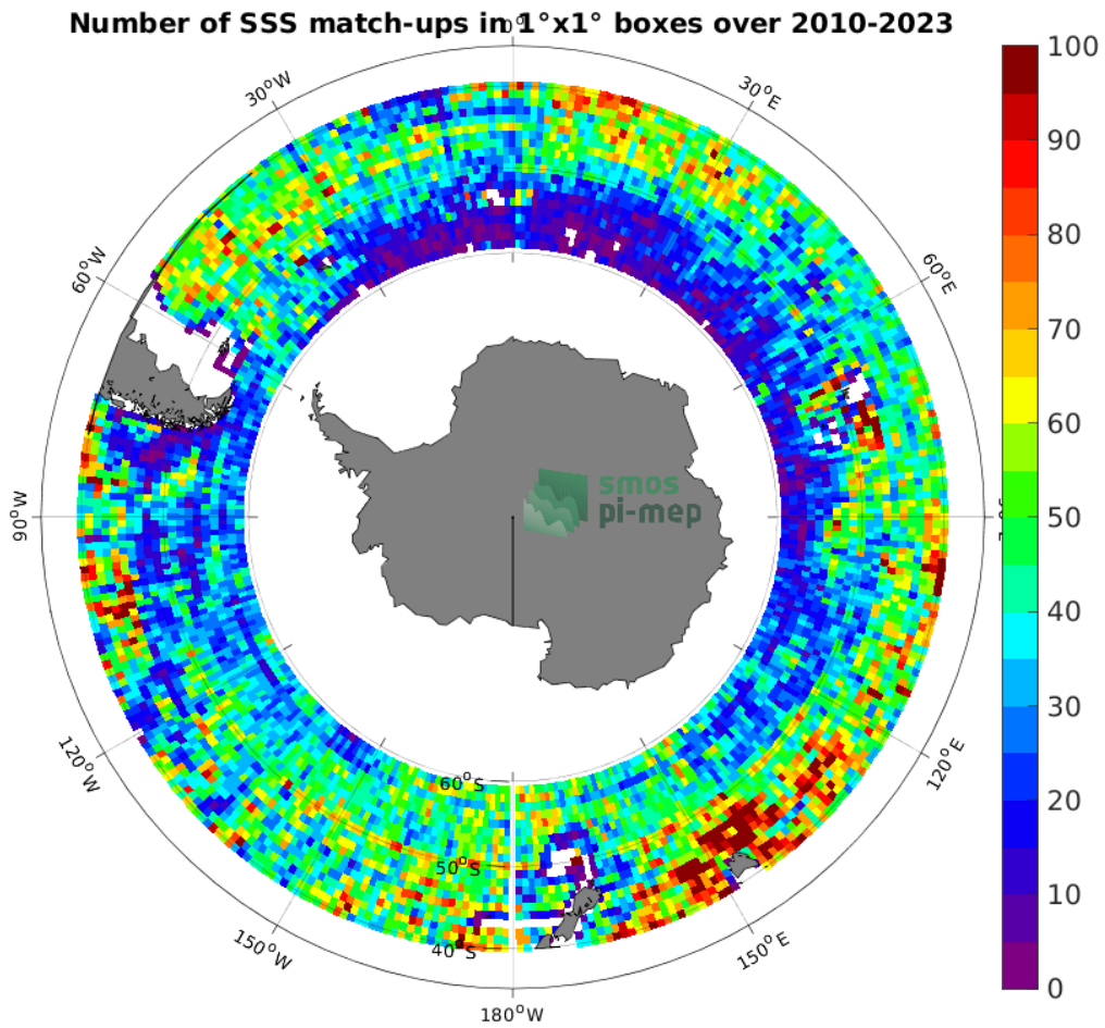
Figure 4: Number of SSS match-ups between Argo SSS and the SMOS SSS L3 v8 - 9 Days (CATDS-CECOS-LOCEAN) SSS product for the Roaring Forties and Furious Fifties Pi-MEP region over 1^\circ \times 1^\circ boxes and for the full satellite product period.
