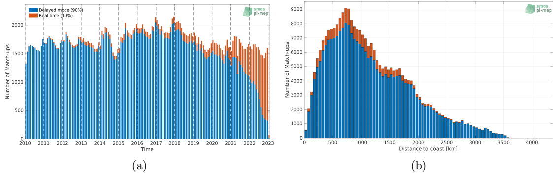
Figure 1: Number of match-ups between Argo and SMOS SSS L3 v8 - 9 Days (CATDS-CECOS-LOCEAN) SSS as a function of time (a) and as function of the distance to coast (b) over the Roaring Forties and Furious Fifties Pi-MEP region and for the full satellite product period.
