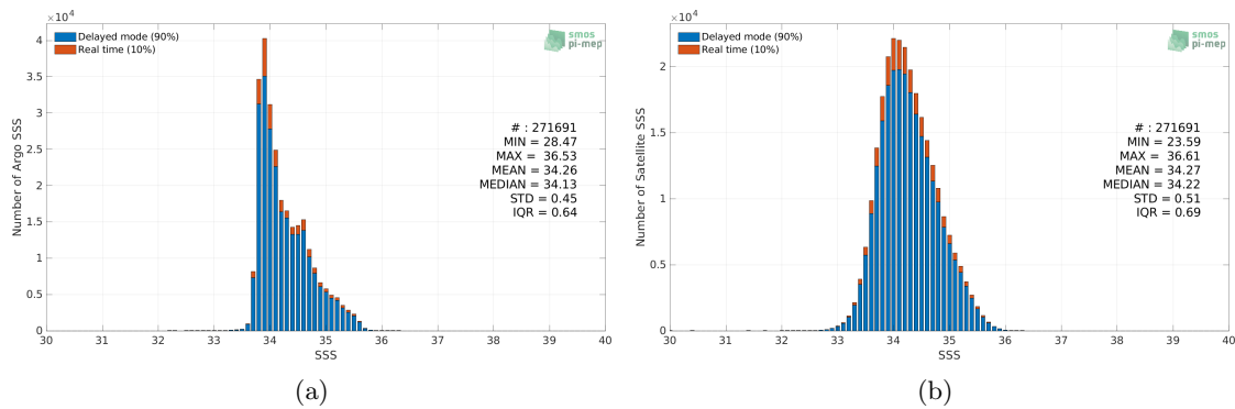
Figure 2: Histograms of SSS from Argo (a) and SMOS SSS L3 v8 - 9 Days (CATDS-CECOS-LOCEAN) (b) considering all match-up pairs per bins of 0.1 over the Roaring Forties and Furious Fifties Pi-MEP region and for the full satellite product period.
