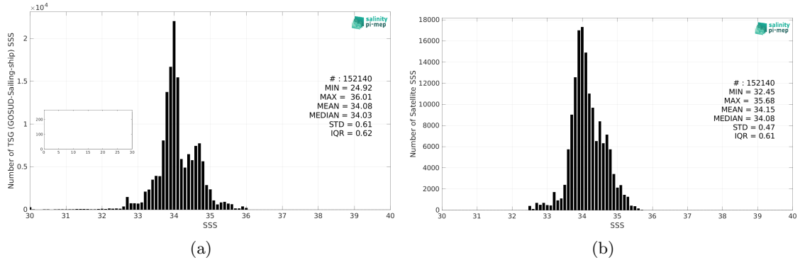
Figure 2: Histograms of SSS from TSG (GOSUD-Sailing-ship) (a) and SMOS SSS L3 v8 - 18 Days (CATDS-CEC-LOCEAN) (b) considering all match-up pairs per bins of 0.1 over the Roaring Forties and Furious Fifties Pi-MEP region and for the full satellite product period.
