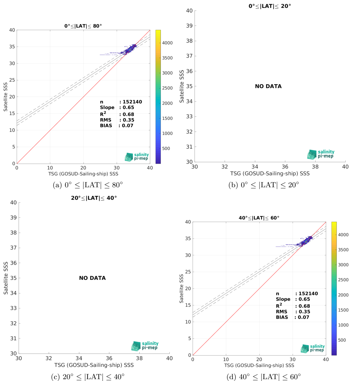
Figure 9: Contour maps of the concentration of SMOS SSS L3 v8 - 18 Days (CATDS-CEC-LOCEAN) SSS (y-axis) versus TSG (GOSUD-Sailing-ship) SSS (x-axis) at match-up pairs for different latitude bands. For each plot, the red line shows x=y . The black thin and dashed lines indicate a linear fit through the data cloud and the \pm 95\% confidence levels, respectively. The number match-up pairs n , the slope and R^2 coefficient of the linear fit, the root mean square (RMS) and the mean bias between satellite and in situ data are indicated for each latitude band in each plots.
