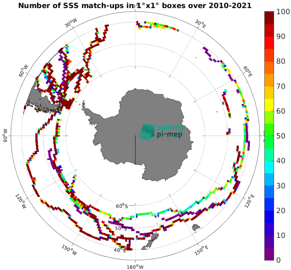
Figure 4: Number of SSS match-ups between TSG (GOSUD-Sailing-ship) SSS and the SMOS SSS L3 v8 - 18 Days (CATDS-CEC-LOCEAN) SSS product for the Roaring Forties and Furious Fifties Pi-MEP region over 1^\circ \times 1^\circ boxes and for the full satellite product period.
