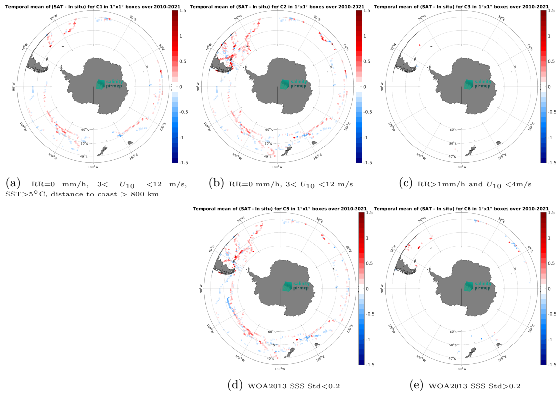
Figure 12: Temporal mean gridded over spatial boxes of size 1^\circ \times 1^\circ of \Delta SSS (SMOS SSS L3 v8 - 18 Days (CATDS-CEC-LOCEAN) - TSG (GOSUD-Sailing-ship)) for 5 different subdatasets corresponding to:RR=0 mm/h, 3 < U_{10} < 12 m/s, SST>5°C, distance to coast > 800 km (a), RR=0 mm/h, 3 < U_{10} < 12 m/s (b), RR>1mm/h and U_{10} < 4 m/s (c), WOA2013 SSS Std<0.2 (d), WOA2013 SSS Std>0.2 (e).
