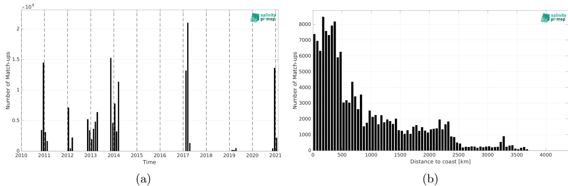
Figure 1: Number of match-ups between TSG (GOSUD-Sailing-ship) and SMOS SSS L3 v8 - 18 Days (CATDS-CEC-LOCEAN) SSS as a function of time (a) and as function of the distance to coast (b) over the Roaring Forties and Furious Fifties Pi-MEP region and for the full satellite product period.
