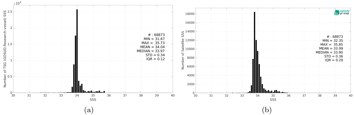
Figure 2: Histograms of SSS from TSG (GOSUD-Research-vessel) (a) and SMOS SSS L3 v8 - 18 Days (CATDS-CEC-LOCEAN) (b) considering all match-up pairs per bins of 0.1 over the Roaring Forties and Furious Fifties Pi-MEP region and for the full satellite product period.
