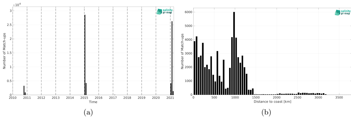
Figure 1: Number of match-ups between TSG (GOSUD-Research-vessel) and SMOS SSS L3 v8 - 18 Days (CATDS-CEC-LOCEAN) SSS as a function of time (a) and as function of the distance to coast (b) over the Roaring Forties and Furious Fifties Pi-MEP region and for the full satellite product period.
