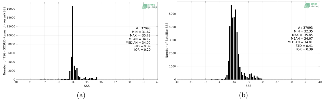
Figure 2: Histograms of SSS from TSG (GOSUD-Research-vessel) (a) and SMOS SSS L3 v8 - 18 Days (CATDS-CECOS-LOCEAN) (b) considering all match-up pairs per bins of 0.1 over the Roaring Forties and Furious Fifties Pi-MEP region and for the full satellite product period.
