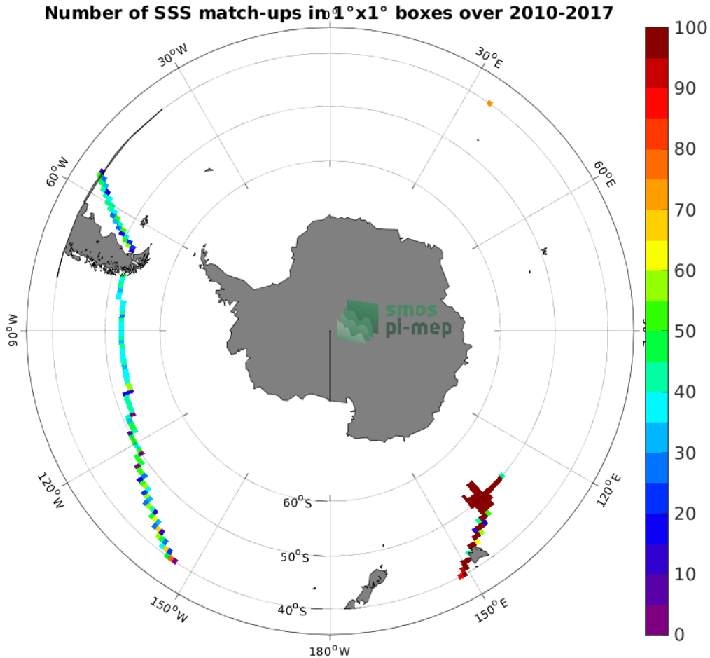
Figure 4: Number of SSS match-ups between TSG (GOSUD-Research-vessel) SSS and the SMOS SSS L3 v8 - 18 Days (CATDS-CECOS-LOCEAN) SSS product for the Roaring Forties and Furious Fifties Pi-MEP region over 1^\circ \times 1^\circ boxes and for the full satellite product period.
