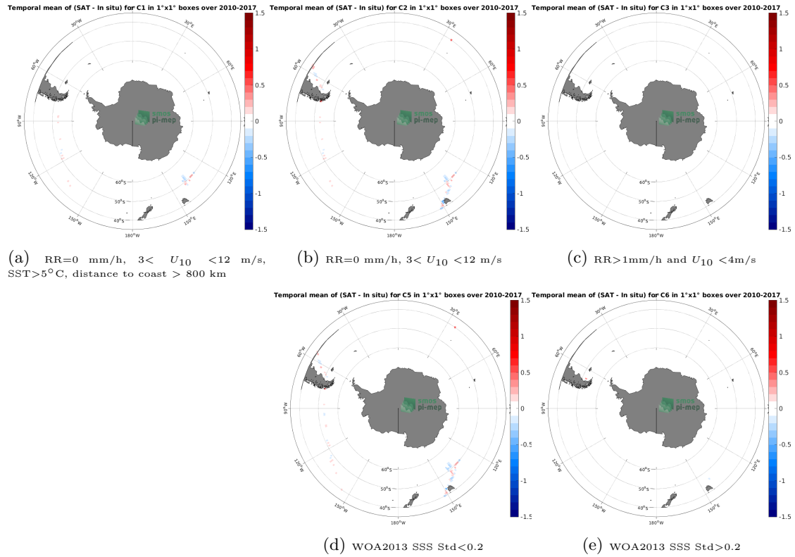
Figure 12: Temporal mean gridded over spatial boxes of size 1^\circ \times 1^\circ of \Delta\text{SSS} (SMOS SSS L3 v8 - 18 Days (CATDS-CECOS-LOCEAN) - TSG (GOSUD-Research-vessel)) for 5 different sub-datasets corresponding to: RR=0 mm/h, 3 < U_{10} < 12 m/s, SST > 5^\circ\text{C} , distance to coast > 800 km (a), RR=0 mm/h, 3 < U_{10} < 12 m/s (b), RR > 1 mm/h and U_{10} < 4 m/s (c), WOA2013 SSS Std < 0.2 (d), WOA2013 SSS Std > 0.2 (e).
