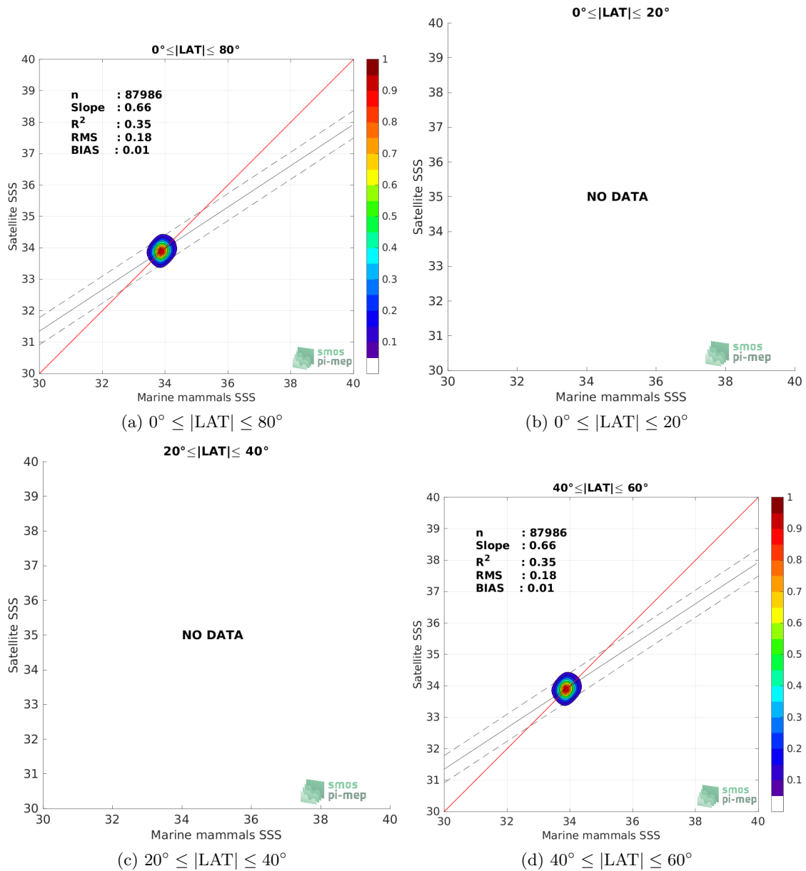
Figure 9: Contour maps of the concentration of SMOS SSS L3 v8 - 18 Days (CATDS-CECOS-LOCEAN) SSS (y-axis) versus Marine mammals SSS (x-axis) at match-up pairs for different latitude bands. For each plot, the red line shows x=y . The black thin and dashed lines indicate a linear fit through the data cloud and the \pm 95\% confidence levels, respectively. The number match-up pairs n , the slope and R^2 coefficient of the linear fit, the root mean square (RMS) and the mean bias between satellite and in situ data are indicated for each latitude band in each plots.
