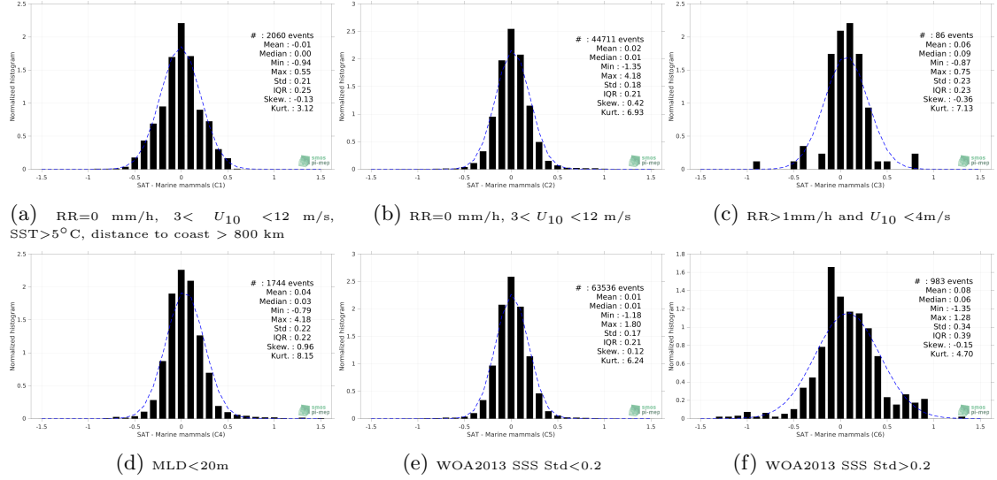
Figure 13: Normalized histogram of \Delta SSS (SMOS SSS L3 v8 - 18 Days (CATDS-CECOS-LOCEAN) - Marine mammals) for 6 different subdatasets corresponding to: RR=0 mm/h, 3 < U_{10} < 12 m/s, SST > 5°C, distance to coast > 800 km (a), RR=0 mm/h, 3 < U_{10} < 12 m/s (b), RR > 1mm/h and U_{10} < 4 m/s (c), MLD < 20m (d), WOA2013 SSS Std < 0.2 (e), WOA2013 SSS Std > 0.2 (f).
