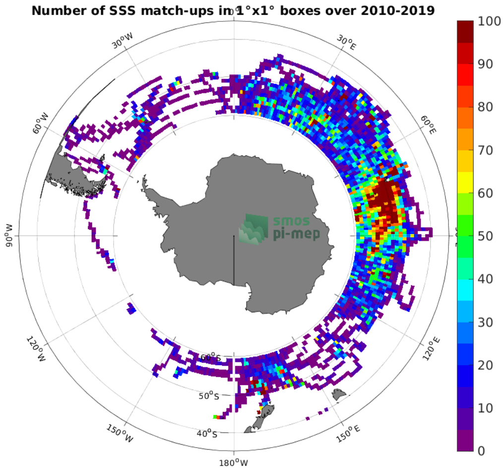
Figure 4: Number of SSS match-ups between Marine mammals SSS and the SMOS SSS L3 v8 - 18 Days (CATDS-CECOS-LOCEAN) SSS product for the Roaring Forties and Furious Fifties Pi-MEP region over 1^\circ \times 1^\circ boxes and for the full satellite product period.
