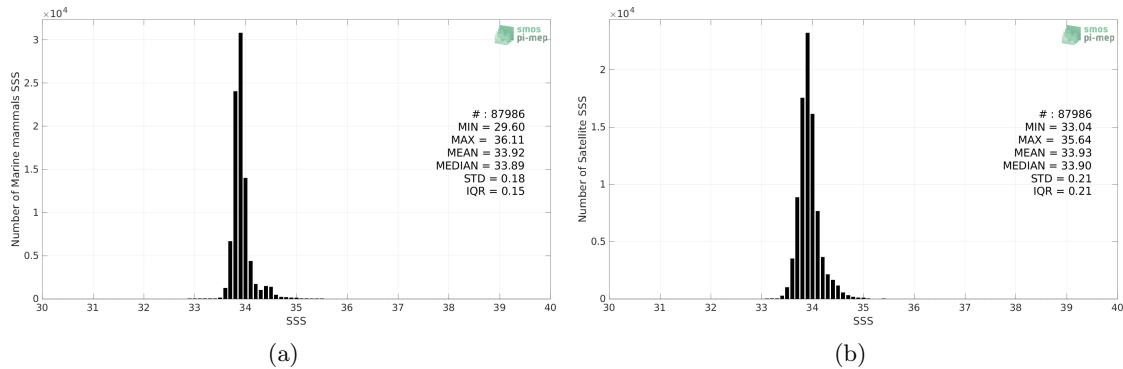
Figure 2: Histograms of SSS from Marine mammals (a) and SMOS SSS L3 v8 - 18 Days (CATDS-CECOS-LOCEAN) (b) considering all match-up pairs per bins of 0.1 over the Roaring Forties and Furious Fifties Pi-MEP region and for the full satellite product period.
