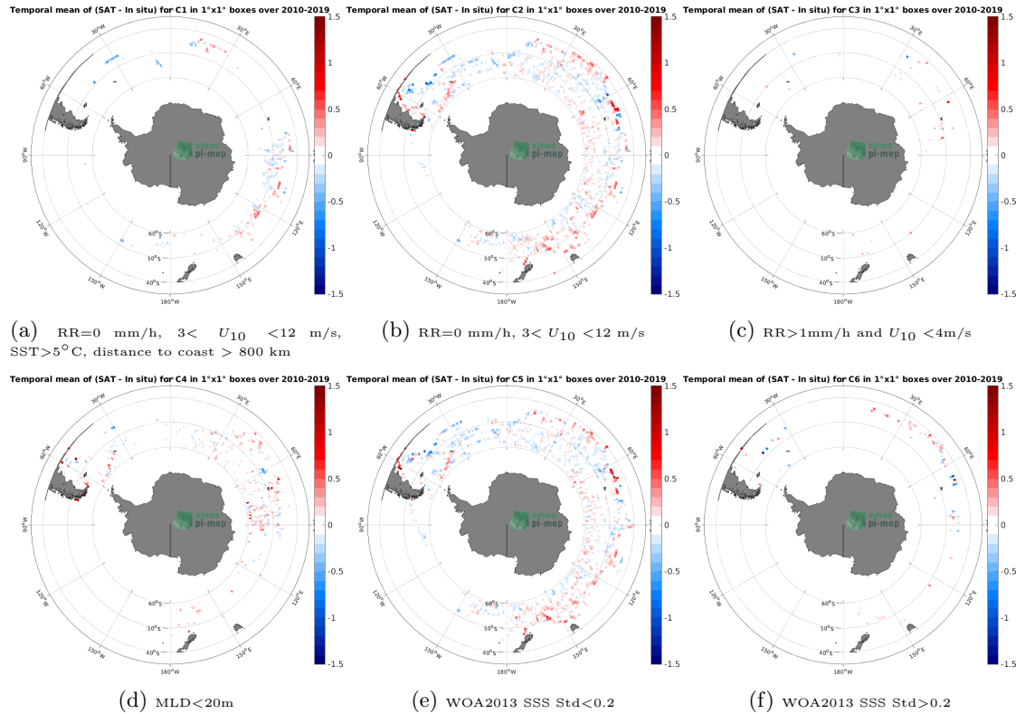
Figure 12: Temporal mean gridded over spatial boxes of size 1^{\circ}\times 1^{\circ} of \Delta\text{SSS} (SMOS SSS L3 v8 - 18 Days (CATDS-CECOS-LOCEAN) - Marine mammals) for 6 different subdatasets corresponding to:RR=0 mm/h, 3 < U_{10} < 12 m/s, SST >5^{\circ}\text{C} , distance to coast > 800 km (a), RR=0 mm/h, 3 < U_{10} < 12 m/s (b), RR >1 mm/h and U_{10} < 4 m/s (c),MLD <20 m (d),WOA2013 SSS Std <0.2 (e),WOA2013 SSS Std >0.2 (f).
