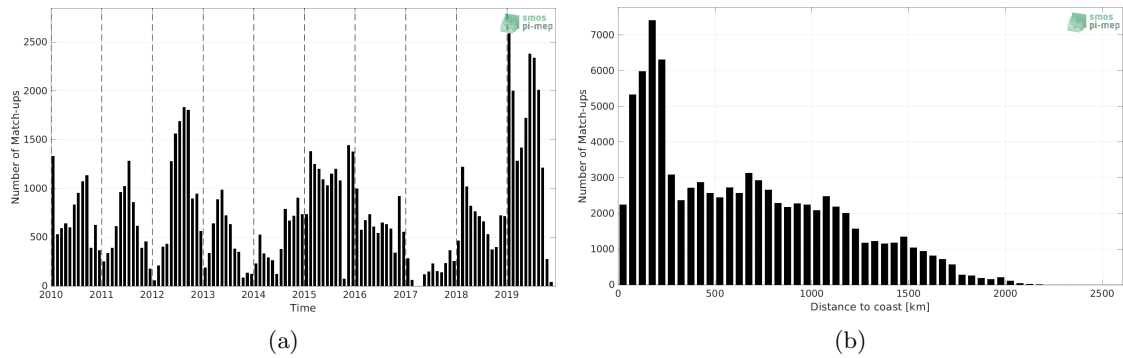
Figure 1: Number of match-ups between Marine mammals and SMOS SSS L3 v8 - 18 Days (CATDS-CECOS-LOCEAN) SSS as a function of time (a) and as function of the distance to coast (b) over the Roaring Forties and Furious Fifties Pi-MEP region and for the full satellite product period.
