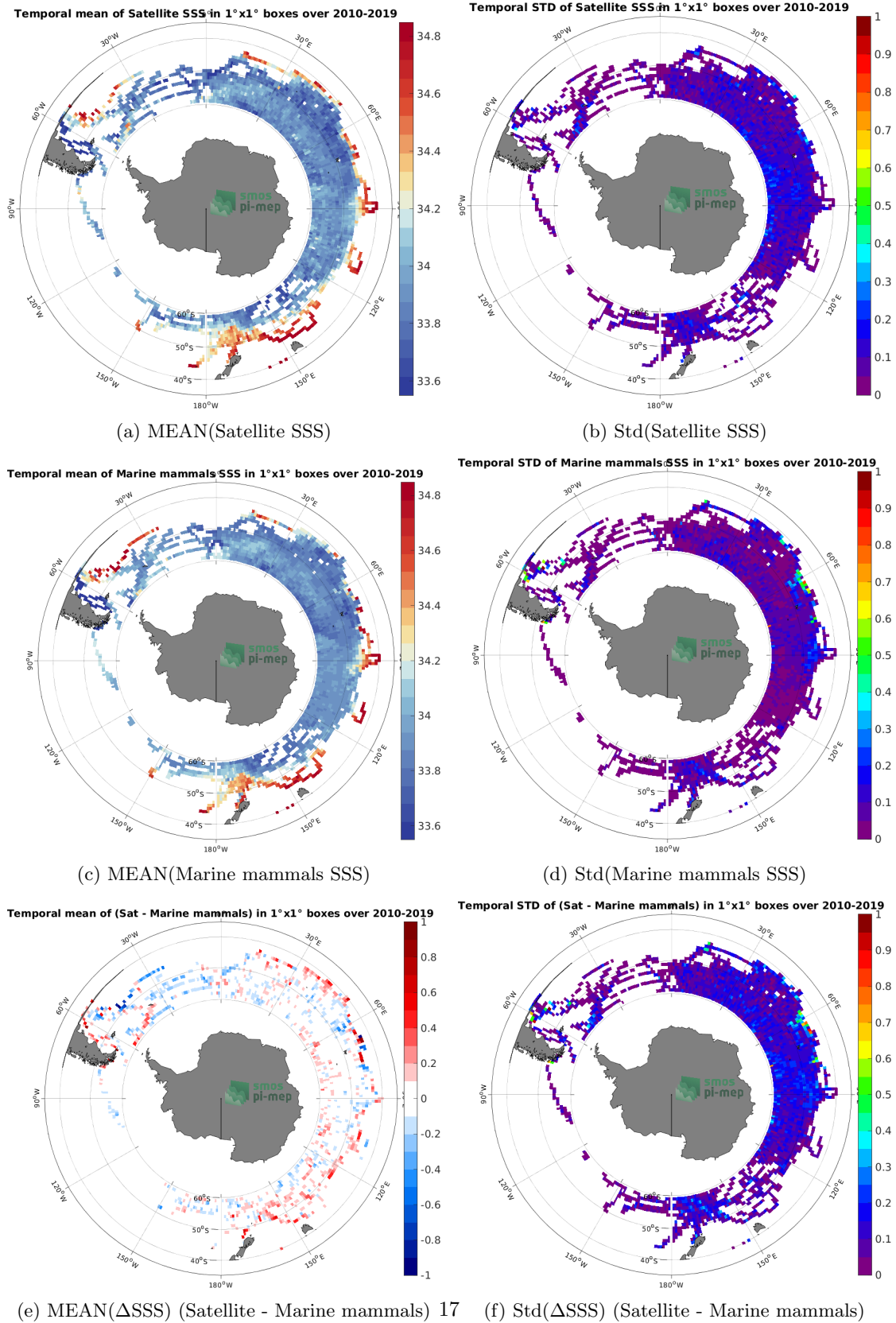
Figure 6: Temporal mean (left) and Std (right) of SSS from SMOS SSS L3 v8 - 18 Days (CATDS-CECOS-LOCEAN) (top), Marine mammals (middle), and of \Delta SSS (Satellite - Marine mammals). Only match-up pairs are used to generate these maps.
