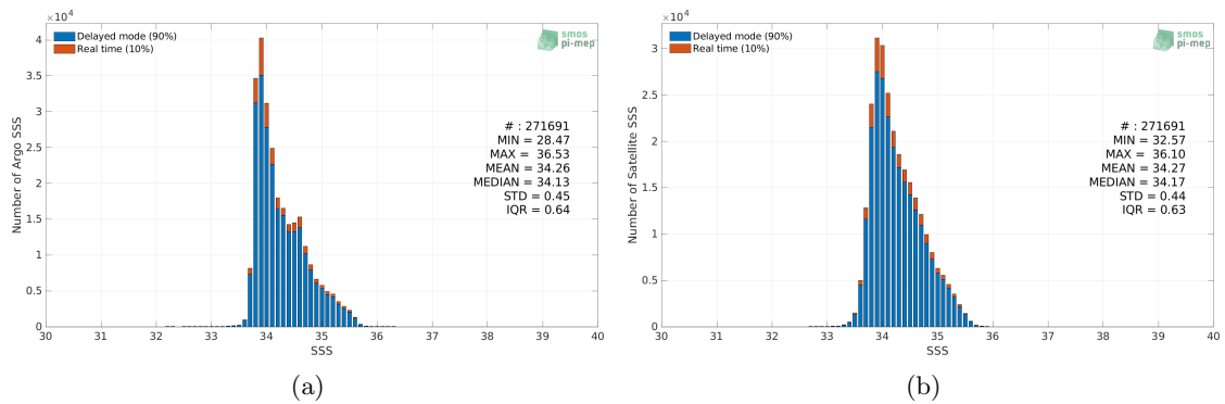
Figure 2: Histograms of SSS from Argo (a) and SMOS SSS L3 v8 - 18 Days (CATDS-CECOS-LOCEAN) (b) considering all match-up pairs per bins of 0.1 over the Roaring Forties and Furious Fifties Pi-MEP region and for the full satellite product period.
