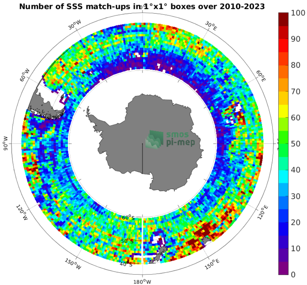
Figure 4: Number of SSS match-ups between Argo SSS and the SMOS SSS L3 v8 - 18 Days (CATDS-CECOS-LOCEAN) SSS product for the Roaring Forties and Furious Fifties Pi-MEP region over 1^\circ \times 1^\circ boxes and for the full satellite product period.
