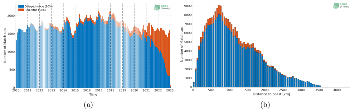
Figure 1: Number of match-ups between Argo and SMOS SSS L3 v8 - 18 Days (CATDS-CECOS-LOCEAN) SSS as a function of time (a) and as function of the distance to coast (b) over the Roaring Forties and Furious Fifties Pi-MEP region and for the full satellite product period.
