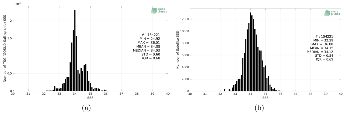
Figure 2: Histograms of SSS from TSG (GOSUD-Sailing-ship) (a) and SMOS SSS L3 v7 - 9 Days (CATDS-CECOS-LOCEAN) (b) considering all match-up pairs per bins of 0.1 over the Roaring Forties and Furious Fifties Pi-MEP region and for the full satellite product period.
