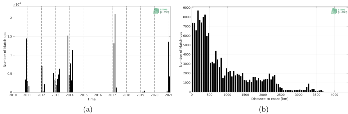
Figure 1: Number of match-ups between TSG (GOSUD-Sailing-ship) and SMOS SSS L3 v7 - 9 Days (CATDS-CECOS-LOCEAN) SSS as a function of time (a) and as function of the distance to coast (b) over the Roaring Forties and Furious Fifties Pi-MEP region and for the full satellite product period.
