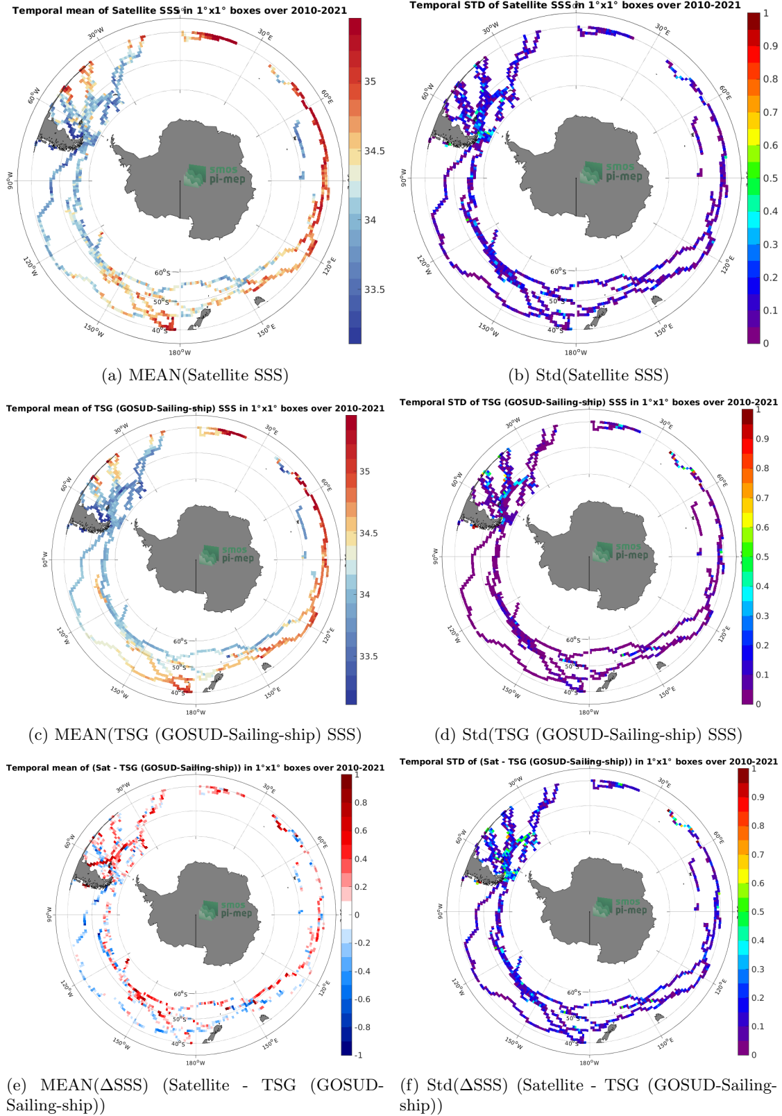
Figure 6: Temporal mean (left) and Std (right), of SSS from SMOS SSS L3 v7 - 9 Days (CATDS-CECOS-LOCEAN) (top), TSG (GOSUD-Sailing-ship) (middle), and of \Delta SSS (Satellite - TSG (GOSUD-Sailing-ship)). Only match-up pairs are used to generate these maps.
