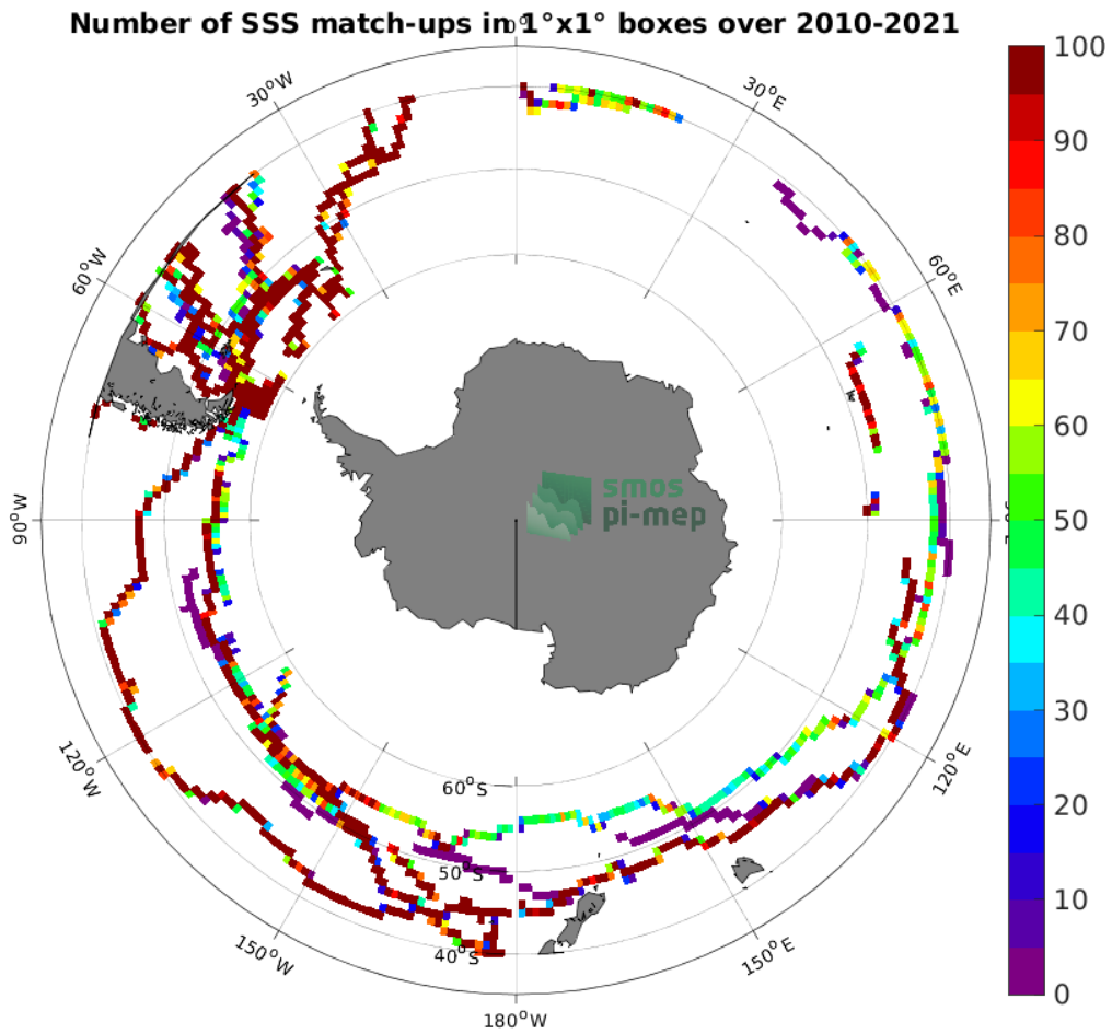
Figure 4: Number of SSS match-ups between TSG (GOSUD-Sailing-ship) SSS and the SMOS SSS L3 v7 - 9 Days (CATDS-CECOS-LOCEAN) SSS product for the Roaring Forties and Furious Fifties Pi-MEP region over 1^\circ \times 1^\circ boxes and for the full satellite product period.
