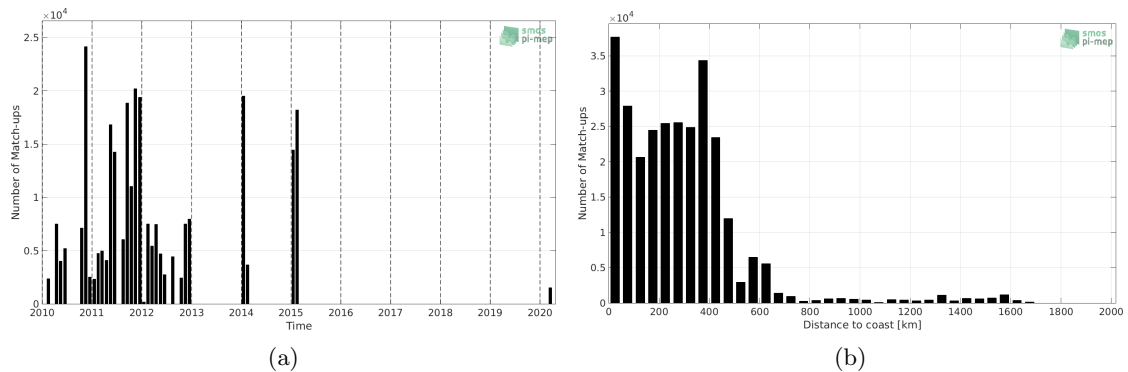
Figure 1: Number of match-ups between TSG (SAMOS) and SMOS SSS L3 v7 - 18 Days (CATDS-CECOS-LOCEAN) SSS as a function of time (a) and as function of the distance to coast (b) over the Roaring Forties and Furious Fifties Pi-MEP region and for the full satellite product period.
