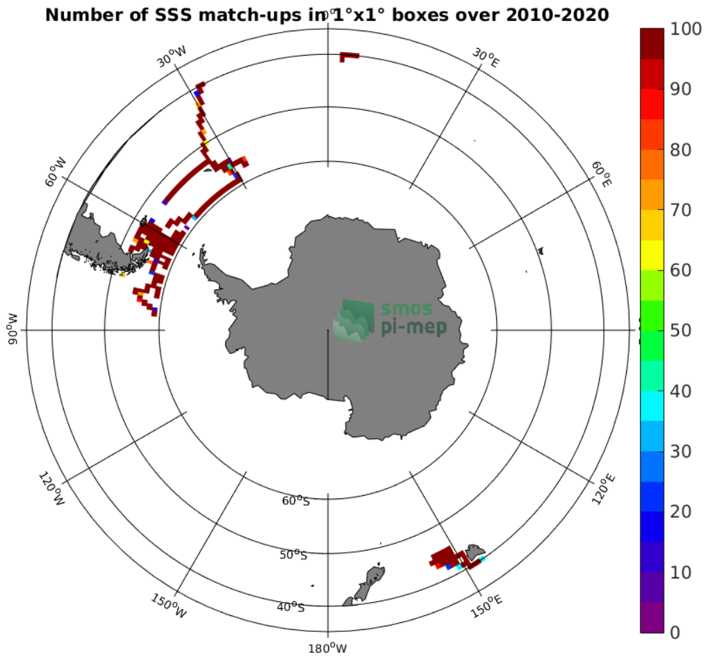
Figure 4: Number of SSS match-ups between TSG (SAMOS) SSS and the SMOS SSS L3 v7 - 18 Days (CATDS-CECOS-LOCEAN) SSS product for the Roaring Forties and Furious Fifties Pi-MEP region over 1^\circ \times 1^\circ boxes and for the full satellite product period.
