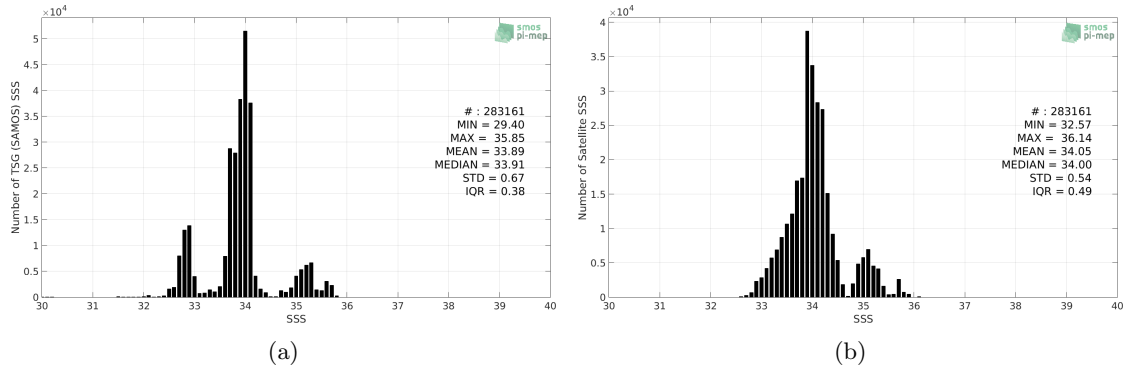
Figure 2: Histograms of SSS from TSG (SAMOS) (a) and SMOS SSS L3 v7 - 18 Days (CATDS-CECOS-LOCEAN) (b) considering all match-up pairs per bins of 0.1 over the Roaring Forties and Furious Fifties Pi-MEP region and for the full satellite product period.
