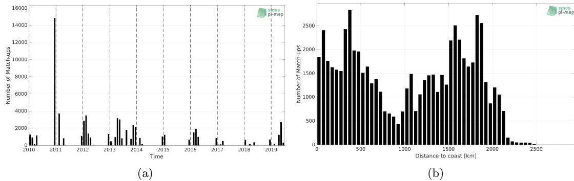
Figure 1: Number of match-ups between TSG (Polarstern) and SMOS SSS L3 v7 - 18 Days (CATDS-CECOS-LOCEAN) SSS as a function of time (a) and as function of the distance to coast (b) over the Roaring Forties and Furious Fifties Pi-MEP region and for the full satellite product period.
