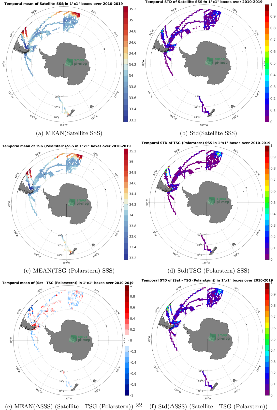
Figure 6: Temporal mean (left) and Std (right) of SSS from SMOS SSS L3 v7 - 18 Days (CATDS-CECOS-LOCEAN) (top), TSG (Polarstern) (middle), and of \Delta SSS (Satellite - TSG (Polarstern)). Only match-up pairs are used to generate these maps.
