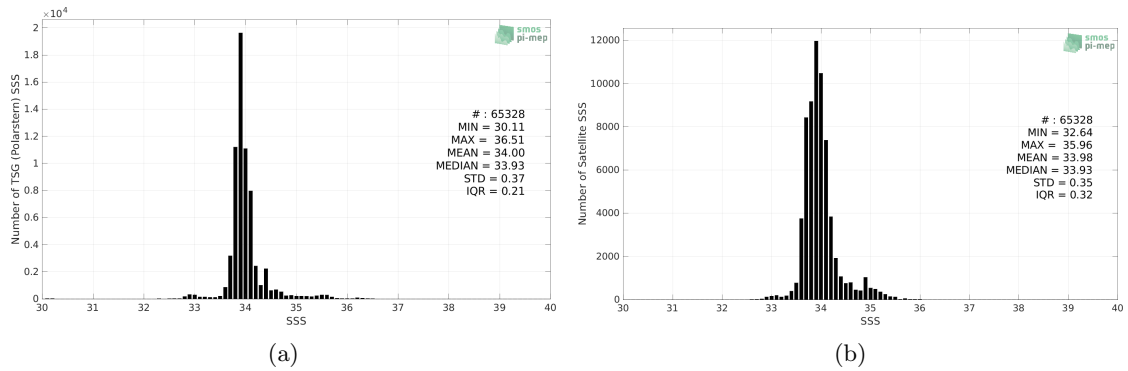
Figure 2: Histograms of SSS from TSG (Polarstern) (a) and SMOS SSS L3 v7 - 18 Days (CATDS-CECOS-LOCEAN) (b) considering all match-up pairs per bins of 0.1 over the Roaring Forties and Furious Fifties Pi-MEP region and for the full satellite product period.
