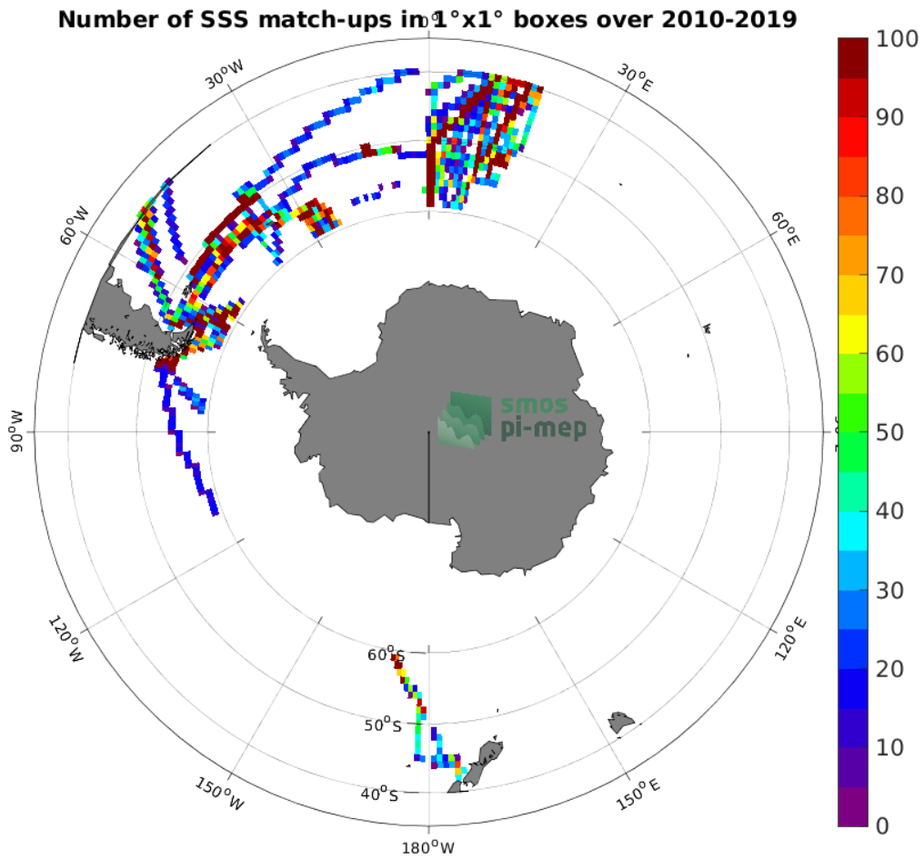
Figure 4: Number of SSS match-ups between TSG (Polarstern) SSS and the SMOS SSS L3 v7 - 18 Days (CATDS-CECOS-LOCEAN) SSS product for the Roaring Forties and Furious Fifties Pi-MEP region over 1^\circ \times 1^\circ boxes and for the full satellite product period.
