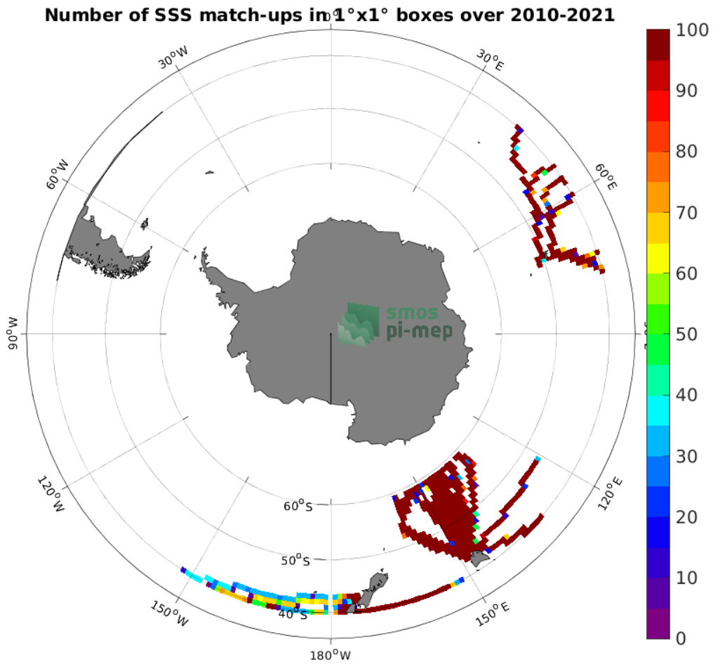
Figure 4: Number of SSS match-ups between TSG (LEGOS-DM) SSS and the SMOS SSS L3 v7 - 18 Days (CATDS-CECOS-LOCEAN) SSS product for the Roaring Forties and Furious Fifties Pi-MEP region over 1^\circ \times 1^\circ boxes and for the full satellite product period.
