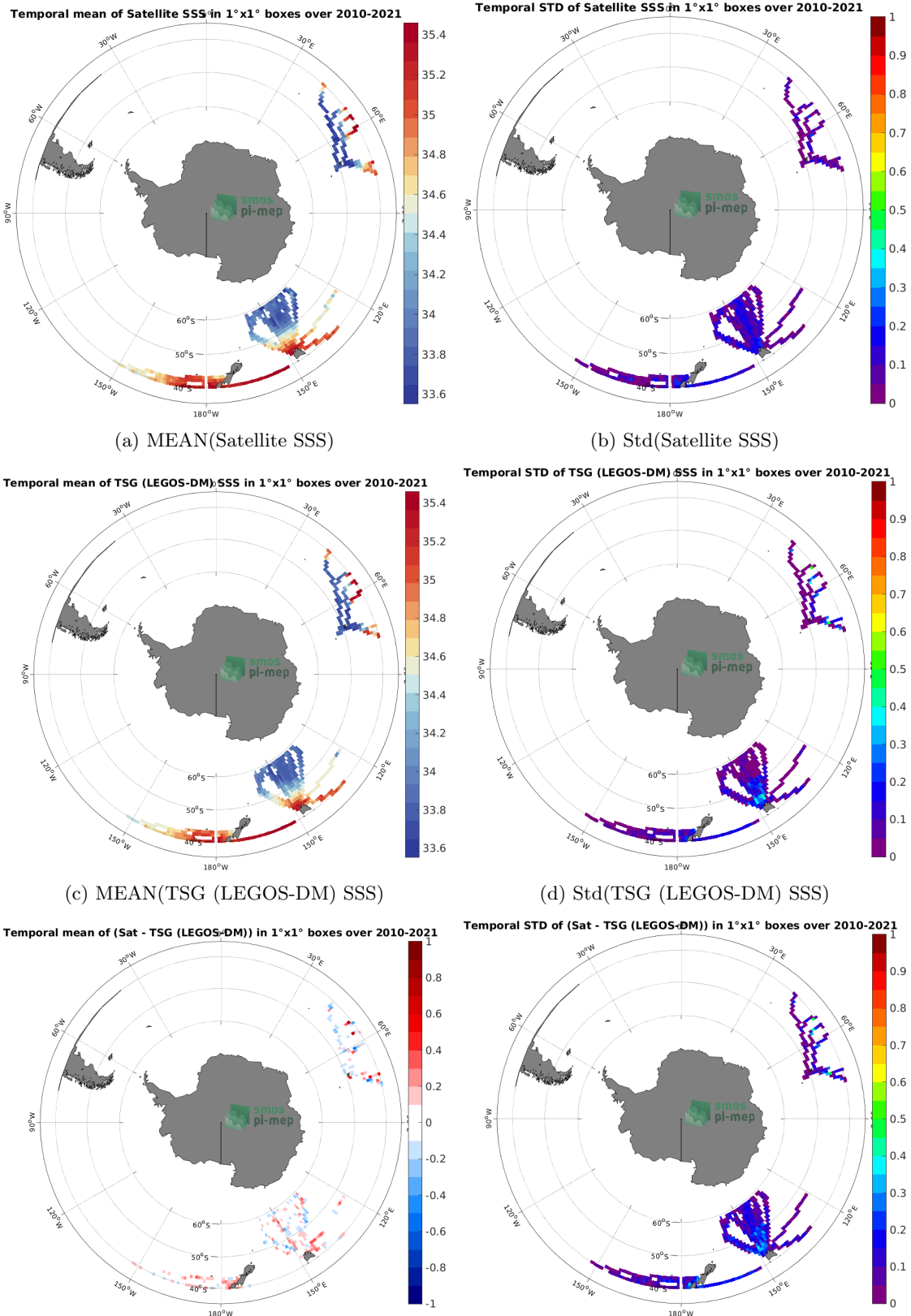
Figure 6: Temporal mean (left) and Std (right) of SSS from SMOS SSS L3 v7 - 18 Days (CATDS-CECOS-LOCEAN) (top), TSG (LEGOS-DM) (middle), and of \Delta SSS (Satellite - TSG (LEGOS-DM)). Only match-up pairs are used to generate these maps.
