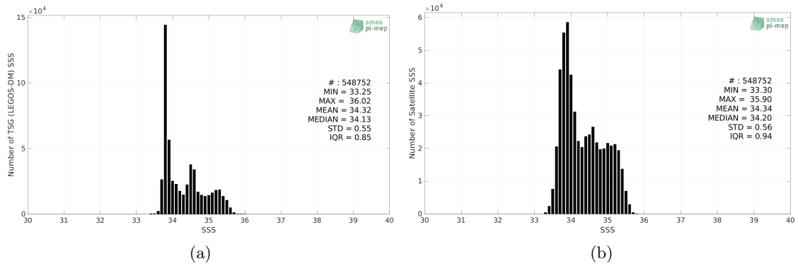
Figure 2: Histograms of SSS from TSG (LEGOS-DM) (a) and SMOS SSS L3 v7 - 18 Days (CATDS-CECOS-LOCEAN) (b) considering all match-up pairs per bins of 0.1 over the Roaring Forties and Furious Fifties Pi-MEP region and for the full satellite product period.
