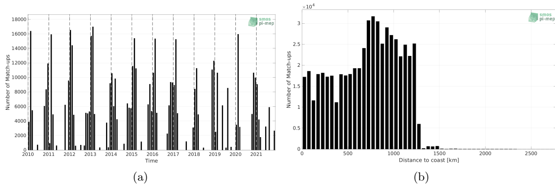
Figure 1: Number of match-ups between TSG (LEGOS-DM) and SMOS SSS L3 v7 - 18 Days (CATDS-CECOS-LOCEAN) SSS as a function of time (a) and as function of the distance to coast (b) over the Roaring Forties and Furious Fifties Pi-MEP region and for the full satellite product period.
