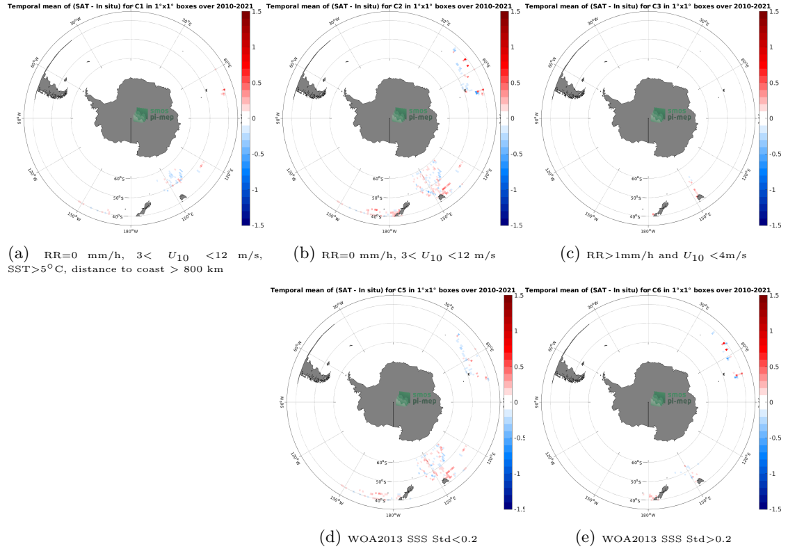
Figure 12: Temporal mean gridded over spatial boxes of size 1^{\circ}\times 1^{\circ} of \Delta\text{SSS} (SMOS SSS L3 v7 - 18 Days (CATDS-CECOS-LOCEAN) - TSG (LEGOS-DM)) for 5 different subdatasets corresponding to:RR=0 mm/h, 3 < U_{10} < 12 m/s, SST >5^{\circ}\text{C} , distance to coast > 800 km (a), RR=0 mm/h, 3 < U_{10} < 12 m/s (b), RR >1 mm/h and U_{10} < 4 m/s (c), WOA2013 SSS Std <0.2 (d), WOA2013 SSS Std >0.2 (e).
