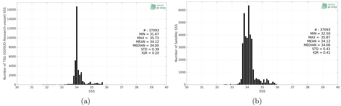
Figure 2: Histograms of SSS from TSG (GOSUD-Research-vessel) (a) and SMOS SSS L3 v7 - 18 Days (CATDS-CECOS-LOCEAN) (b) considering all match-up pairs per bins of 0.1 over the Roaring Forties and Furious Fifties Pi-MEP region and for the full satellite product period.
