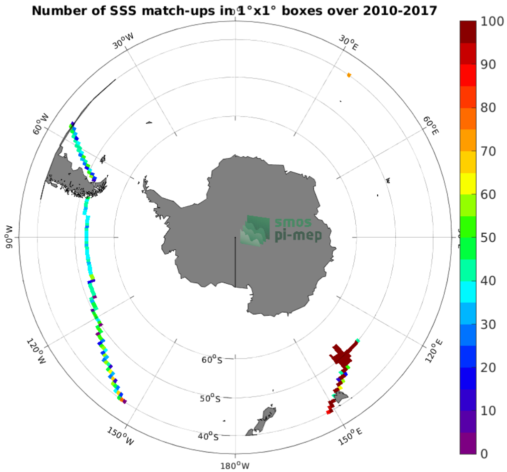
Figure 4: Number of SSS match-ups between TSG (GOSUD-Research-vessel) SSS and the SMOS SSS L3 v7 - 18 Days (CATDS-CECOS-LOCEAN) SSS product for the Roaring Forties and Furious Fifties Pi-MEP region over 1^\circ \times 1^\circ boxes and for the full satellite product period.
