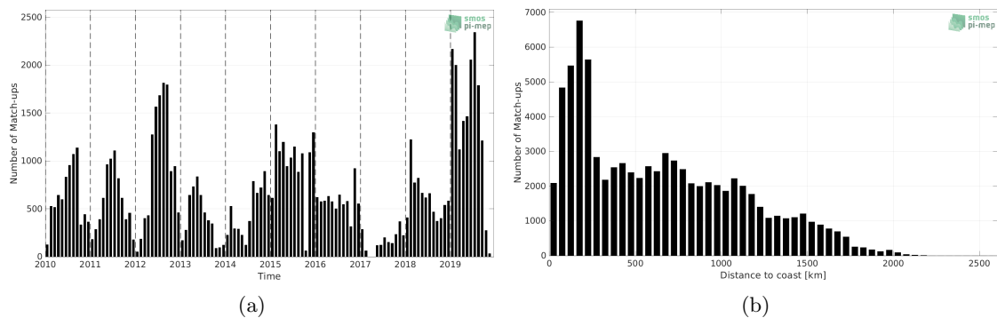
Figure 1: Number of match-ups between Marine mammals and SMOS SSS L3 v7 - 18 Days (CATDS-CECOS-LOCEAN) SSS as a function of time (a) and as function of the distance to coast (b) over the Roaring Forties and Furious Fifties Pi-MEP region and for the full satellite product period.
