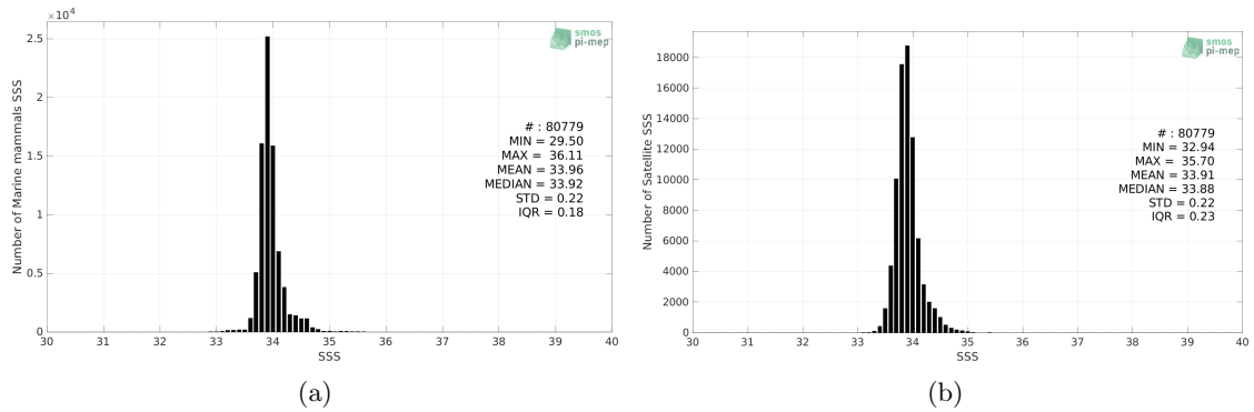
Figure 2: Histograms of SSS from Marine mammals (a) and SMOS SSS L3 v7 - 18 Days (CATDS-CECOS-LOCEAN) (b) considering all match-up pairs per bins of 0.1 over the Roaring Forties and Furious Fifties Pi-MEP region and for the full satellite product period.
