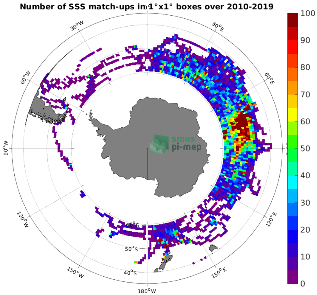
Figure 4: Number of SSS match-ups between Marine mammals SSS and the SMOS SSS L3 v7 - 18 Days (CATDS-CECOS-LOCEAN) SSS product for the Roaring Forties and Furious Fifties Pi-MEP region over 1^\circ \times 1^\circ boxes and for the full satellite product period.
