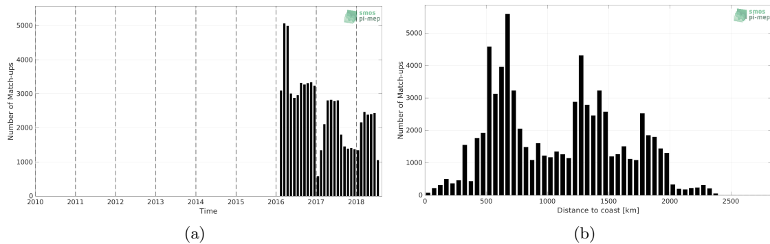
Figure 1: Number of match-ups between Surface drifters and SMOS SSS L3 v7 - 18 Days (CATDS-CECOS-LOCEAN) SSS as a function of time (a) and as function of the distance to coast (b) over the Roaring Forties and Furious Fifties Pi-MEP region and for the full satellite product period.
