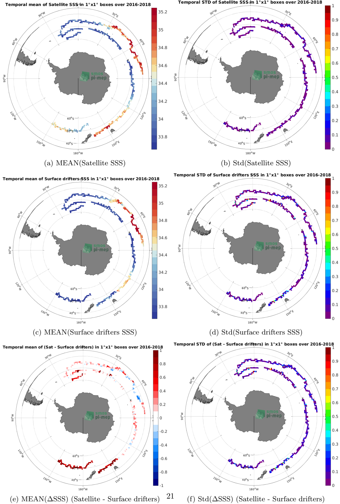
Figure 5: Temporal mean (left) and Std (right) of SSS from SMOS SSS L3 v7 - 18 Days (CATDS-CECOS-LOCEAN) (top), Surface drifters (middle), and of \Delta SSS (Satellite - Surface drifters). Only match-up pairs are used to generate these maps.
