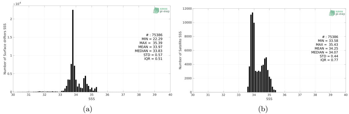
Figure 2: Histograms of SSS from Surface drifters (a) and SMOS SSS L3 v7 - 18 Days (CATDS-CECOS-LOCEAN) (b) considering all match-up pairs per bins of 0.1 over the Roaring Forties and Furious Fifties Pi-MEP region and for the full satellite product period.
