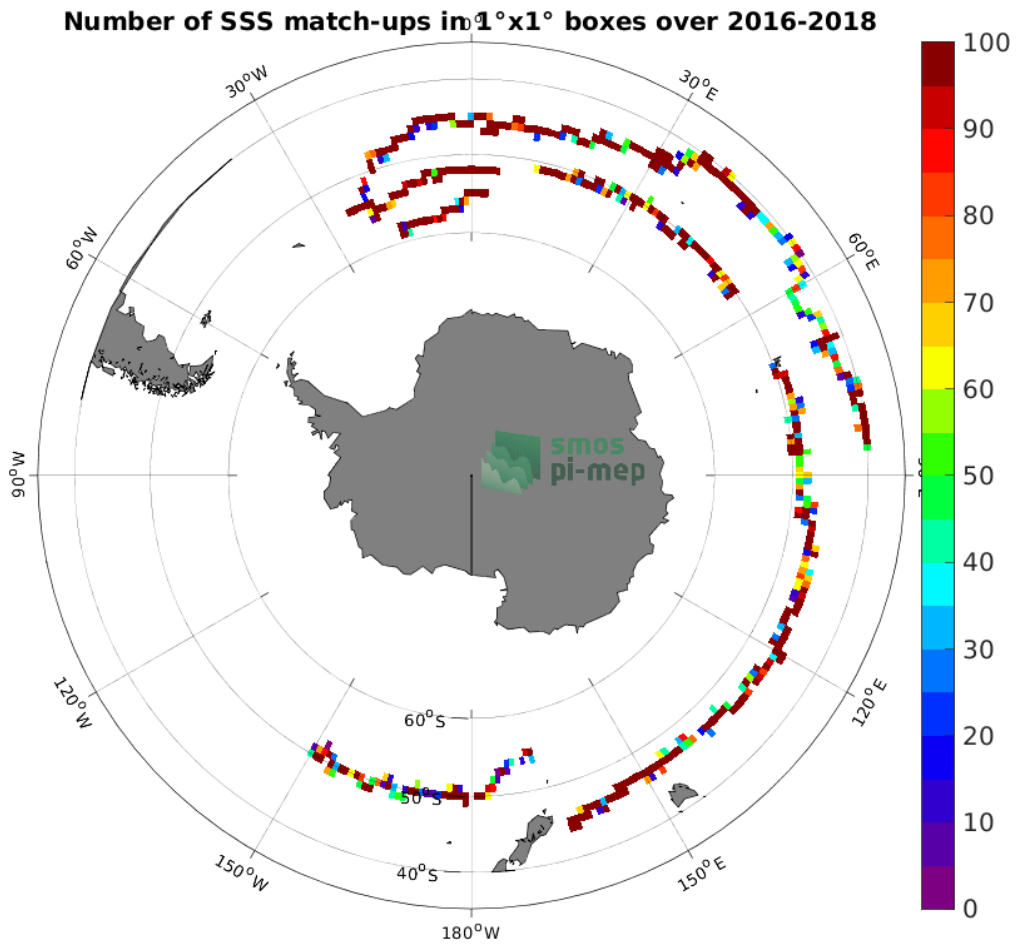
Figure 3: Number of SSS match-ups between Surface drifters SSS and the SMOS SSS L3 v7 - 18 Days (CATDS-CECOS-LOCEAN) SSS product for the Roaring Forties and Furious Fifties Pi-MEP region over 1^\circ \times 1^\circ boxes and for the full satellite product period.
