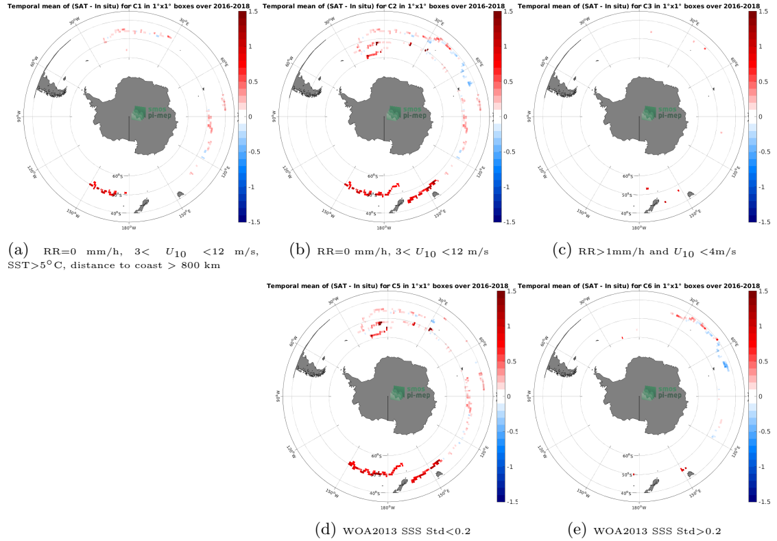
Figure 11: Temporal mean gridded over spatial boxes of size 1^{\circ}\times 1^{\circ} of \Delta\text{SSS} (SMOS SSS L3 v7 - 18 Days (CATDS-CECOS-LOCEAN) - Surface drifters) for 5 different subdatasets corresponding to:RR=0 mm/h, 3 < U_{10} < 12 m/s, SST >5^{\circ}\text{C} , distance to coast > 800 km (a), RR=0 mm/h, 3 < U_{10} < 12 m/s (b), RR >1 mm/h and U_{10} < 4 m/s (c), WOA2013 SSS Std <0.2 (d), WOA2013 SSS Std >0.2 (e).
