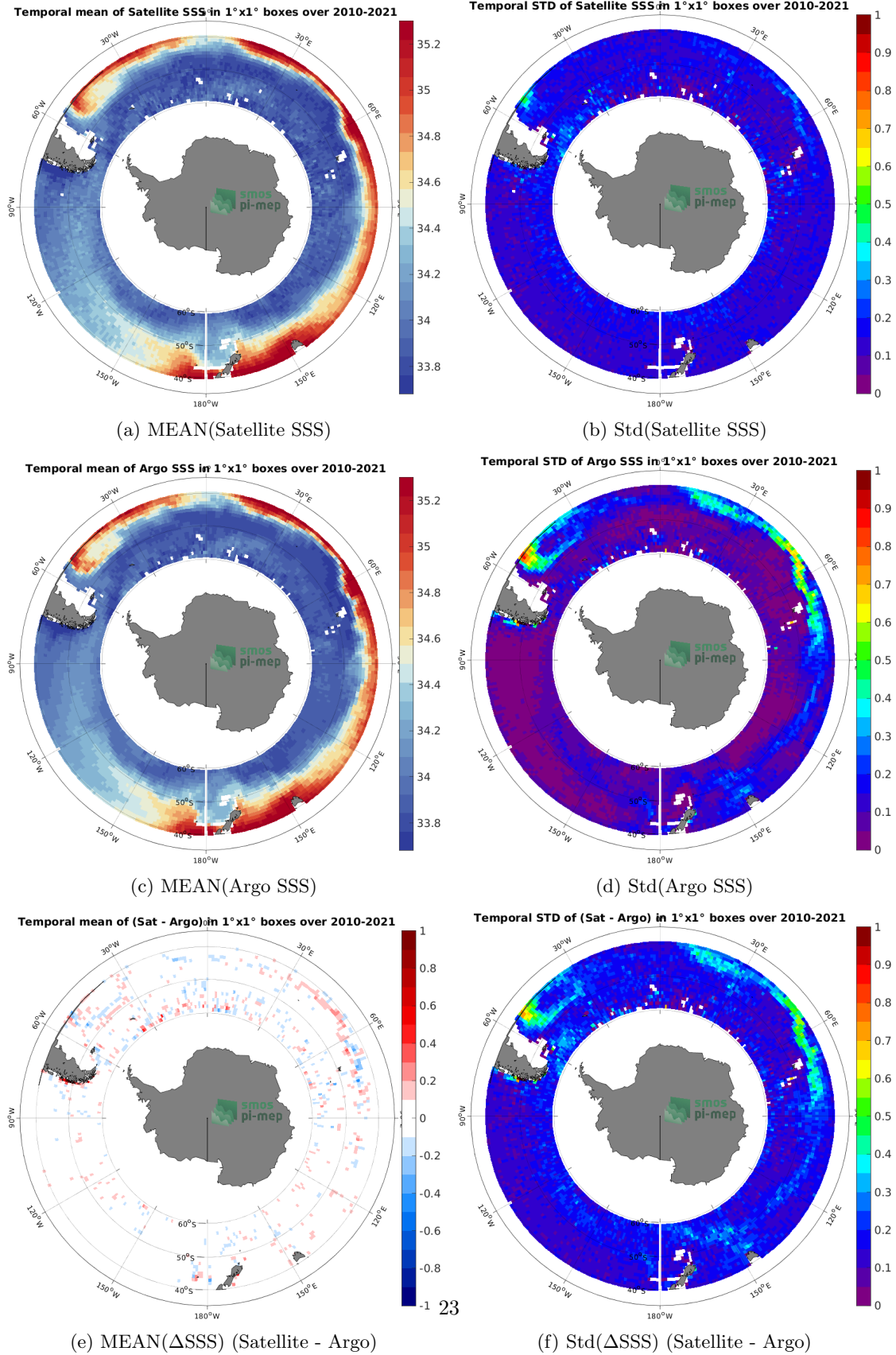
Figure 6: Temporal mean (left) and Std (right) of SSS from SMOS SSS L3 v7 - 18 Days (CATDS-CECOS-LOCEAN) (top), Argo (middle), and of \Delta SSS (Satellite - Argo). Only match-up pairs are used to generate these maps.
