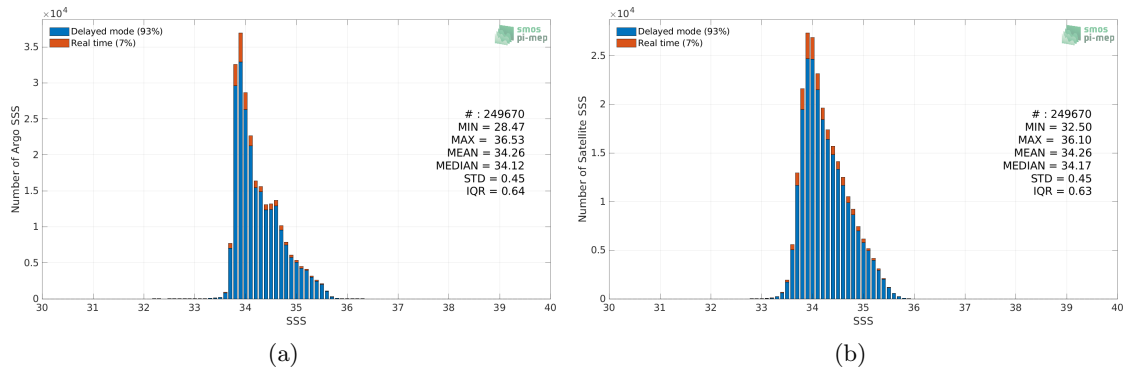
Figure 2: Histograms of SSS from Argo (a) and SMOS SSS L3 v7 - 18 Days (CATDS-CECOS-LOCEAN) (b) considering all match-up pairs per bins of 0.1 over the Roaring Forties and Furious Fifties Pi-MEP region and for the full satellite product period.
