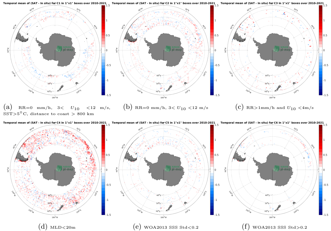
Figure 12: Temporal mean gridded over spatial boxes of size 1^{\circ}\times 1^{\circ} of \Delta\text{SSS} (SMOS SSS L3 v7 - 18 Days (CATDS-CECOS-LOCEAN) - Argo) for 6 different subdatasets corresponding to:RR=0 mm/h, 3 < U_{10} < 12 m/s, SST >5^{\circ}\text{C} , distance to coast > 800 km (a), RR=0 mm/h, 3 < U_{10} < 12 m/s (b), RR >1\text{mm/h} and U_{10} < 4\text{m/s} (c),MLD <20\text{m} (d),WOA2013 SSS Std <0.2 (e),WOA2013 SSS Std >0.2 (f).
