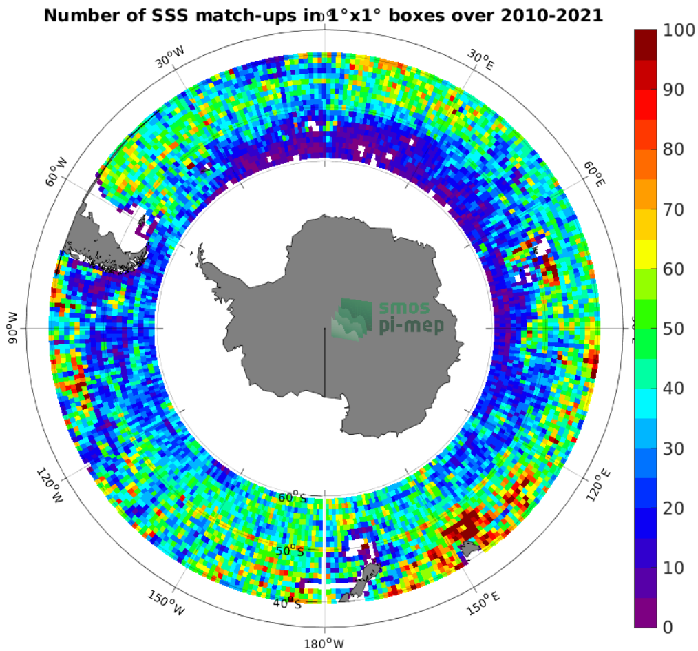
Figure 4: Number of SSS match-ups between Argo SSS and the SMOS SSS L3 v7 - 18 Days (CATDS-CECOS-LOCEAN) SSS product for the Roaring Forties and Furious Fifties Pi-MEP region over 1^\circ \times 1^\circ boxes and for the full satellite product period.
