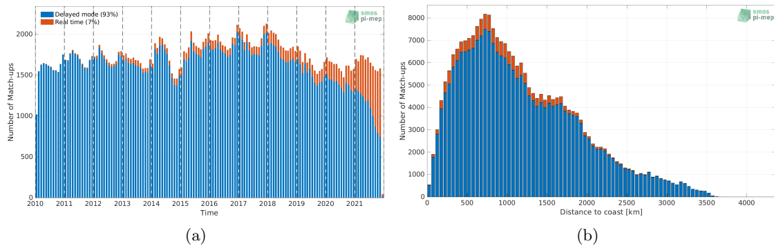
Figure 1: Number of match-ups between Argo and SMOS SSS L3 v7 - 18 Days (CATDS-CECOS-LOCEAN) SSS as a function of time (a) and as function of the distance to coast (b) over the Roaring Forties and Furious Fifties Pi-MEP region and for the full satellite product period.
