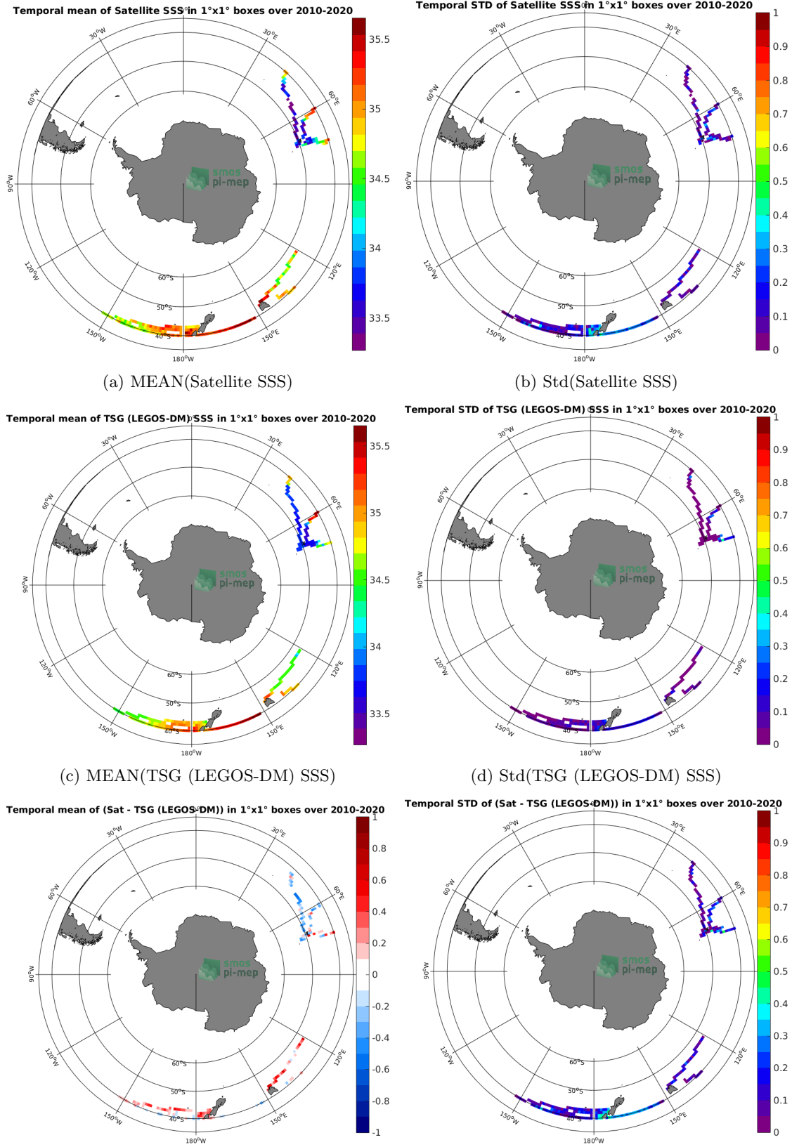
(a) MEAN(Satellite SSS) (b) Std(Satellite SSS) (c) MEAN(TSG (LEGOS-DM) SSS) (d) Std(TSG (LEGOS-DM) SSS) (e) MEAN( \Delta SSS) (Satellite - TSG (LEGOS-DM)) 22 (f) Std( \Delta SSS) (Satellite - TSG (LEGOS-DM)) Figure 6: Temporal mean (left) and Std (right) of SSS from SMOS SSS L3 v5 - 9 Days (CATDS-CECOS-LOCEAN) (top), TSG (LEGOS-DM) (middle), and of \Delta SSS (Satellite - TSG (LEGOS-DM)). Only match-up pairs are used to generate these maps.
