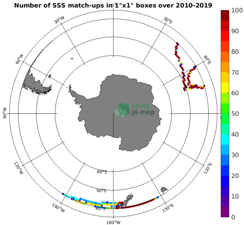
Figure 4: Number of SSS match-ups between TSG (LEGOS-DM) SSS and the SMOS SSS L3 v5 - 9 Days (CATDS-CECOS-LOCEAN) SSS product for the Roaring Forties and Furious Fifties Pi-MEP region over 1^\circ \times 1^\circ boxes and for the full satellite product period.
