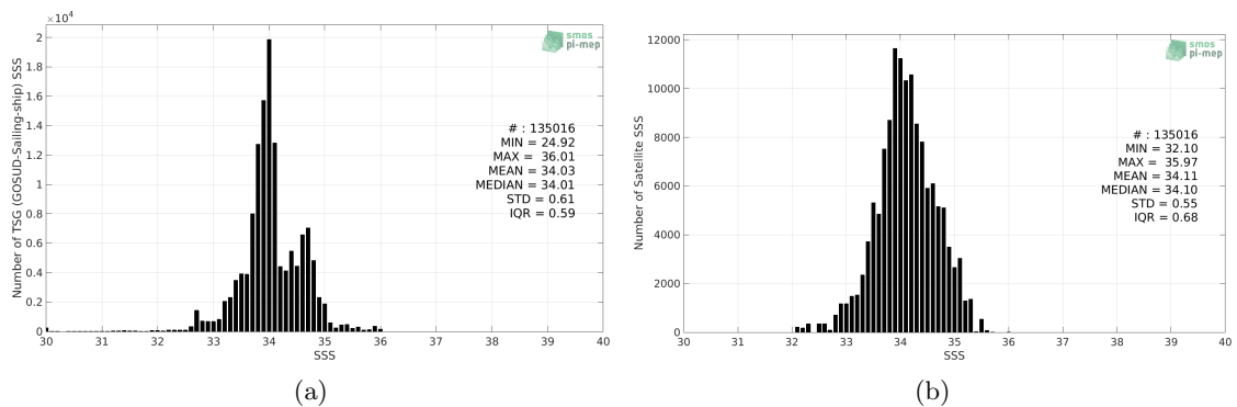
Figure 2: Histograms of SSS from TSG (GOSUD-Sailing-ship) (a) and SMOS SSS L3 v5 - 9 Days (CATDS-CECOS-LOCEAN) (b) considering all match-up pairs per bins of 0.1 over the Roaring Forties and Furious Fifties Pi-MEP region and for the full satellite product period.
