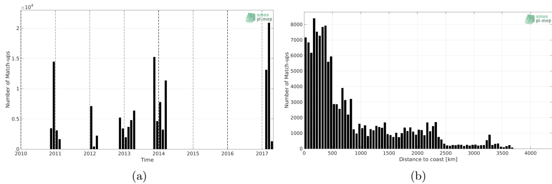
Figure 1: Number of match-ups between TSG (GOSUD-Sailing-ship) and SMOS SSS L3 v5 - 9 Days (CATDS-CECOS-LOCEAN) SSS as a function of time (a) and as function of the distance to coast (b) over the Roaring Forties and Furious Fifties Pi-MEP region and for the full satellite product period.
