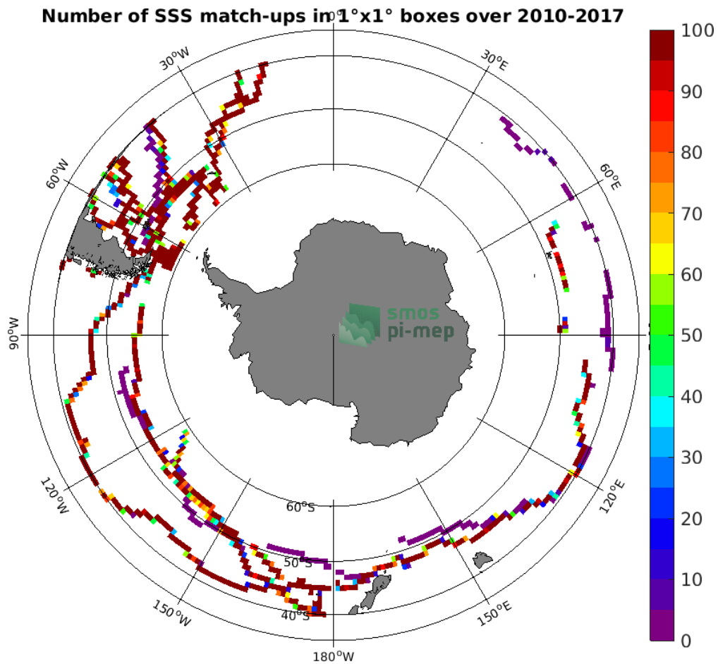
Figure 4: Number of SSS match-ups between TSG (GOSUD-Sailing-ship) SSS and the SMOS SSS L3 v5 - 9 Days (CATDS-CECOS-LOCEAN) SSS product for the Roaring Forties and Furious Fifties Pi-MEP region over 1^\circ \times 1^\circ boxes and for the full satellite product period.
