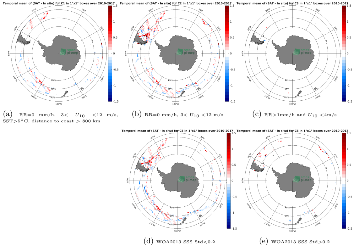
Figure 12: Temporal mean gridded over spatial boxes of size 1°x1° of \Delta SSS (SMOS SSS L3 v5 - 9 Days (CATDS-CECOS-LOCEAN) - TSG (GOSUD-Sailing-ship)) for 5 different subdatasets corresponding to:RR=0 mm/h, 3 < U_{10} < 12 m/s, SST>5°C, distance to coast > 800 km (a), RR=0 mm/h, 3 < U_{10} < 12 m/s (b), RR>1mm/h and U_{10} < 4 m/s (c), WOA2013 SSS Std<0.2 (d), WOA2013 SSS Std>0.2 (e).
