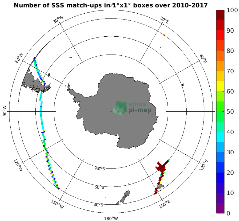
Figure 4: Number of SSS match-ups between TSG (GOSUD-Research-vessel) SSS and the SMOS SSS L3 v5 - 9 Days (CATDS-CECOS-LOCEAN) SSS product for the Roaring Forties and Furious Fifties Pi-MEP region over 1°x1° boxes and for the full satellite product period.
