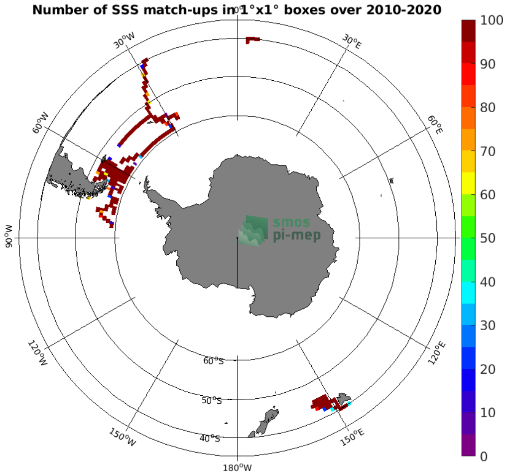
Figure 4: Number of SSS match-ups between TSG (SAMOS) SSS and the SMOS SSS L3 v5 - 18 Days (CATDS-CECOS-LOCEAN) SSS product for the Roaring Forties and Furious Fifties Pi-MEP region over 1^\circ \times 1^\circ boxes and for the full satellite product period.
