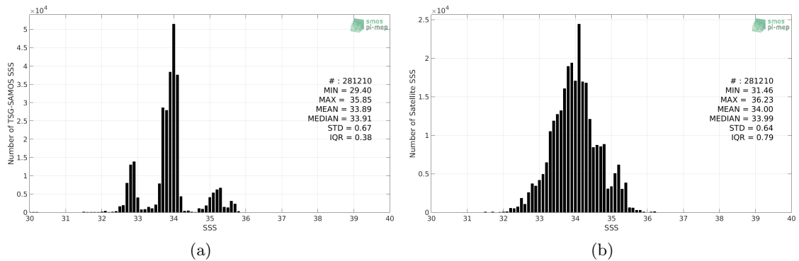
Figure 2: Histograms of SSS from TSG-SAMOS (a) and SMOS-L3-CATDS-CECOS-LOCEAN-V4-9DAYS-25KM (b) considering all match-up pairs per bins of 0.1 over the Roaring Forties and Furious Fifties Pi-MEP region and for the full satellite product period.
