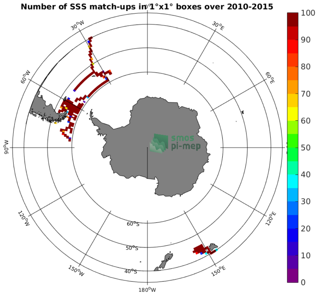
Figure 4: Number of SSS match-ups between TSG-SAMOS SSS and the SMOS-L3-CATDS-CECOS-LOCEAN-V4-9DAYS-25KM SSS product for the Roaring Forties and Furious Fifties Pi-MEP region over 1^\circ \times 1^\circ boxes and for the full satellite product period.
