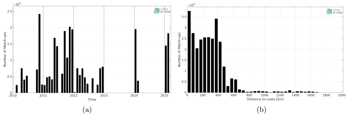
Figure 1: Number of match-ups between TSG-SAMOS and SMOS-L3-CATDS-CECOS-LOCEAN-V4-9DAYS-25KM SSS as a function of time (a) and as function of the distance to coast (b) over the Roaring Forties and Furious Fifties Pi-MEP region and for the full satellite product period.
